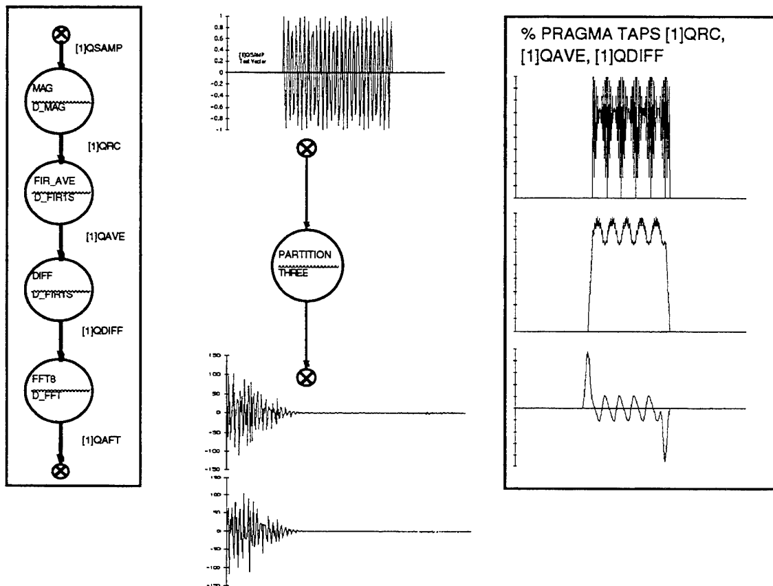
Figure 9 - GrTT Behavior Model Execution Input and output test vectors and internal queue content of the behavior model are shown
