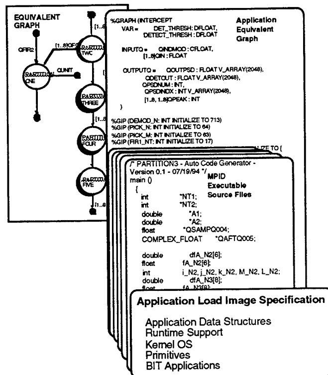
Figure 5. - Application Generator
