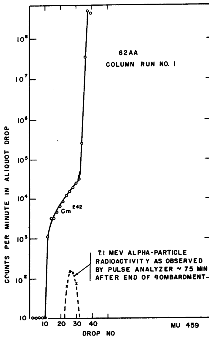
Fig. 3. Results of separation in first Dowex-50 resin column showing small amount of new 7.1-Mev alpha-radioactivity separated ahead of large amount of Cm 242 alpha-radioactivity.
