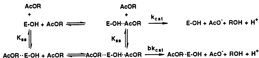
Scheme 4
