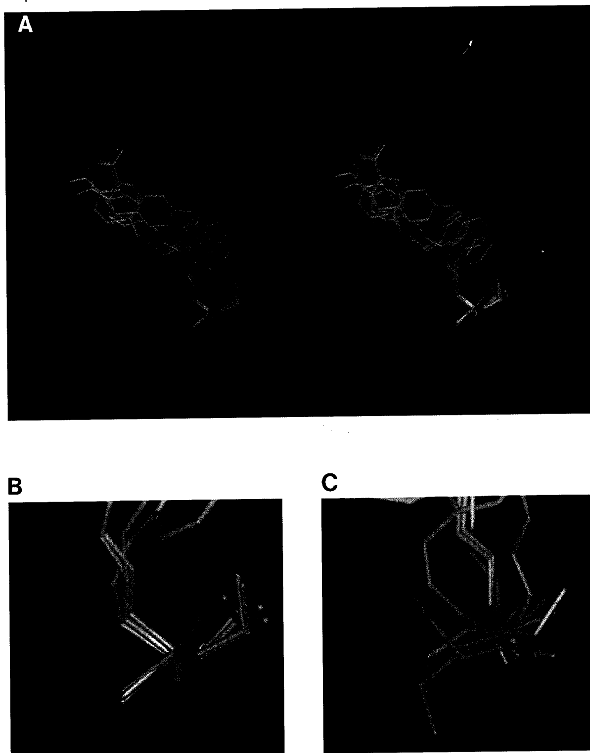
FIG. 7. Molecular dynamics of the pentacoordinate transition state between EMP R,S -AChE and HI-6. A stereoview of EMP R,S -AChE-HI6. Geometry around phosphorus was pentacoordinate with the oxime and Ser-203 oxygen assuming apical positions. Shown are the results of five simulations with heating and equilibrating at 700 K with subsequent cooling to 300 K. Simulations were constructed for R and S enantiomers of EMP. B shows an enlarged view in the region of the pentacoordinate phosphorus for the EMP R -AChE-HI-6 transition state. Note the fixed position of the phosphonyl oxygen. C shows an identical simulation for EMP S -AChE-HI-6 where a large variation of position of the residues around the phosphorus are noted.
