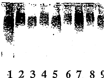
Fig. 4. Electrophoretic analysis of mAChE and fasciculin-mAChE complexes. A: SDS-PAGE (4–20% gradient gel, 8 cm \times 8 cm) under reducing conditions: lanes 2, 3, and 4, purified mAChE; lane 1, mAChE complexed to Fas1; lane 5, mAChE complexed to Fas2; lane 6, washed and dissolved Fas2-mAChE hexagonal crystal; mAChE migrates as two diffuse and overlapping bands; arrow at the bottom of the gel indicates the fasciculin band (lanes 1, 5, and 6). B: Native gel electrophoresis (7.5% resolving/5% stacking gel, 8 cm \times 8 cm) with migration toward the anode: lanes 1, 3, 5, and 9, purified mAChE; lane 2, mAChE complexed to Fas1; lane 4, mAChE complexed to Fas2; lanes 6, 7, and 8, washed and dissolved triangular, needle-shaped, and hexagonal Fas2-mAChE crystals, grown in (\text{NH}_4)_2\text{SO}_4 ; the shift toward the cathode in the position of the complexes (lanes 2, 4, 6, 7, and 8) relative to the free mAChE is evident.
