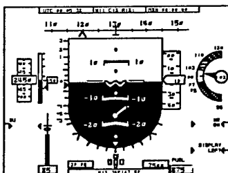
PRIMARY FLIGHT DISPLAY
