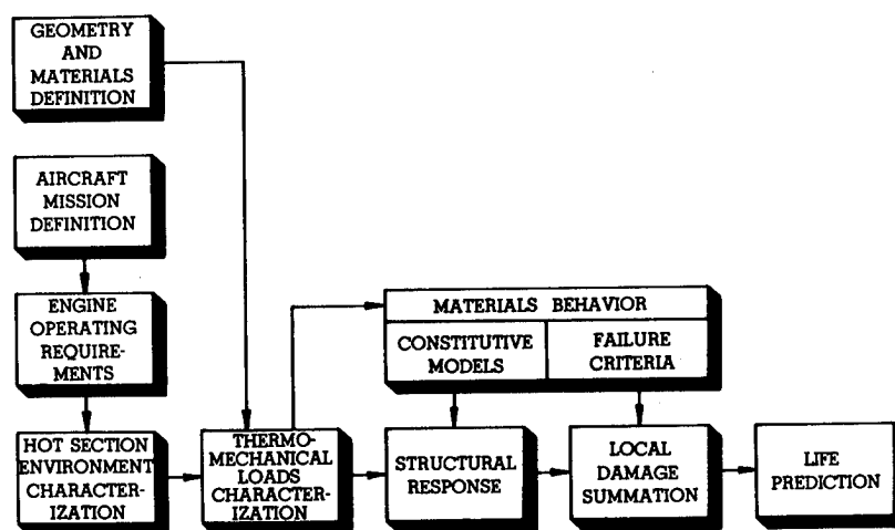
FIGURE 1. - INTEGRATION OF ANALYSES LEADS TO LIFE PREDICTION OF HOT SECTION PARTS.
