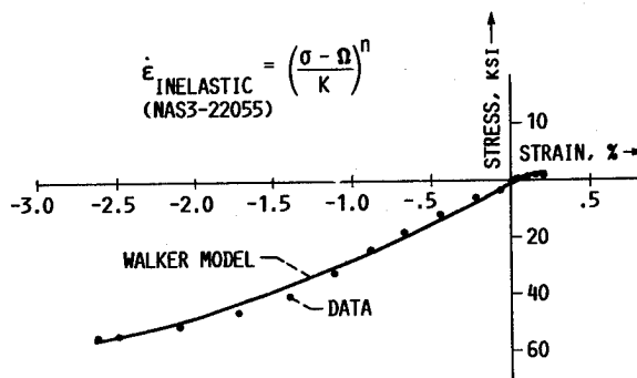
FIGURE 5. - CERAMIC BEHAVIOR MODELED WITH WALKER EQUATION ACCORDING TO THE PRATT & WHITNEY MODEL.
