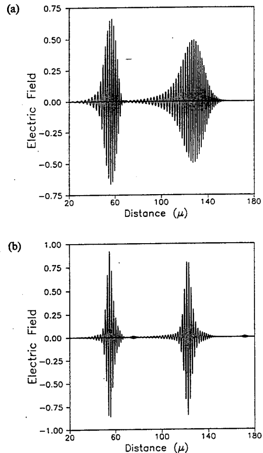
Fig. 7. FD-TD computed propagation of a 50 fs duration infrared optical pulse observed at propagation distances of 55 and 126 \mu m from the source in a medium having anomalous dispersion due to a single Lorentzian relaxation: (a) linear case, showing pulse attenuation, broadening, and frequency modulation; (b) dispersive non-linear case, showing the formation of a soliton pulse and precursor.
