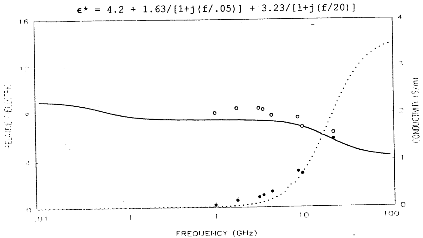
Figure 3. Permittivity of bone [16, 17].
