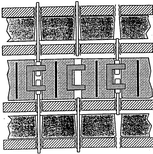
Fig. 4. Vertical cut through the four-board, three-connector geometry showing the via pins spaced 0.1 in apart.
