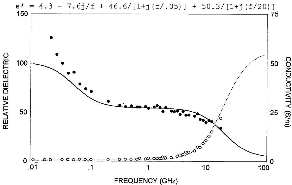
Figure 10. Permittivity of muscle tissue [16-19, 21-24].
