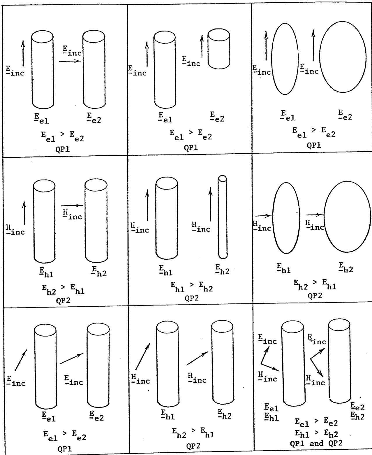
Fig. 10. (Fig. 72, third edition) Qualitative evaluation of the internal fields based on qualitative principle QP1 and QP2. E_e is the internal electric field generated by E_{inc} , the incident field, and E_h is the internal electric field generated by H_{inc} , the incident H field.
