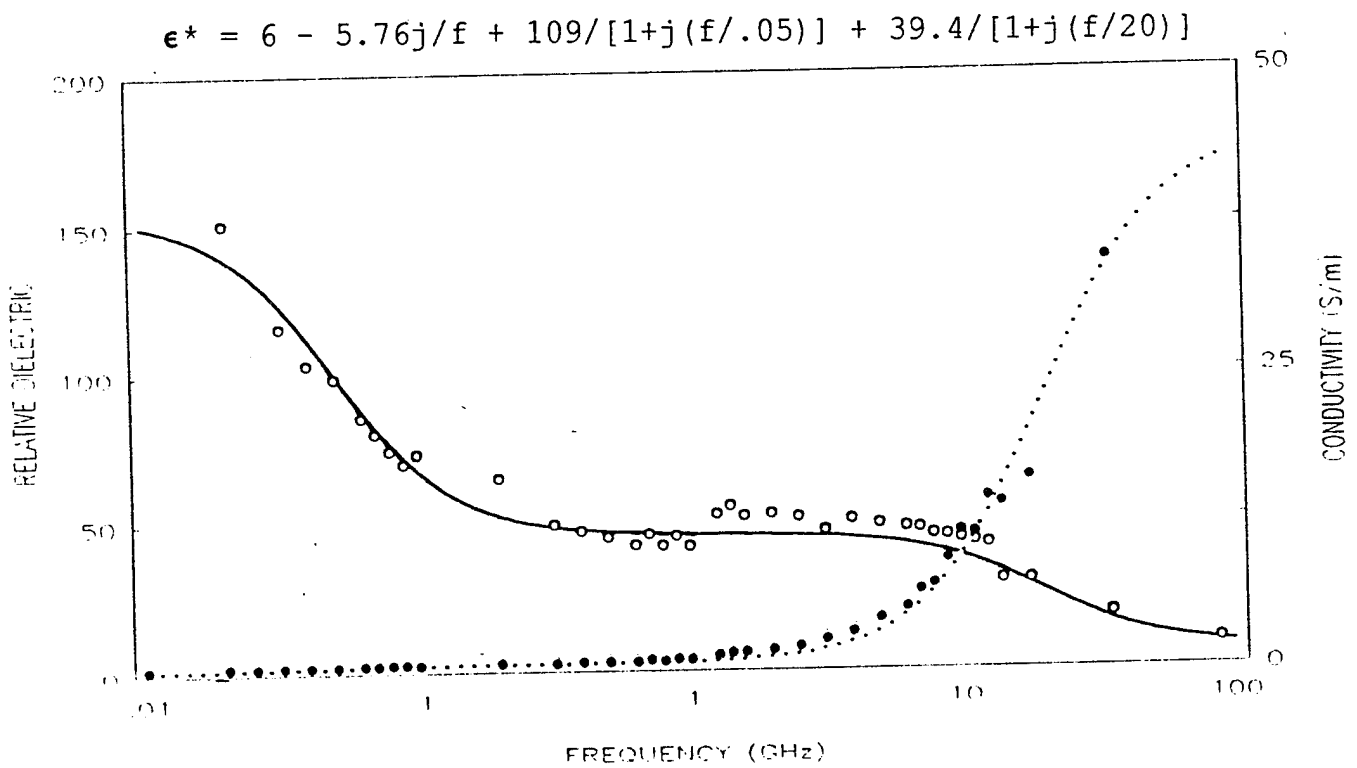
Figure 4. Permittivity of brain tissue [16-20, 23, 26].
