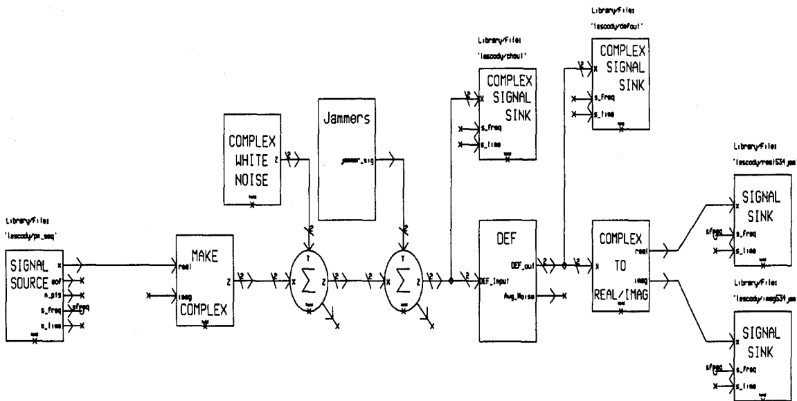
Figure 18. System Model for Measuring PAR
