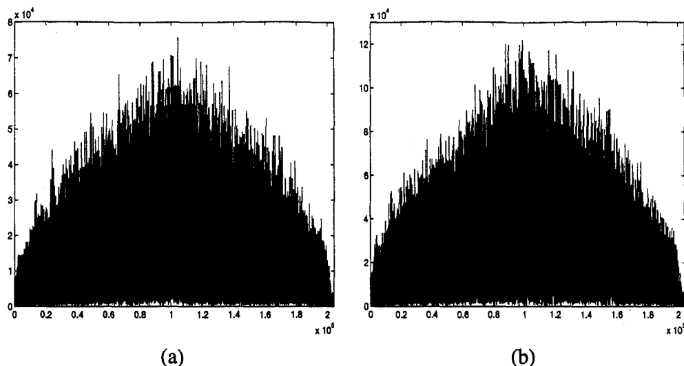
Figure 30. Cross Correlations For 4 Pulsed CW Jammer: (a) 53 dB J/N with 6 dB Threshold (b) 53 dB J/N with 9 dB Threshold
