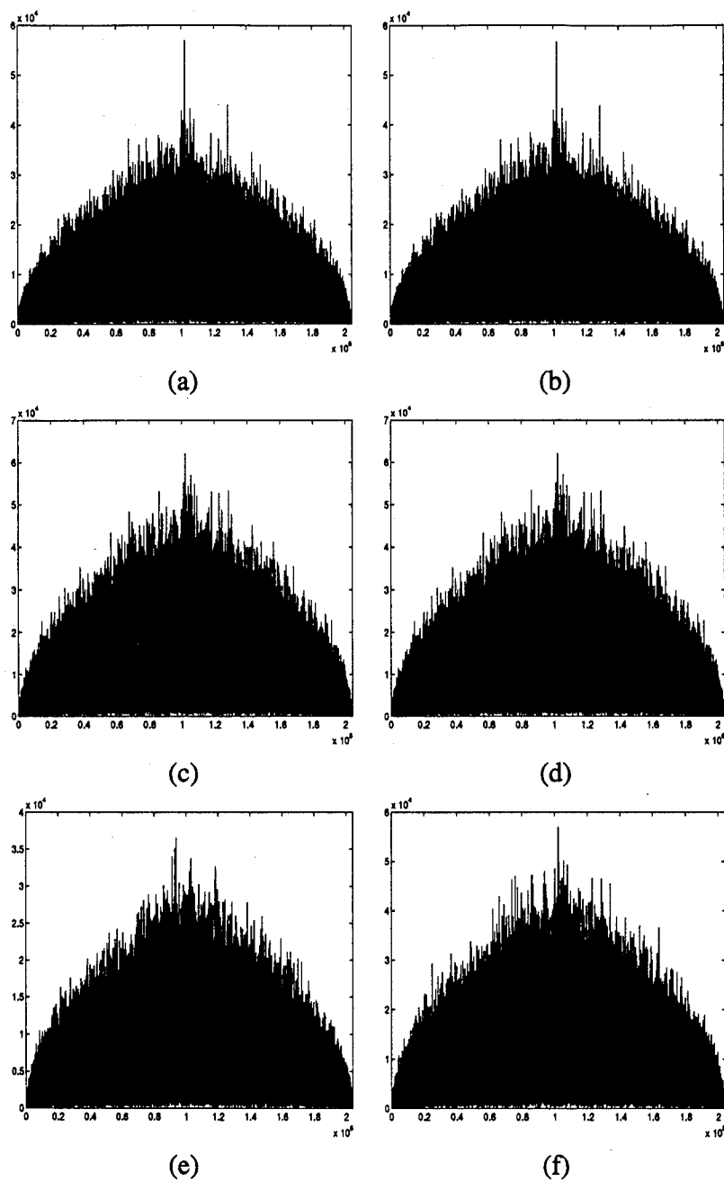
Figure 33. Cross Correlations For Broadband Noise Jammer: (a) & (b) 6 dB J/N with 6 & 9 dB Threshold (c) & (d) 9 dB J/N with 6 & 9 dB Threshold (e) & (f) 9 dB J/N with 1 & 3 dB Threshold
