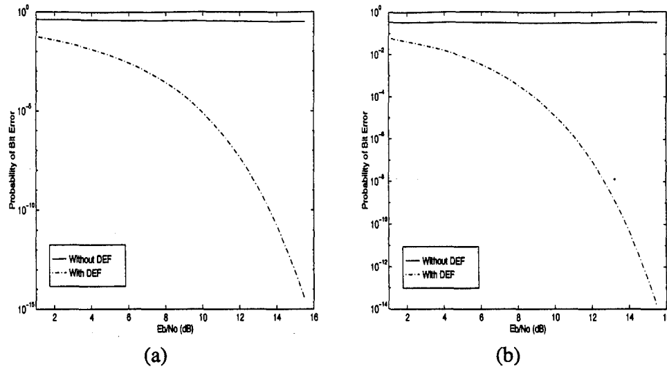
Figure 29. BER Curves For 1 Pulsed CW Jammer: (a) 33 dB J/N (b) 50 dB J/N (Note the scale difference)
