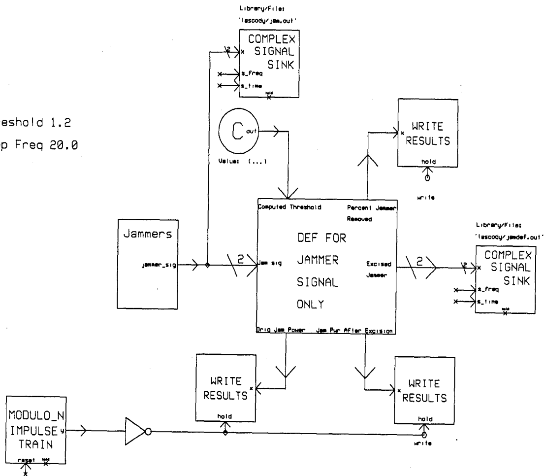
Figure 22. SPW Model for Determining Jammer Power
