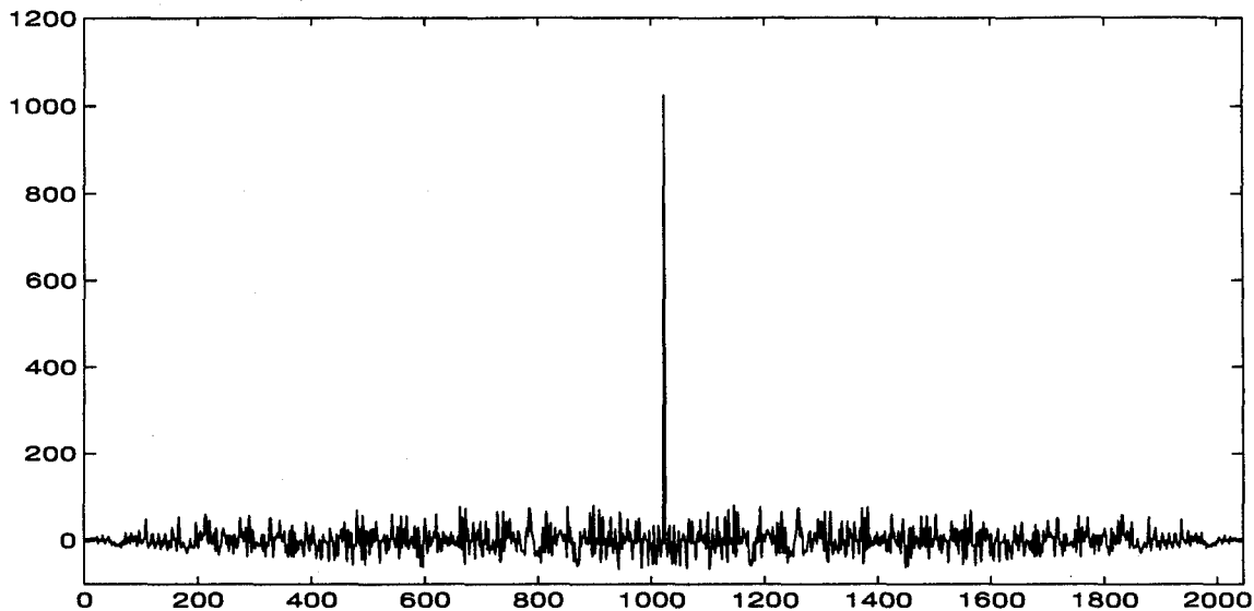
Figure 19. Sample Correlation Sequence Used to Calculate PAR
