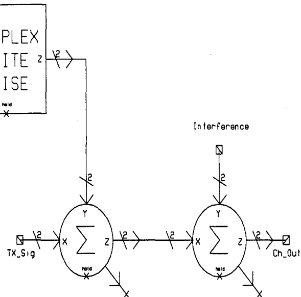
Figure 12. Channel Model
