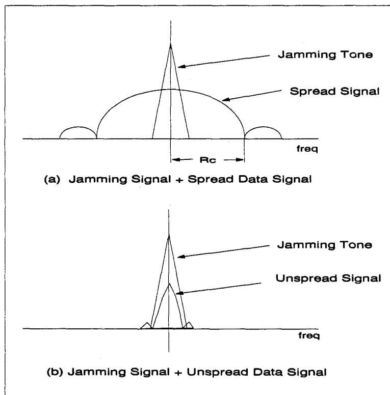
Figure 4. Example of Jammer Effects upon Spread and Unspread Signals
