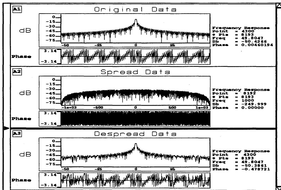
Figure 15. Spectra of Data
