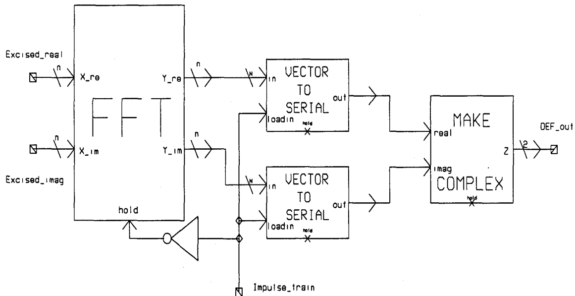
Figure 10. Third DEF Subsystem
