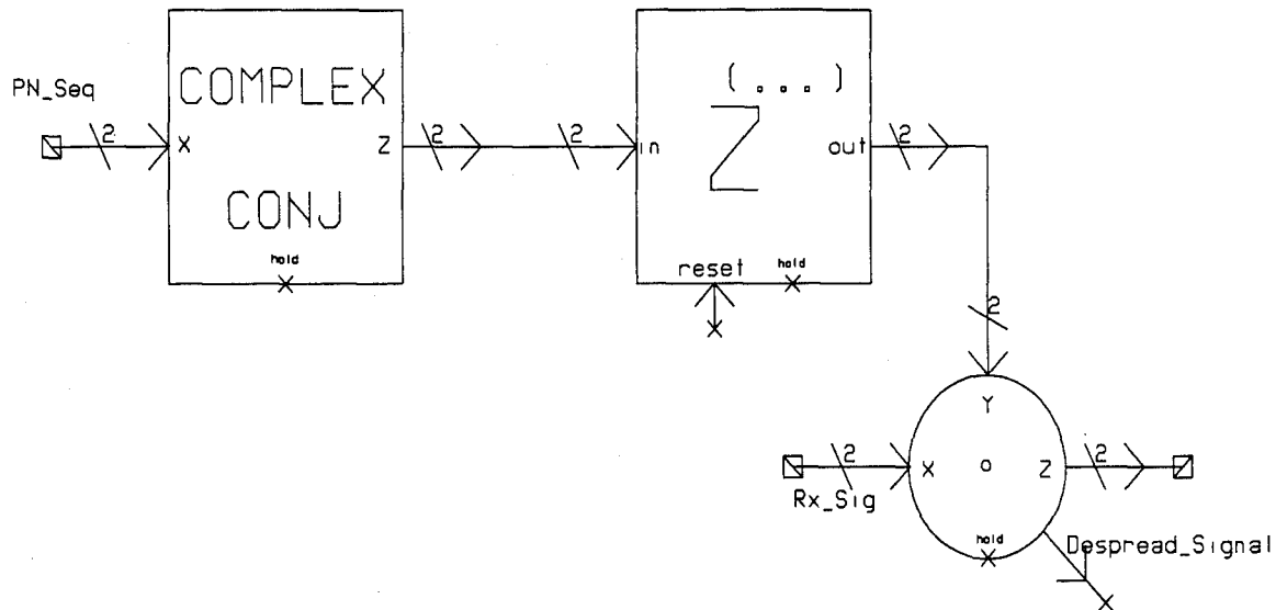
Figure 7. Despreading Block
