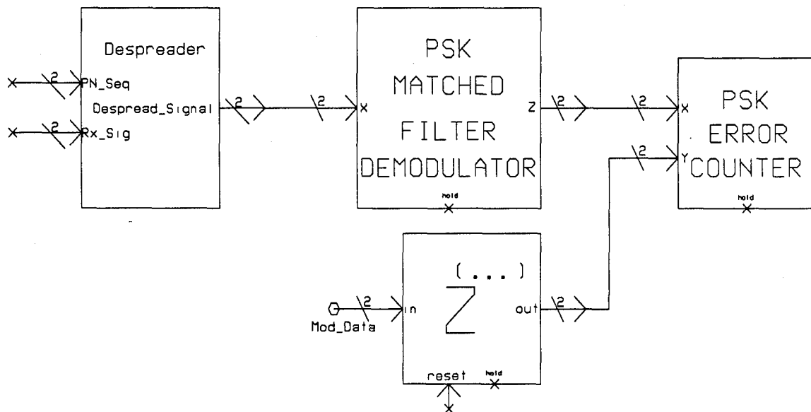
Figure 6. Direct Sequence Spread Spectrum Receiver
