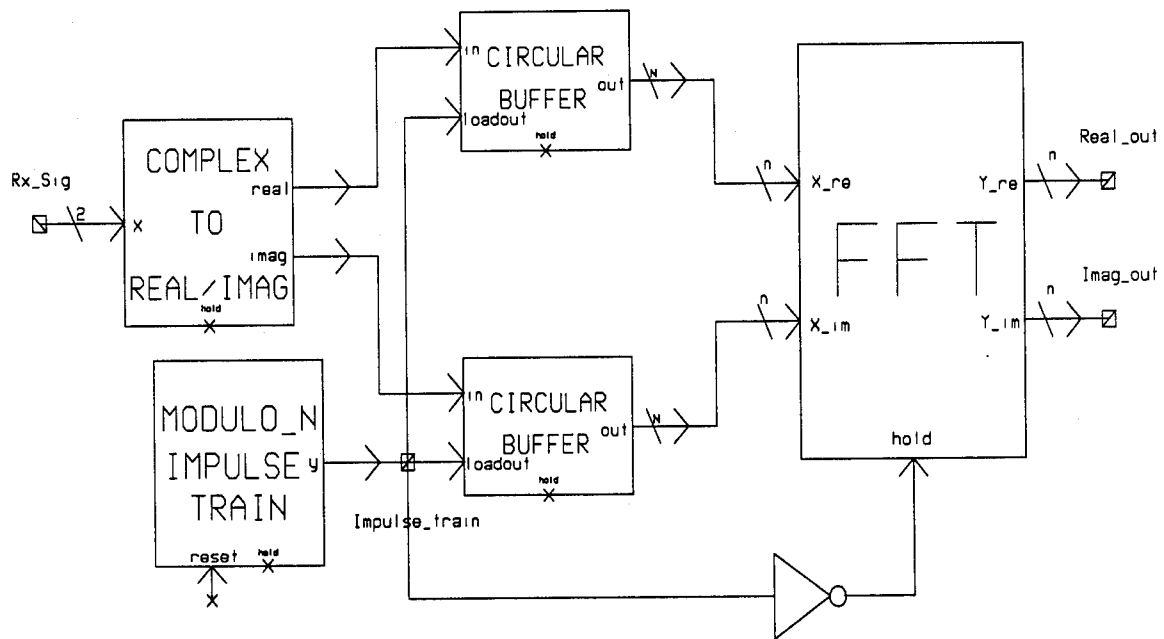
Figure 8. First DEF Subsystem
