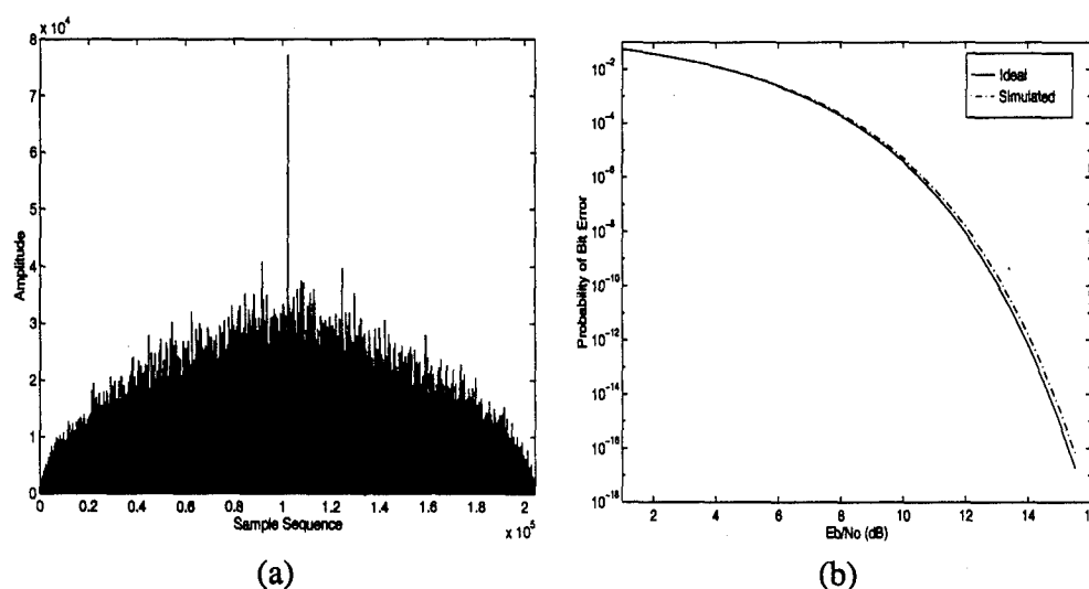
Figure 23. Results of Scenario #1: (a) PAR Correlation Sequence (b) Baseline BER Curve
