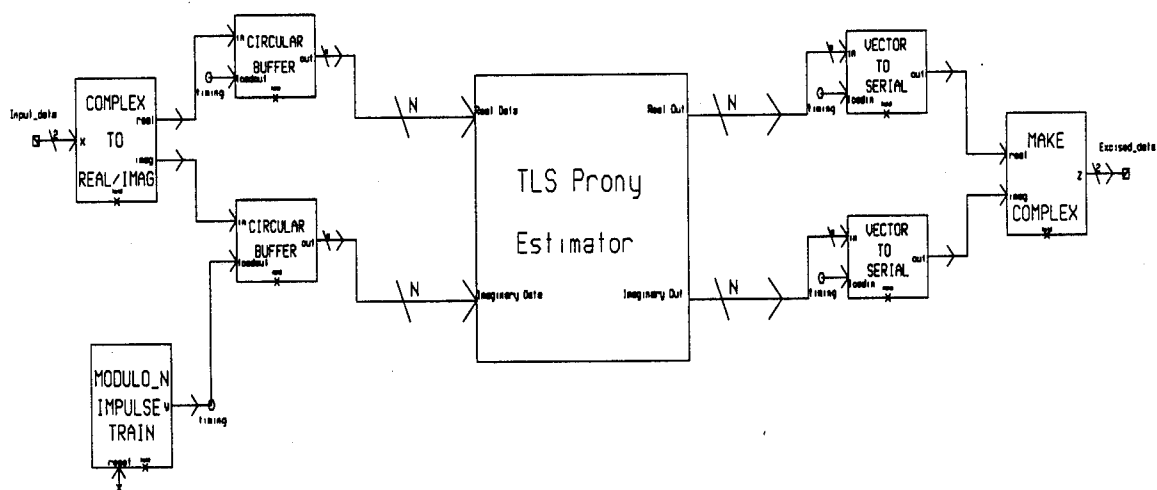
Figure 21. TLS Prony Subsystems
