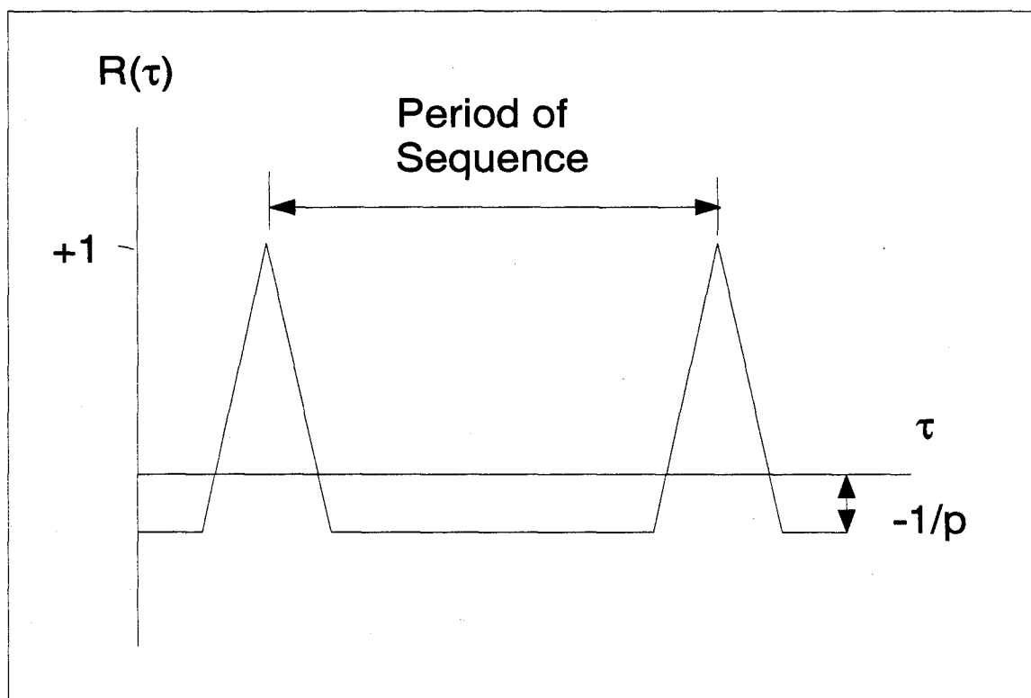
Figure 3. Typical PN Auto-Correlation Function
