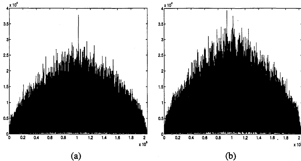
Figure 28. Cross Correlations For 1 Pulsed CW Jammer: (a) 53 \text{ dB J/N} with 6 \text{ dB} Threshold (b) 53 \text{ dB J/N} with 9 \text{ dB} Threshold
