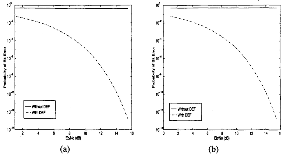
Figure 26. BER Curves For 4 CW Jammers: (a) 33 dB J/N (b) 50 dB J/N
