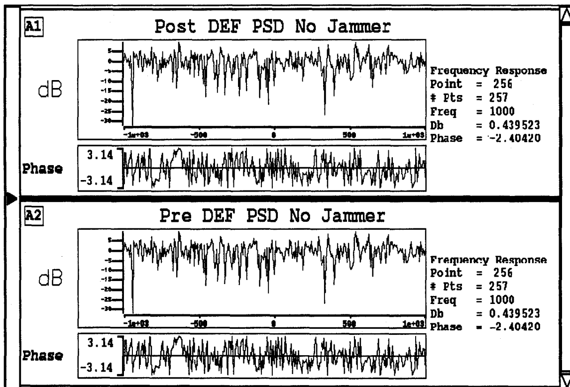
Figure 17. Spectra Plots of DEF and Channel Output With No Jammer Present
