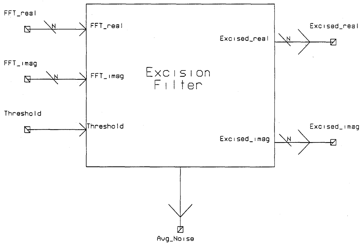
Figure 9. Second DEF Subsystem
