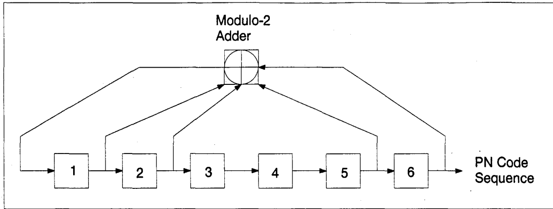
Figure 2. Linear Shift Register PN Code Sequence Generator
