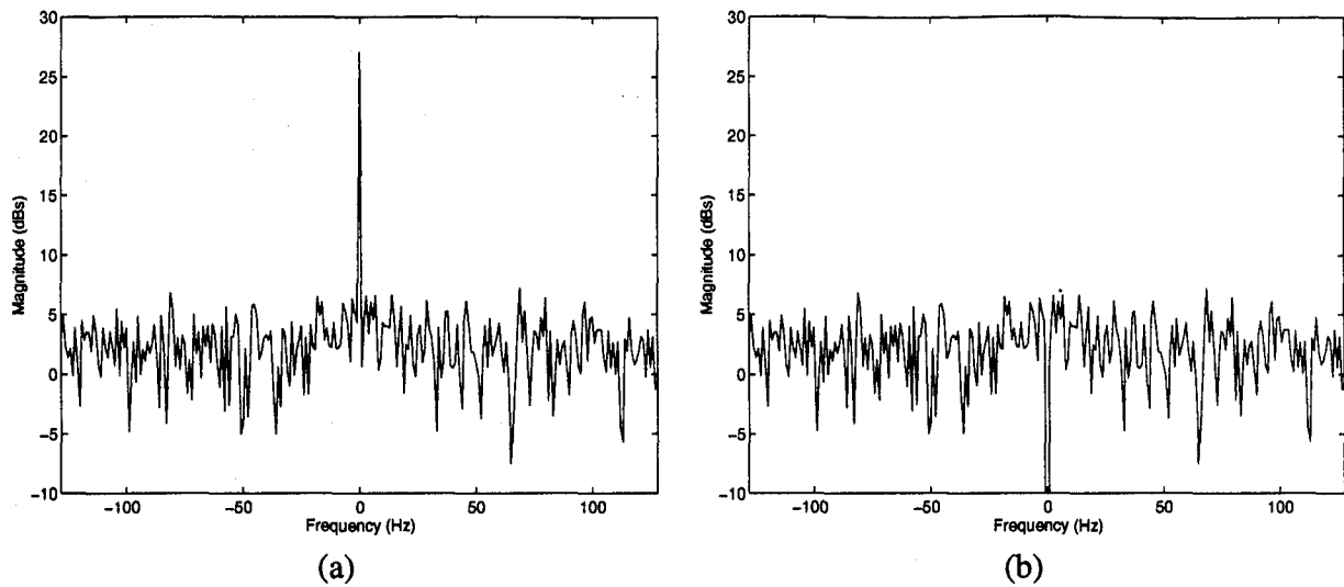
Figure 16. Spectra Plots for 1 Jammer: (a) Channel Output (b) DEF Output
