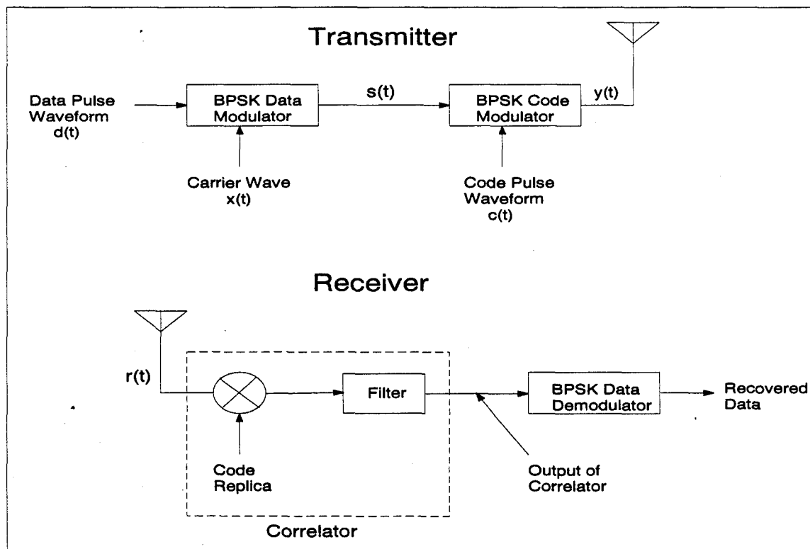
Figure 1. Direct Sequence Spread Spectrum Transmitter and Receiver
