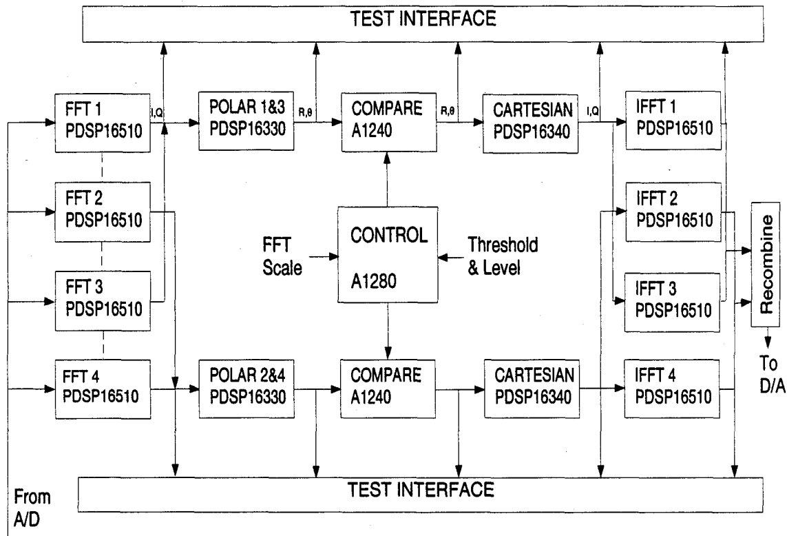
Figure 34. Data Flow Through DEF Circuit Card Assembly
