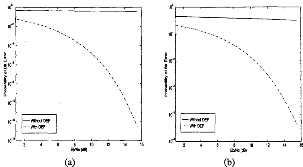
Figure 31. BER Curves For 4 Pulsed CW Jammers: (a) 33 dB J/N (b) 50 dB J/N (Note the scale difference)
