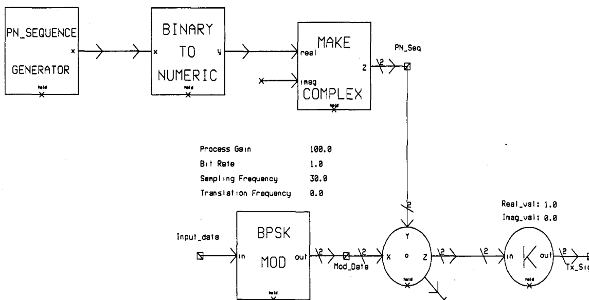
Figure 5. Direct Sequence Spread Spectrum Transmitter
