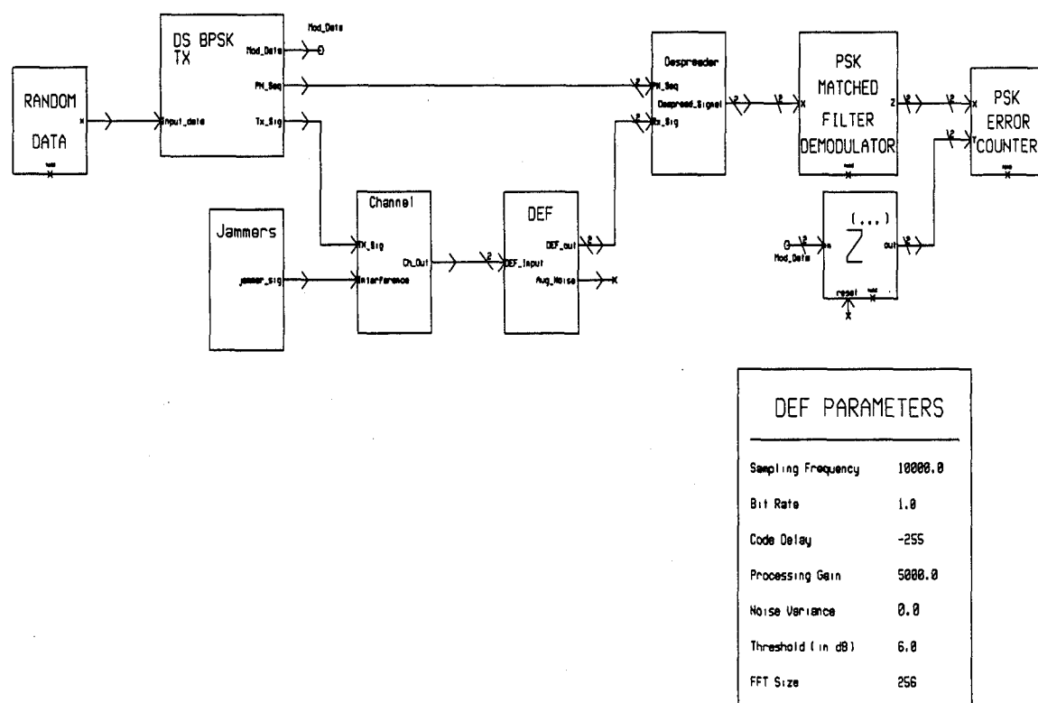
Figure 14. DS BPSK System Model
