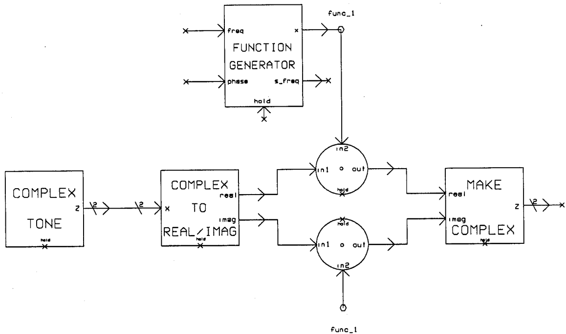
Figure 13. Jammer Model
