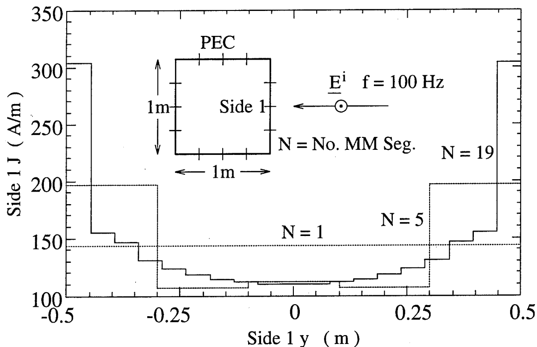
Figure 2.6: The magnitude of the current on Side 1 of a perfectly conducting square shield for N/4 = 1, 5 , and 19 MM expansion function per side.
