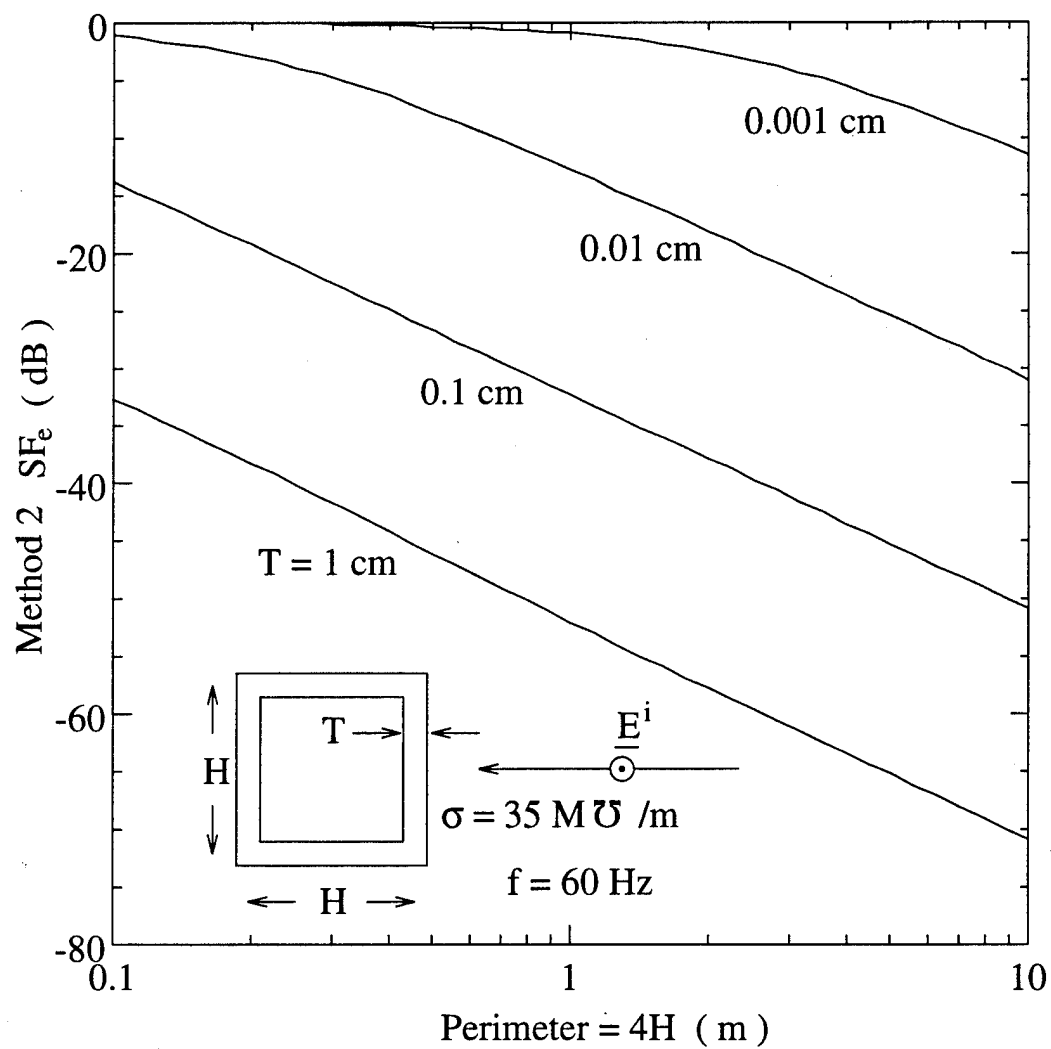
Figure 3.6: The Method 2 electric shielding factor versus the perimeter of an aluminum shield at f = 60 Hz.
