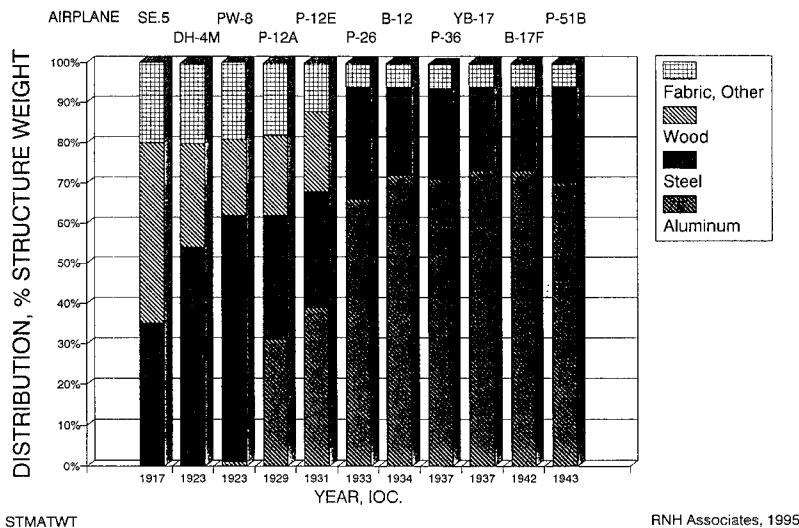
Figure 3.4 USAAC Aircraft Material Distribution 1917-1943
