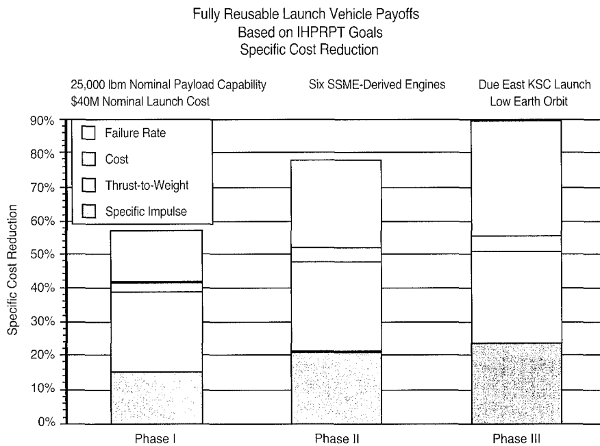
Figure 10.2 IHRPT Goals for a Fully Reusable Launch Vehicle
