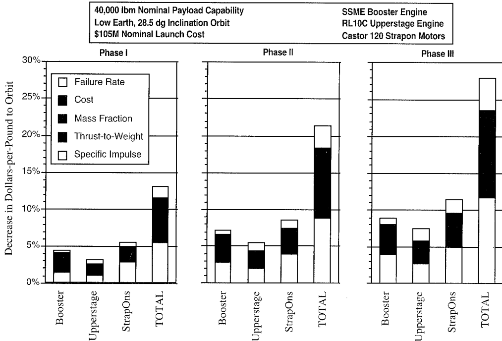
Figure 10.3 IHPRPT Goals for Expendable Launch Vehicles
