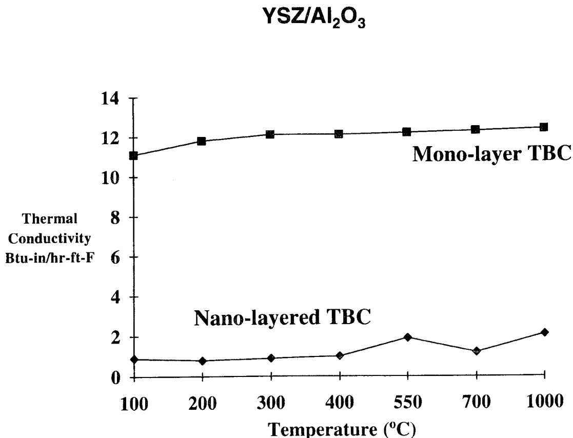
Figure 8.7 Comparison of the thermal conductivity as a function of temperature for mono-layered thermal barrier coatings and multilayered materials
