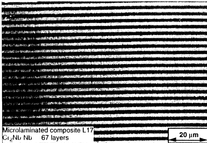
Figure 8.5. An electron micrograph of a microlaminated micro-composite consisting of 67 layers of Cr 2 Nb/Nb
