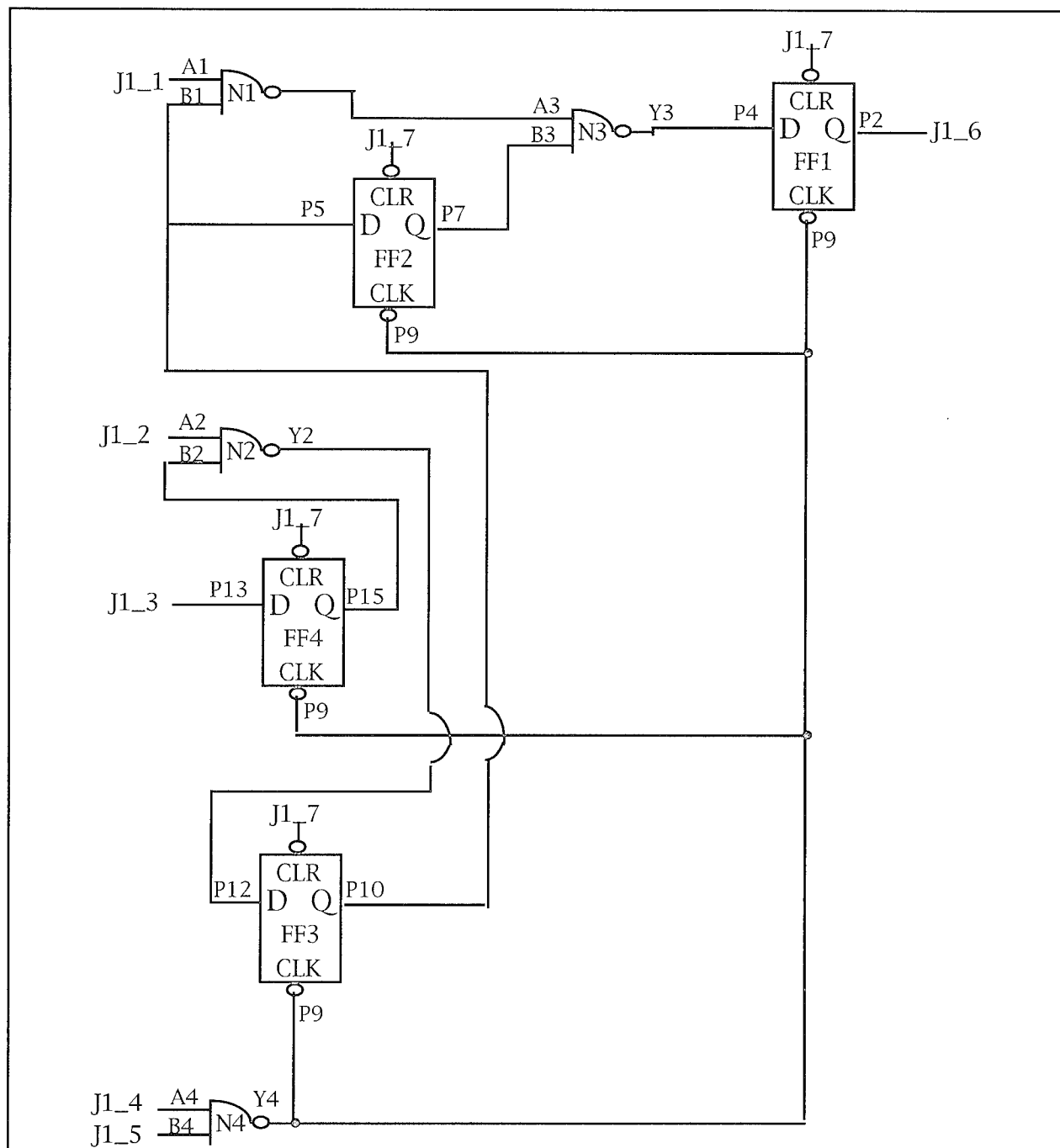
FIGURE C1. EXAMPLE CIRCUIT
