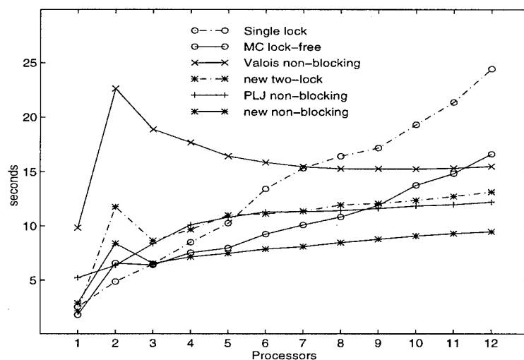
Figure 3: Net execution time for one million enqueue/dequeue pairs on a dedicated multiprocessor.
