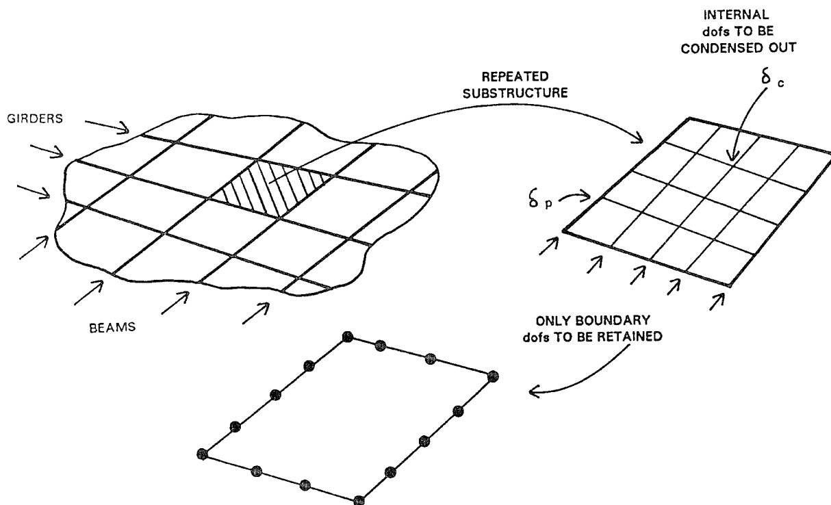
FIGURE 3-3.9 Schematic Illustration of The Static Condensation Process
