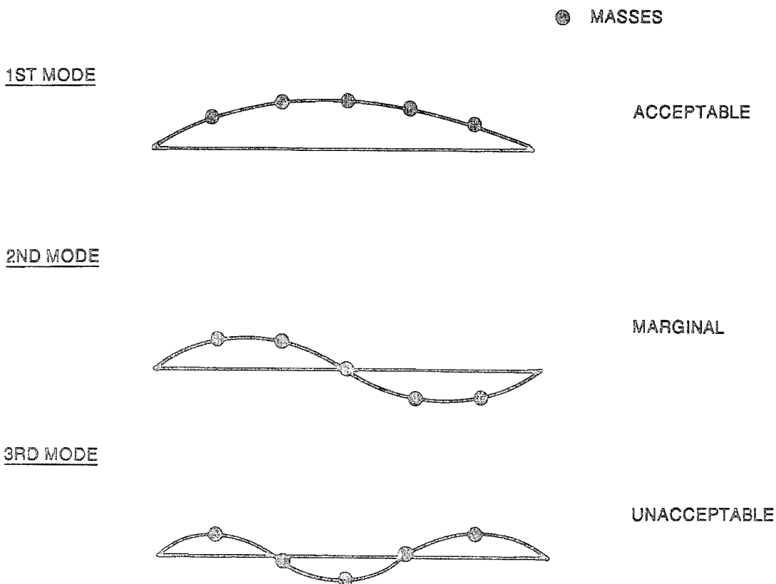
FIGURE 3-2.4 Mass Distribution Required for Accurate Determination of Natural Frequencies
