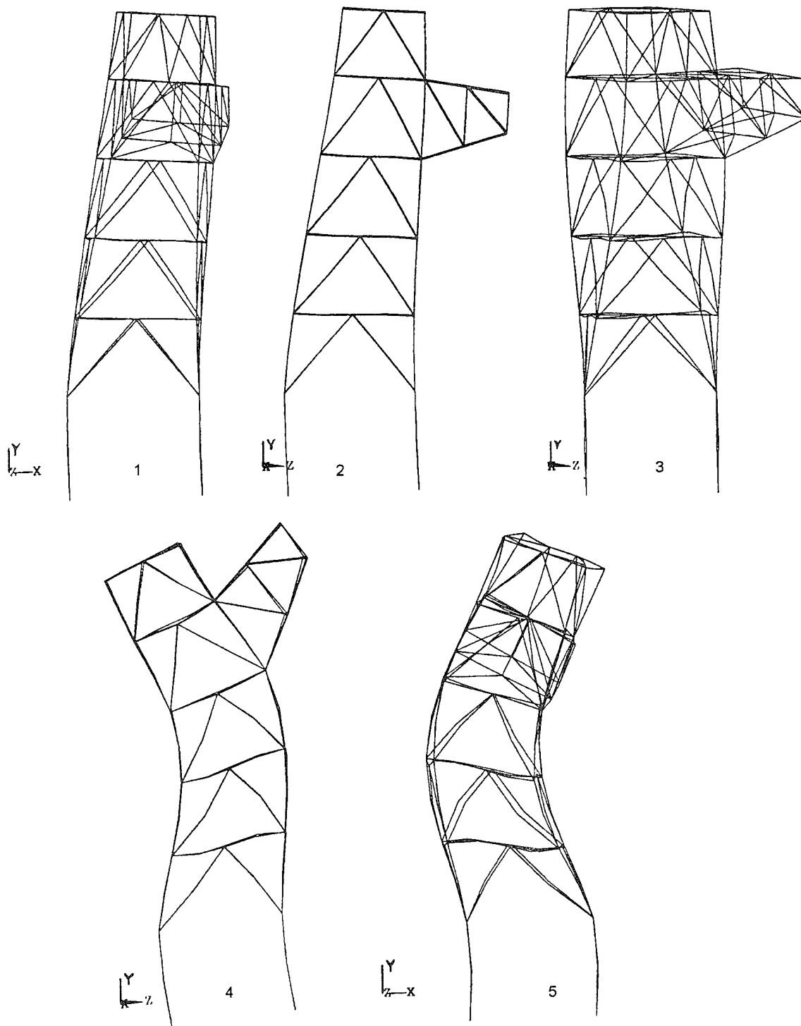
The first five mode shapes
