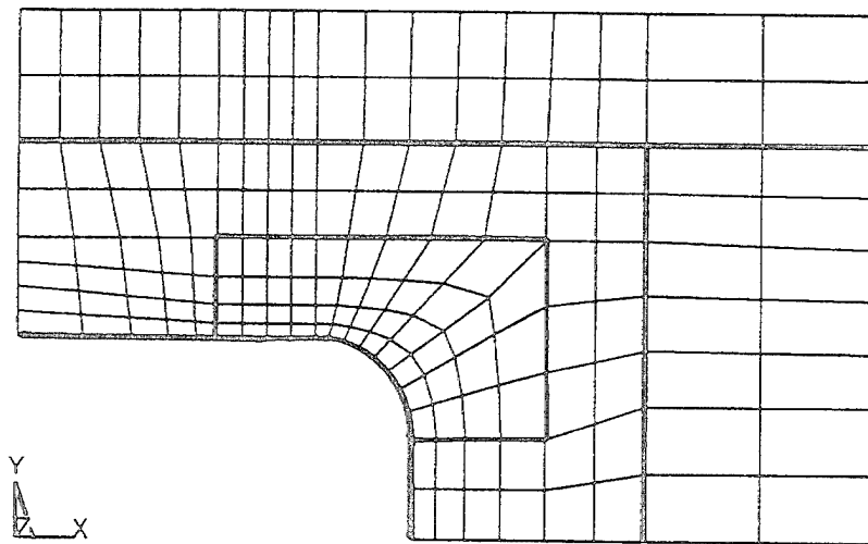
FIGURE 4.2-1 Benchmark Problem BM-1 : Reinforced Deck Opening
