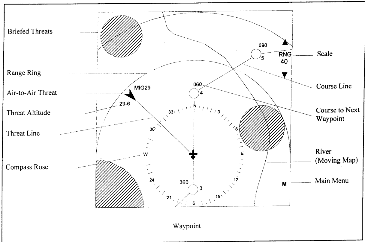
Figure 7. TSD Symbology Formats
