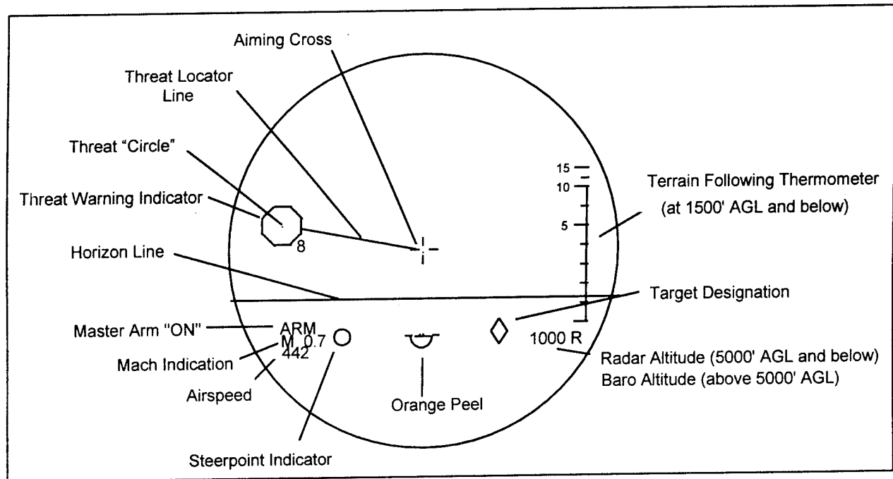
Figure 2.15.15 Modified HMD Symbology
