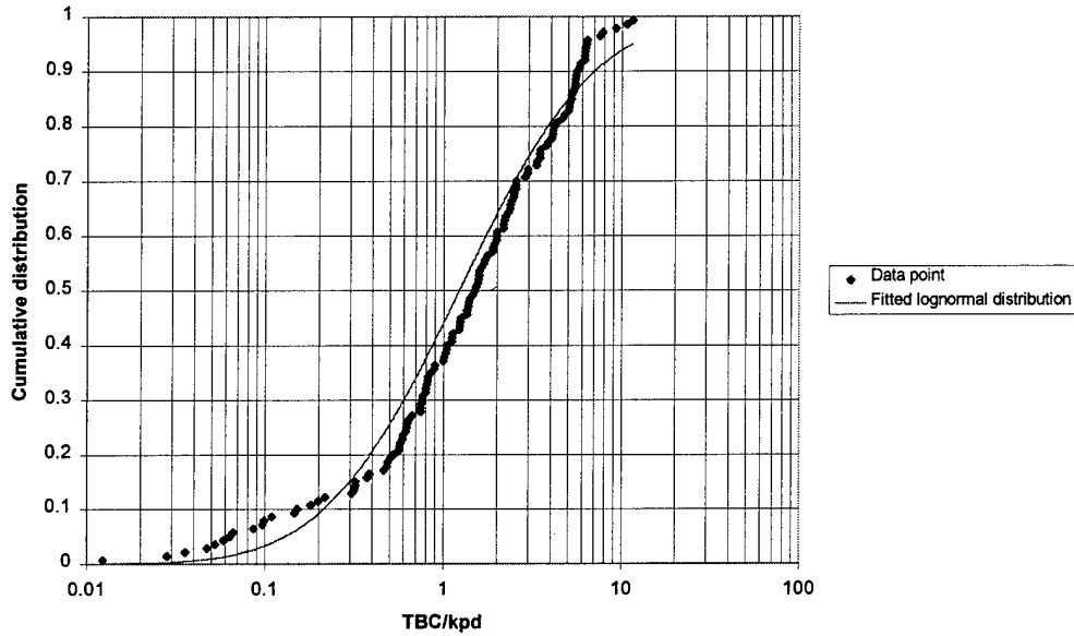
Figure 6-2. Distribution of Nonzero TBC Rates for US 3d Corps in World War II
