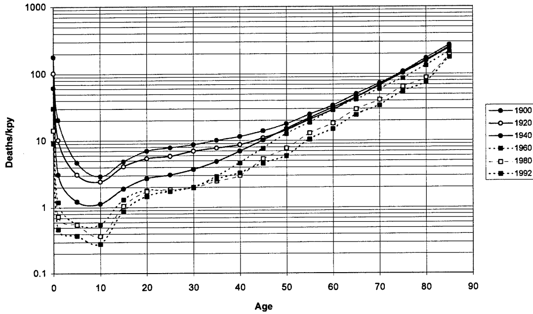
Figure 2-3. Peacetime Mortality of US Males by Age and Calendar Year
