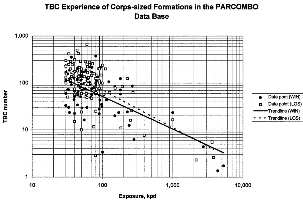
Figure 6-48. TBC Experience of the Winner and Loser for Corps-sized Formations in the PARCOMBO Data Base
