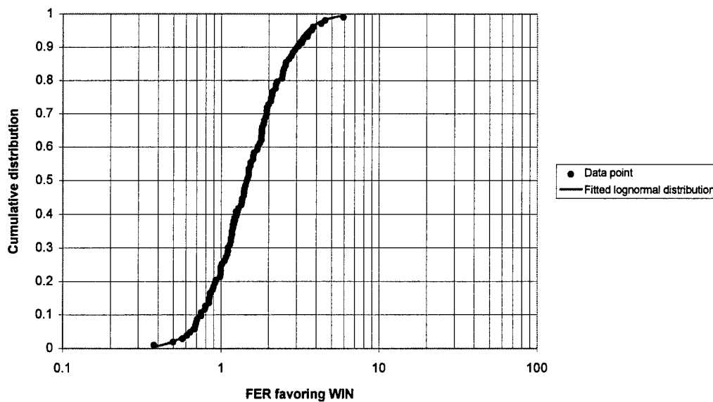
Figure 6-51. Distribution of FER Favoring the Winner for Corps-sized Formations in the PARCOMBO Data Base
