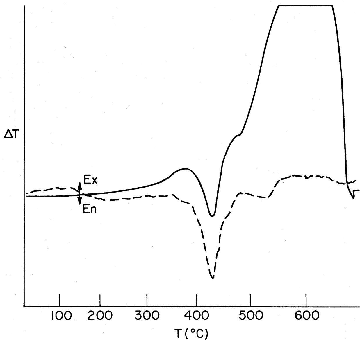
Figure 49. Differential thermal analysis records of modified polyphenylene oxide heated at 5 C/min in helium (broken curve) and air (smooth curve)
