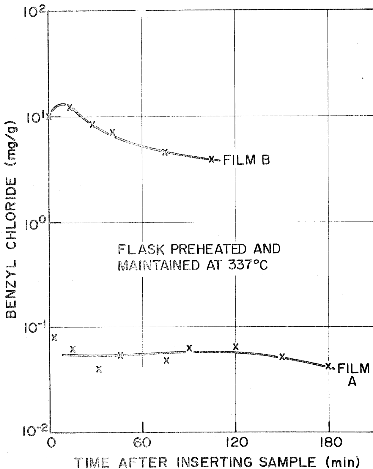
Figure 14. Benzyl chloride production by two meat-wrap films (A and B) heated at 337 C
