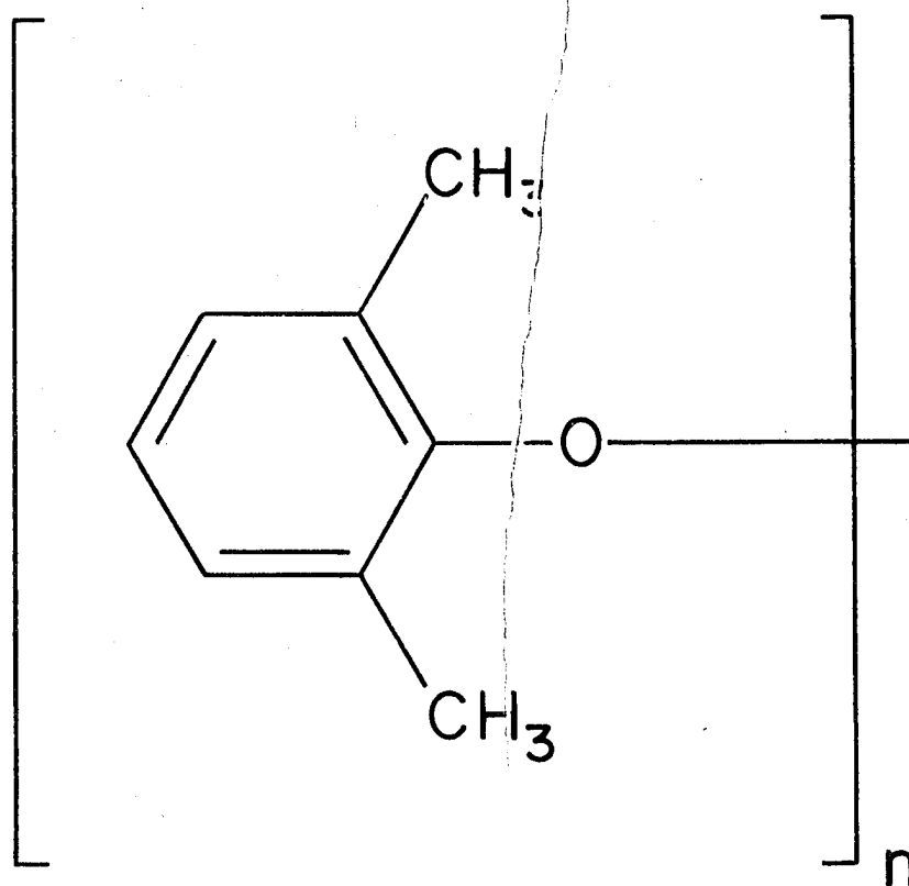
Figure 46. Poly-2,6-dimethyl-1,4-phenylene oxide
