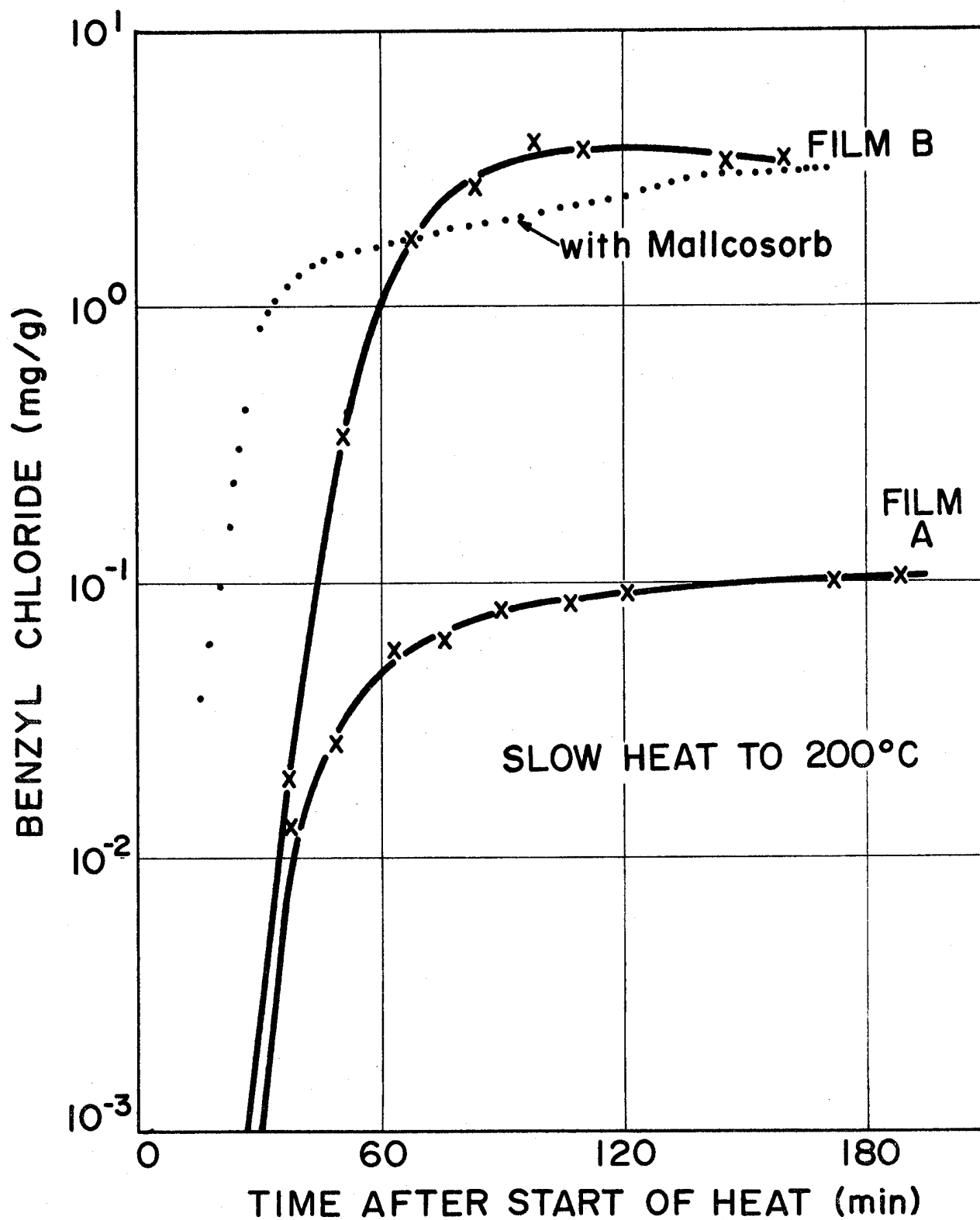
Figure 11. Benzyl chloride production by two meat-wrap films (A and B) heated slowly to 200 C
