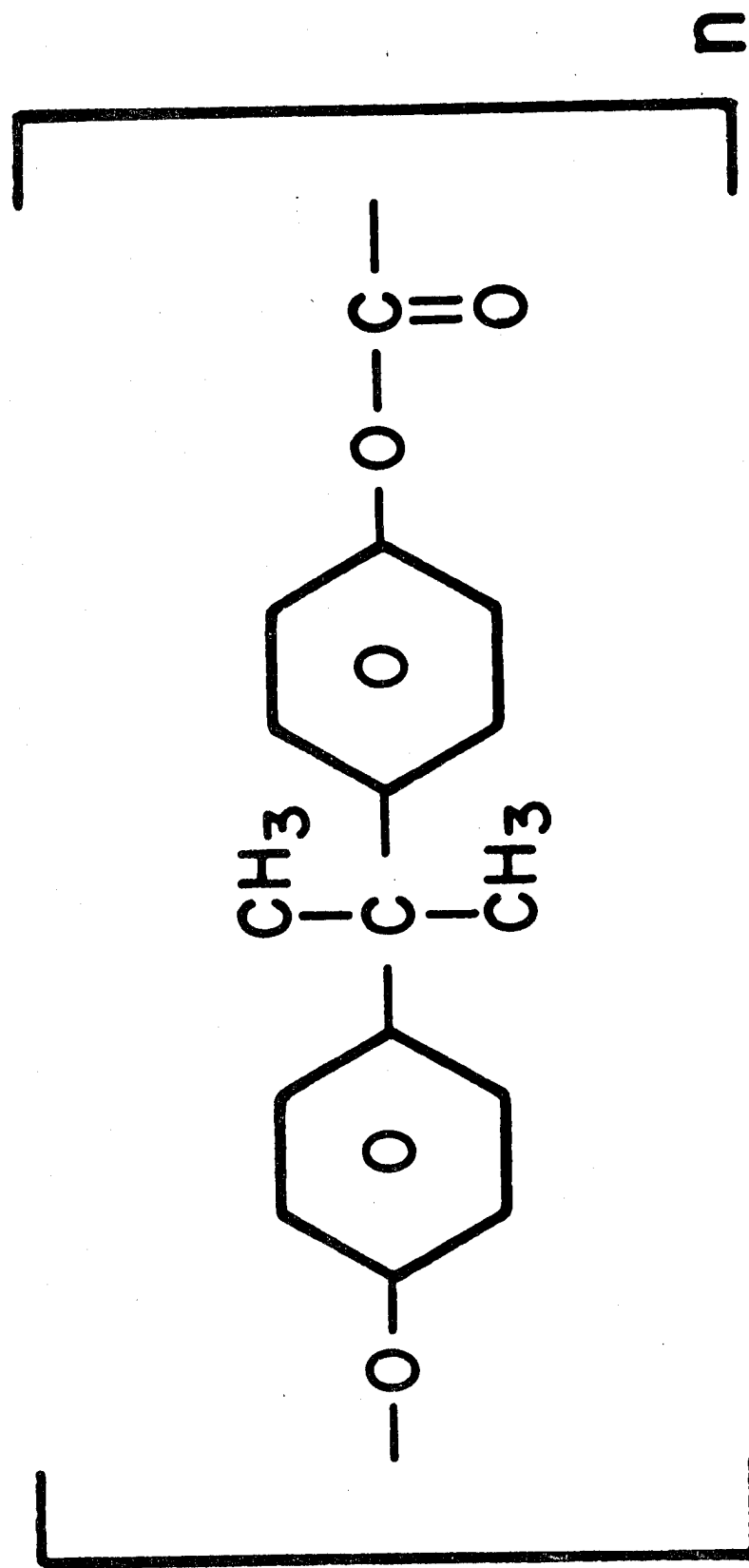
Figure 42. Bisphenol A-polycarbonate
