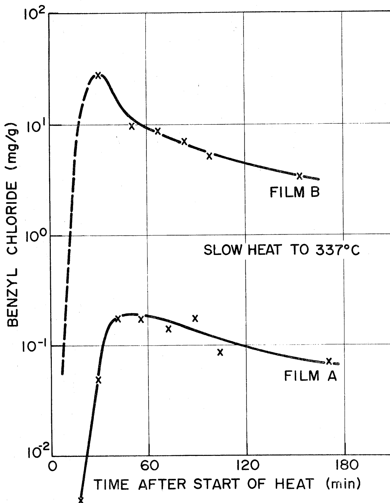
Figure 12. Benzyl chloride production by two meat-wrap films (A and B) heated slowly to 337 C
