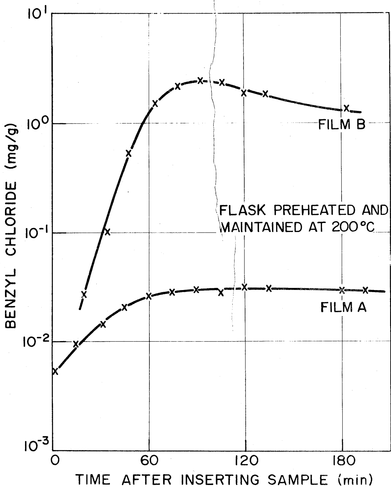
Figure 13. Benzyl chloride production by two meat-wrap films (A and B) heated at 200 C
