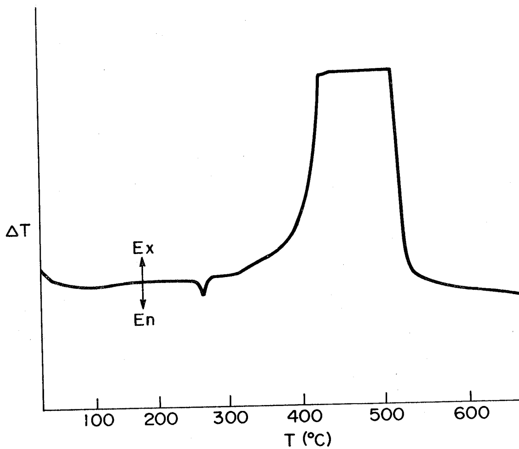
Figure 54. Differential thermal analysis record of Dacron R heated at 5 C/min in air
