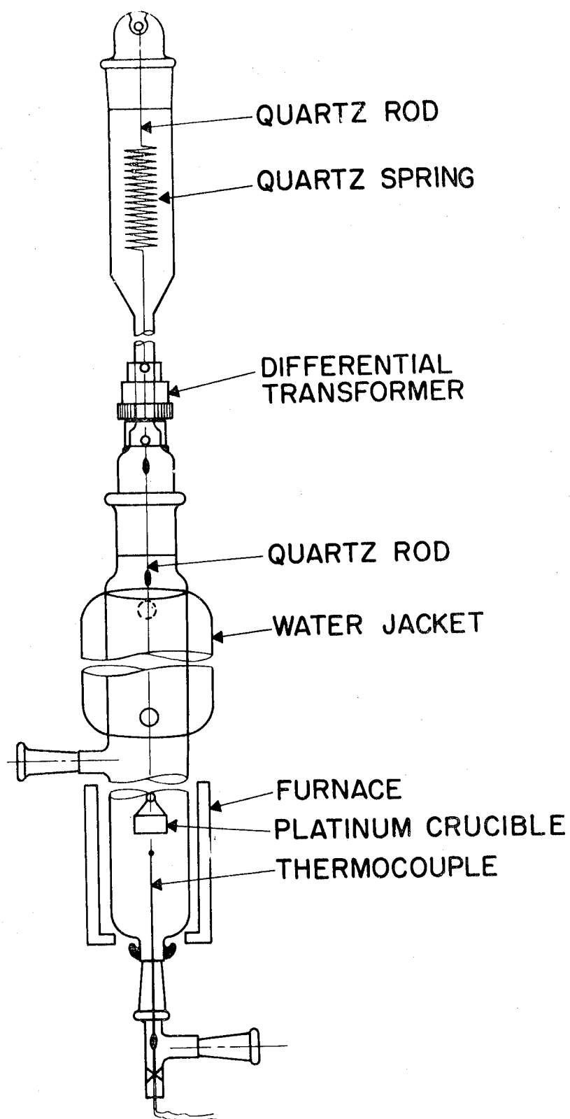
Figure 2. Schematic diagram of a thermogravimetric analysis (TGA) apparatus
