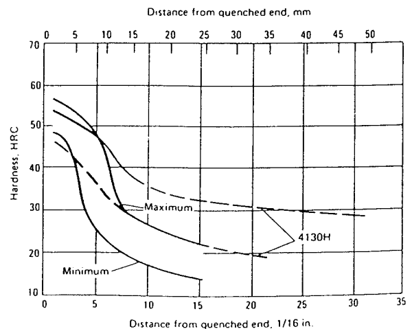
4130H: End-Quench Hardenability. 48 heats of 14835 containing 0.35 to 0.39 C, 0.65 to 1.10 Mn, 0.13 Ni max, 0.05 Cr max, 0.03 Mo max and boron treated; compared with 4130H. (Source: The Hardenability of Steels , American Society for Metals, 1977)
