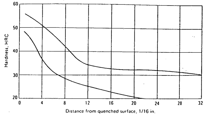
4130H: End-Quench Hardenability. (Source: Metals Handbook , 9th ed., Vol 1, American Society for Metals, 1978)
