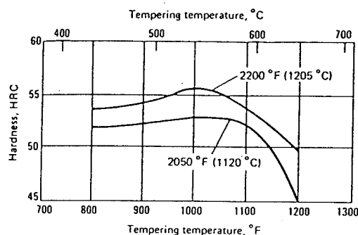
H24: Hardness Versus Tempering Temperature. H24 austenitized at the temperatures shown, oil quenched, and receiving single temper for 2 hr. (Source: Metals Handbook , 8th ed., Vol 2, American Society for Metals, 1964)
