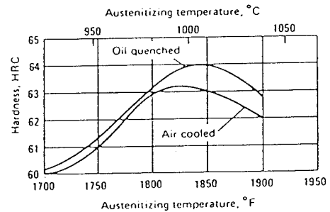
D2: As-quenched Hardness. Effect of quenching medium and austenitizing temperature on as-quenched hardness of a D2 tool steel containing 1.50 C. (Source: Tool Steels , American Society for Metals, 1980)
