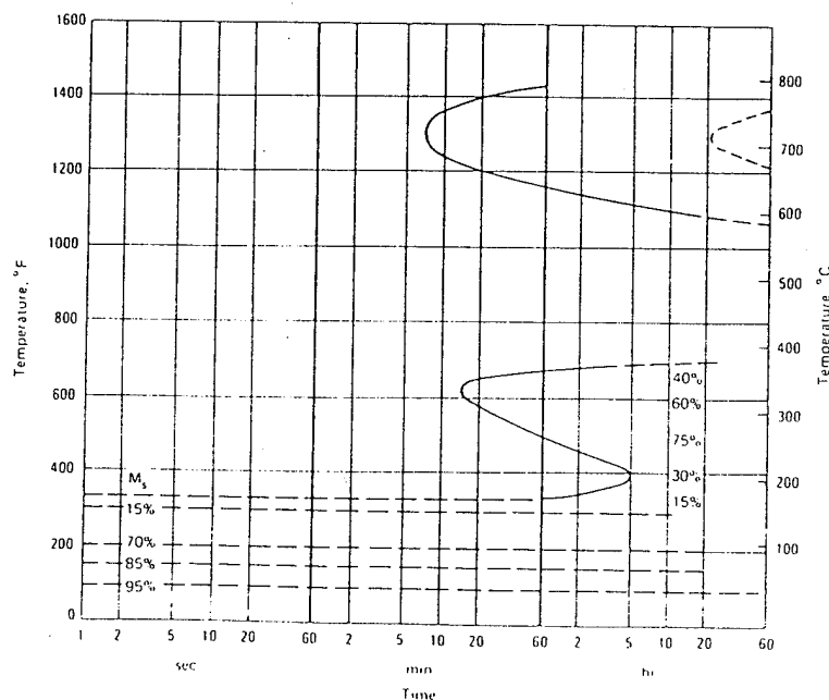
A2: Isothermal Transformation Diagram. Composition: 0.97 C, 0.48 Mn, 0.40 Si, 4.58 Cr, 1.04 Mo, and 0.25 V. Prior condition, annealed. Austenitizing temperature, 1850 °F (1010 °C). (Source: The Hardening of Tool Steels, by P. Payson and J. L. Klein; in Transactions of the American Society for Metals , Vol 31, No. 1, March 1943)
