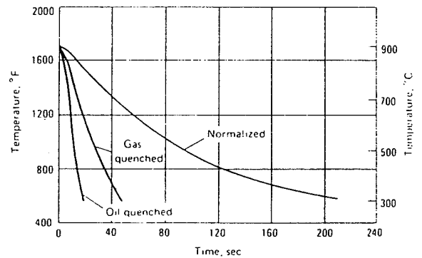
4130: Cooling Curves. Steel tubing, 1.25-in. (31.75-mm) outside diameter by 0.065-in. (1.651-mm) wall. (Source: Metals Handbook , 8th ed., Vol 2, American Society for Metals, 1964)
