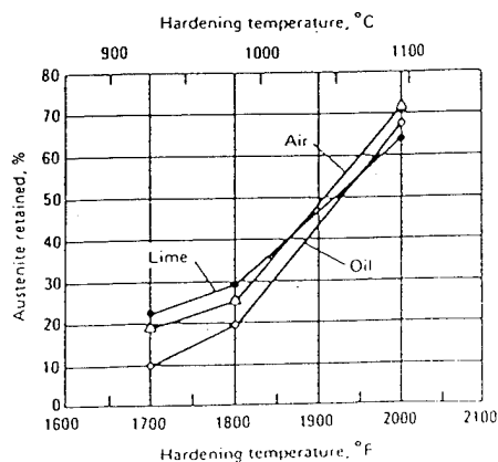
D2: Austenitizing Temperature Versus Retained Austenite. Composition: 1.60 C, 0.33 Mn, 0.32 Si, 11.95 Cr, 0.25 V, 0.79 Mo, 0.010 S, 0.018 P, when quenched in lime, air and oil. (Source: Tool Steels , American Society for Metals, 1980)
