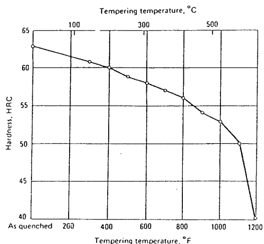
A4: Hardness Versus Tempering Temperature. Austenitized at 1550 °F (845 °C) and cooled in air. (Source: Metals Handbook , 8th ed., Vol 2, American Society for Metals, 1964)
