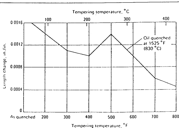
L6: Length Change as a Function of Tempering Temperature. A ½-in. round specimen of an L6 special-purpose tool steel containing 0.75 C, 0.35 Mn, 1.00 Cr, 1.75 Ni. (Source: Tool Steels, American Society for Metals, 1980)
