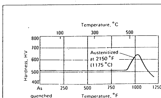
H19: Hardness Versus Tempering Temperature. H19 austenitized at 2150 °F (1175 °C). (Source: Jessop-Saville)
