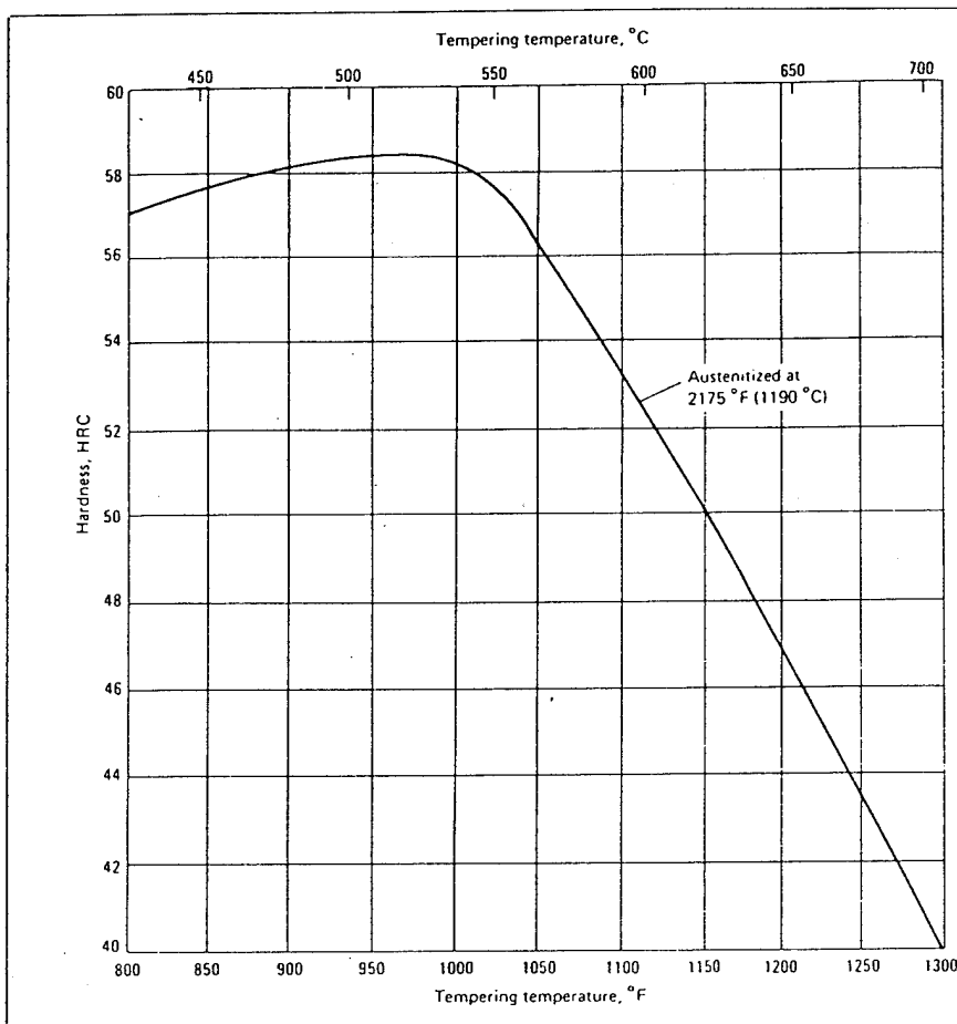
H19: Hardness Versus Tempering Temperature. H19 oil quenched from 2175 °F (1190 °C) and double tempered. (Source: Universal-Cyclops)
