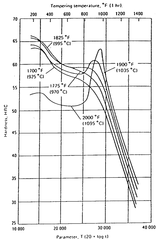
D4: Hardness Versus Tempering Temperature. Tempering curves for D4 tool steel containing 2.17 C, 11.68 Cr, 0.78 V, 0.51 Co; austenitized at the five temperatures shown, cooled in air, and tempered for 1 hr at the tempering temperature. (Source: Teledyne VASCO)
