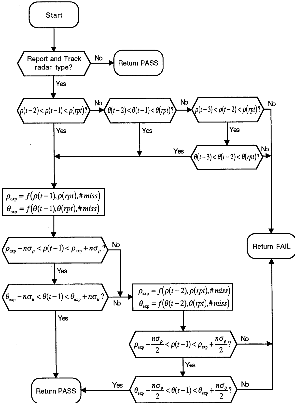
Figure 7. Linearity test.
