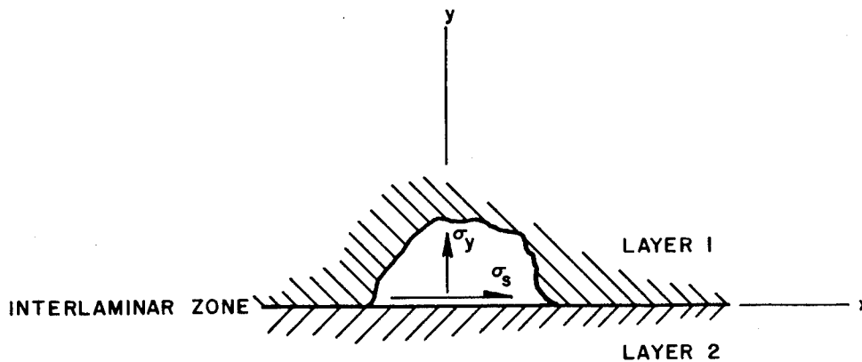
Figure 16. Interlaminar Stresses
