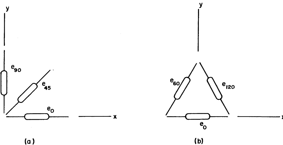
Figure 5. Strain Rosettes
