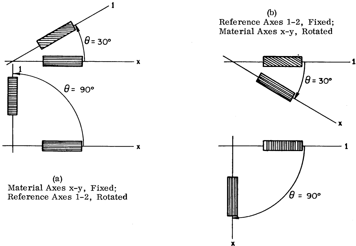
Figure 6. Equivalent Transformations
