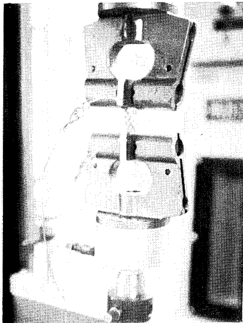
Figure 3 PNEUMATIC JAW DETAIL Top: Upper Jaw with Silver Oxide Plates for Resistance Tensile measurement Center: Tensile Sample Bottom: Lower Jaw
