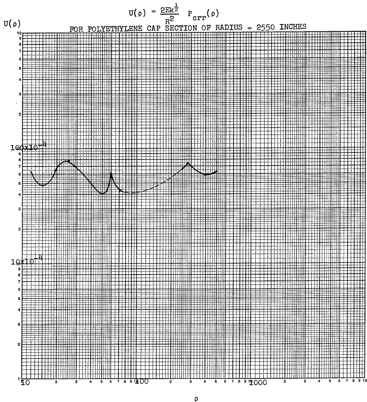
Figure 10 THE FUNCTION U(\rho) = \frac{P_{cr}}{t^2}
