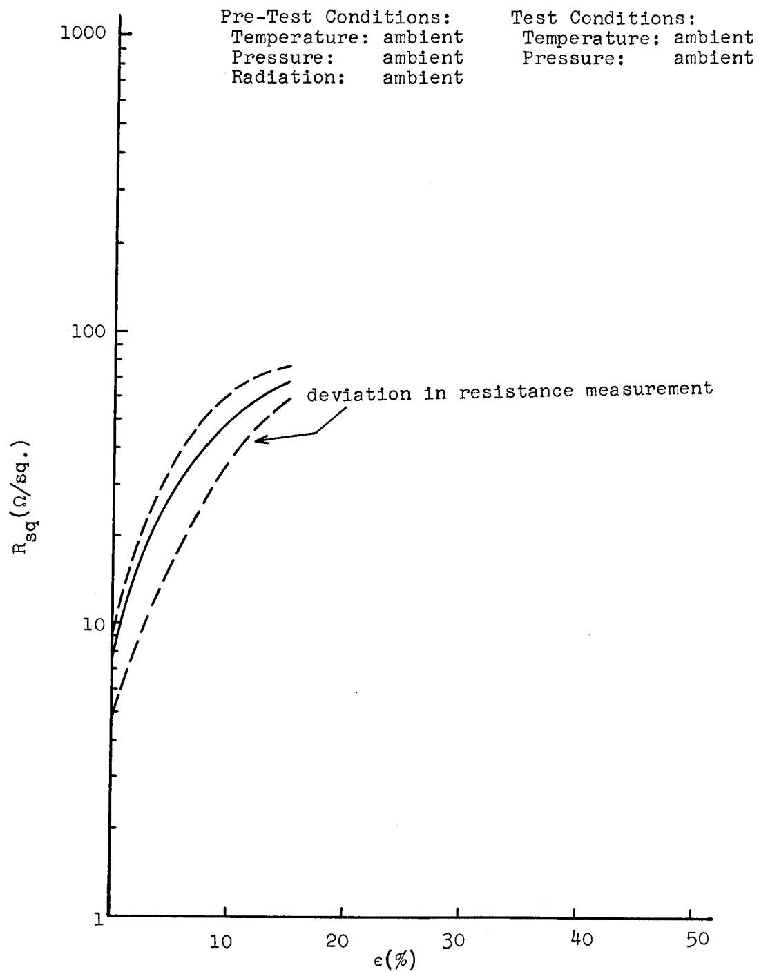
Figure 52 SURFACE RESISTANCE VS. STRAIN FOR COMPLETED MATERIAL, NON-PERFORATED (in 90° Direction)
