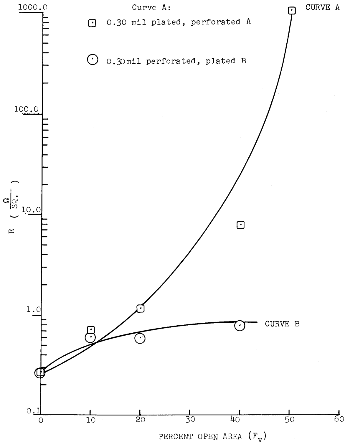
Figure 9 RESISTANCE ( \Omega/SQ. ) OF PERFORATED 0.30 MIL STANDARD DENSITY POLYETHYLENE FILM VS. PERCENT OPEN AREA (Plated to 15 \times 10^{-6} in. Cu on both sides)
