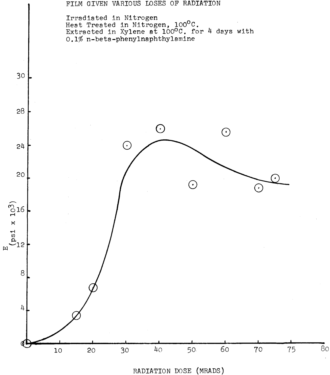
Figure 4 EFFECT OF COMPLETE EXTRACTION ON STRENGTH OF 1 MIL STANDARD DENSITY SEA SPACE POLYETHYLENE FILM GIVEN VARIOUS LOSES OF RADIATION
