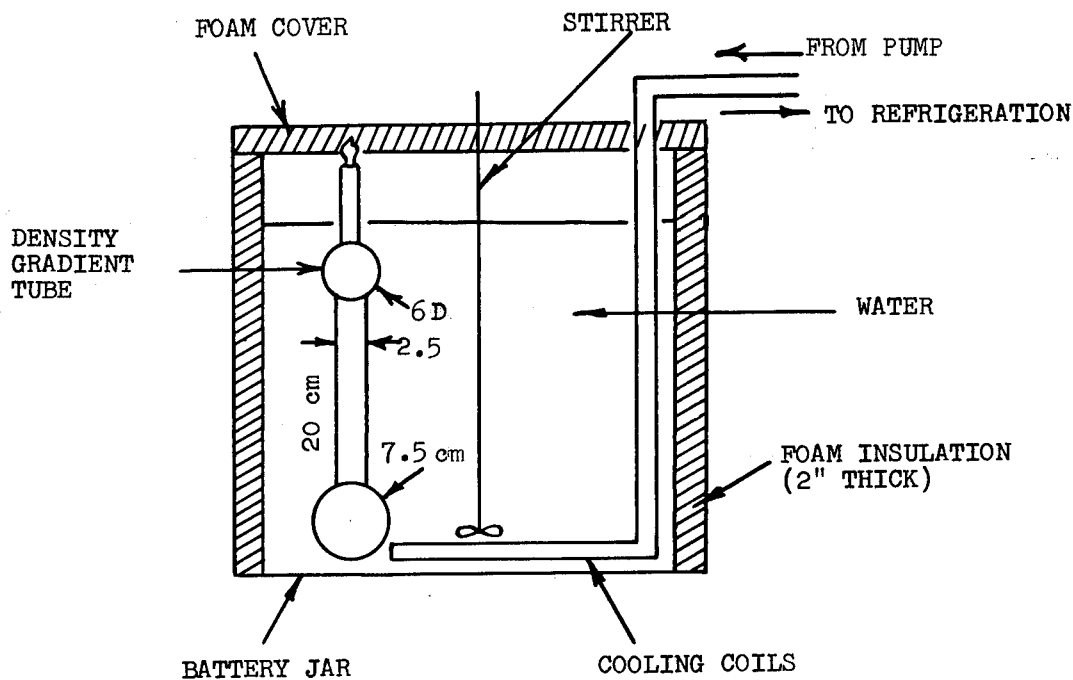
Figure 1: DENSITY GRADIENT APPARATUS
