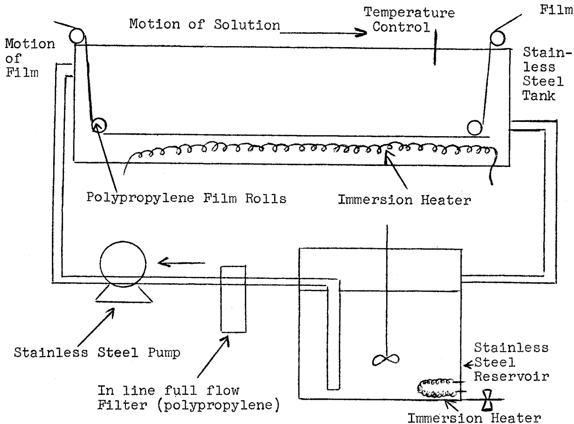
Figure 42 SCHEMATIC OF SENSITIZER OR ACTIVATOR SYSTEMS
