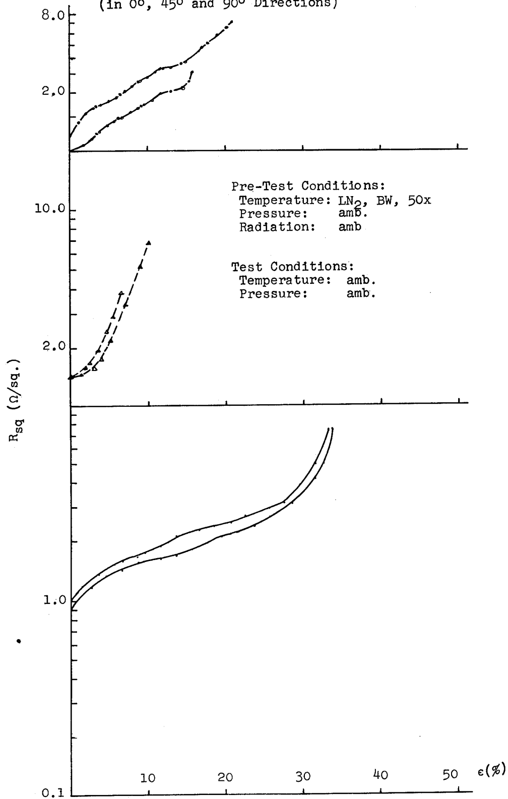
Figure 66 SURFACE RESISTANCE VS. STRAIN FOR COMPLETED MATERIAL (in 0°, 45° and 90° Directions)
