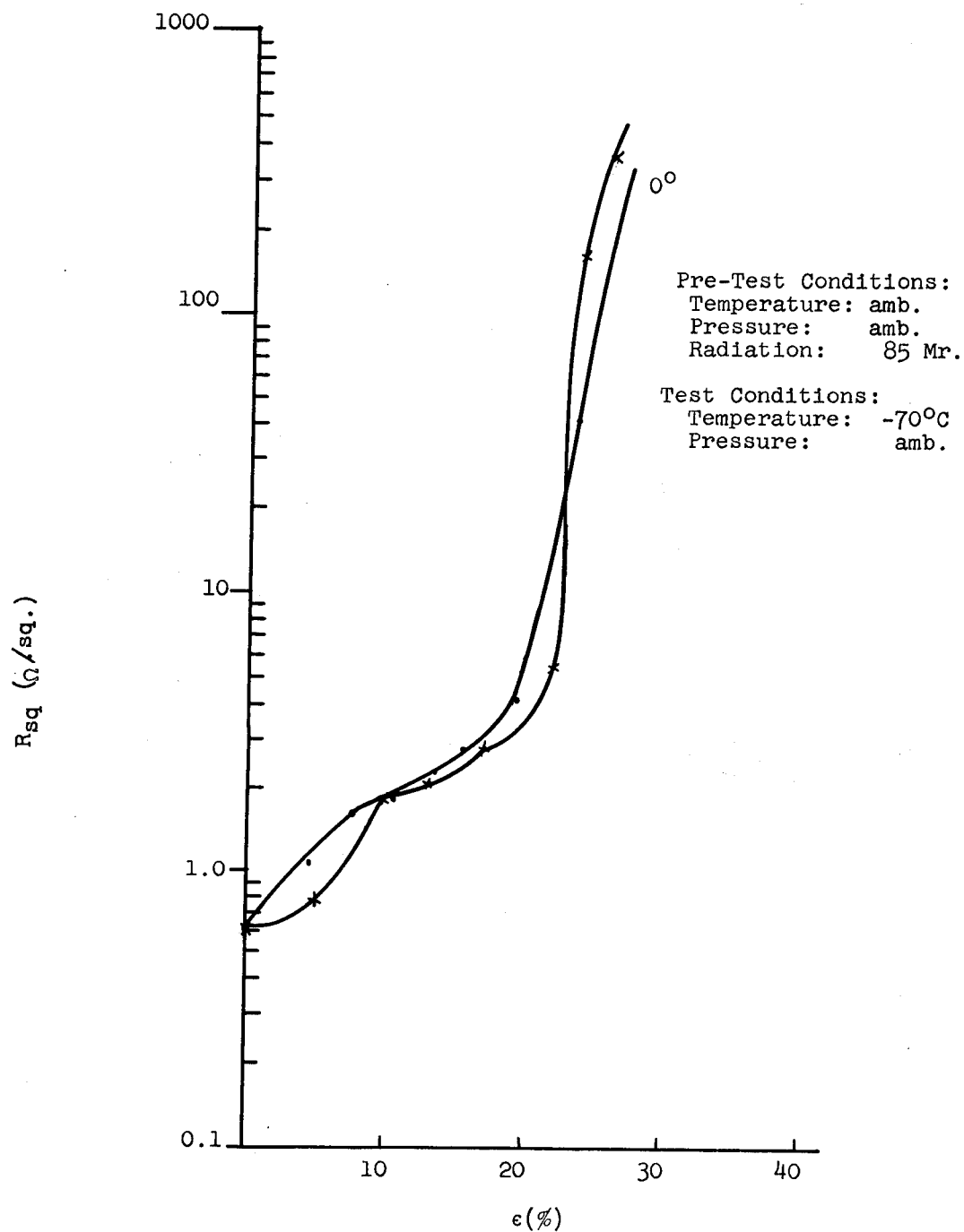
Figure 60 SURFACE RESISTANCE VS. STRAIN FOR COMPLETED MATERIAL (0° Direction)
