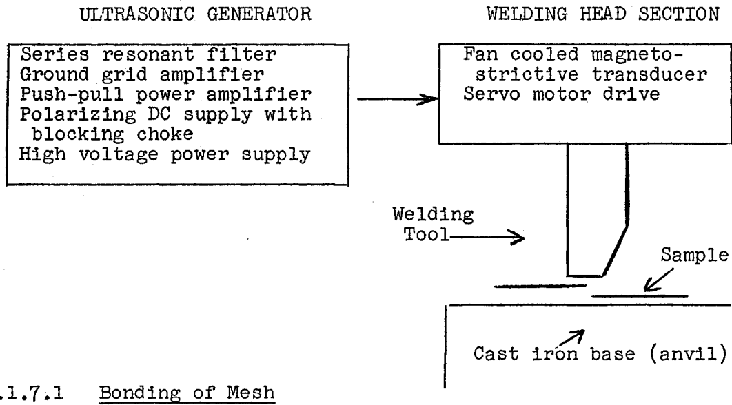
Figure 36: SCHEMATIC DIAGRAM OF ULTRASONIC BONDER
