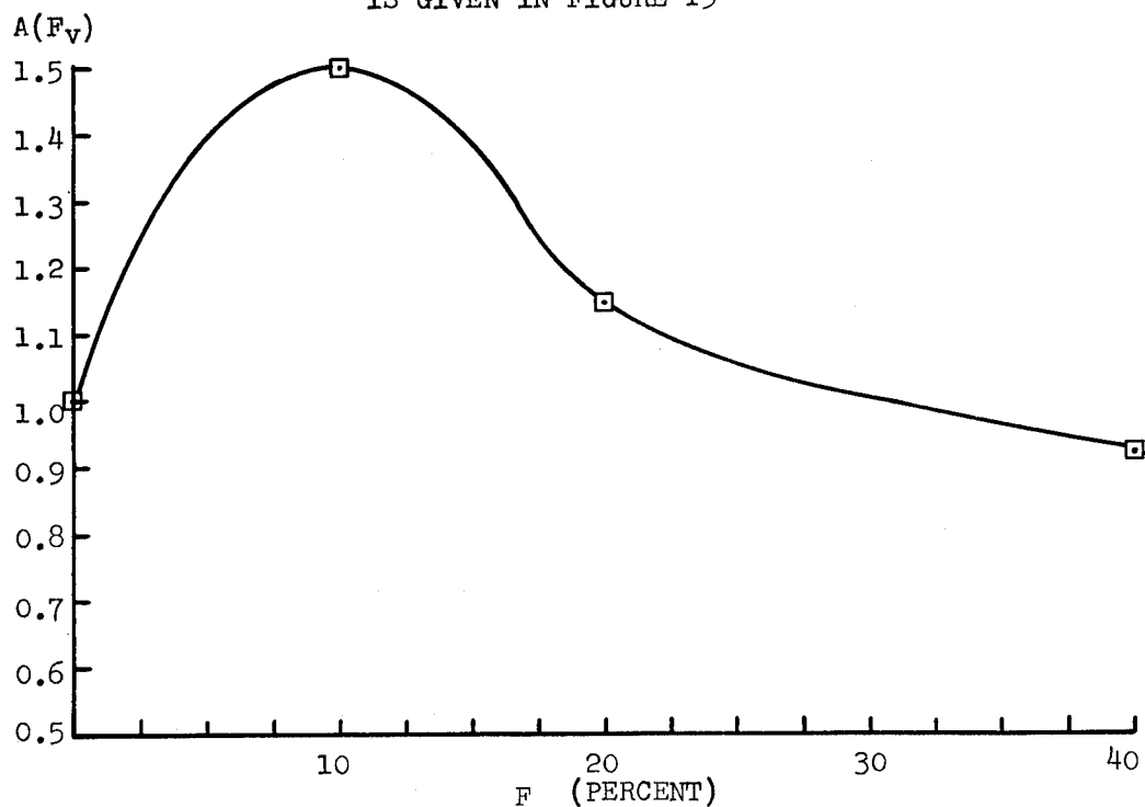
Figure 16 THE FUNCTION A(F_v) = \frac{1 - F_v}{Q(F_v)} WHERE Q(F_v)
