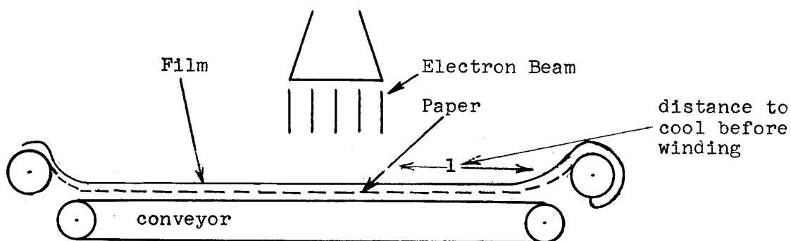
Figure 41 SCHEMATIC DIAGRAM OF CONTINUOUS FILM IRRADIATION
