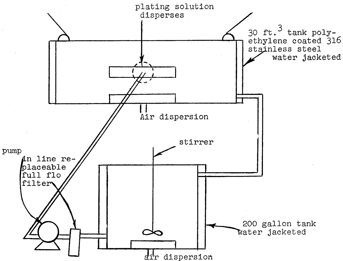
Figure 45 - SCHEMATIC DIAGRAM OF PLATING BATH SYSTEM
