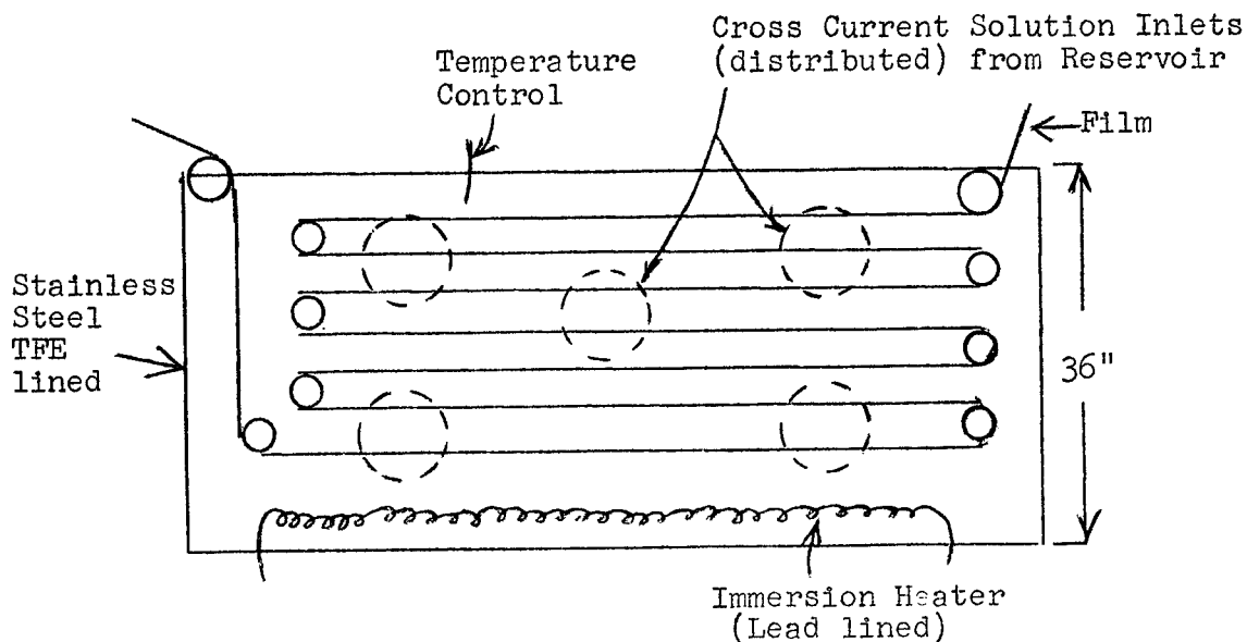
Figure 43 CONDITIONER BATH
