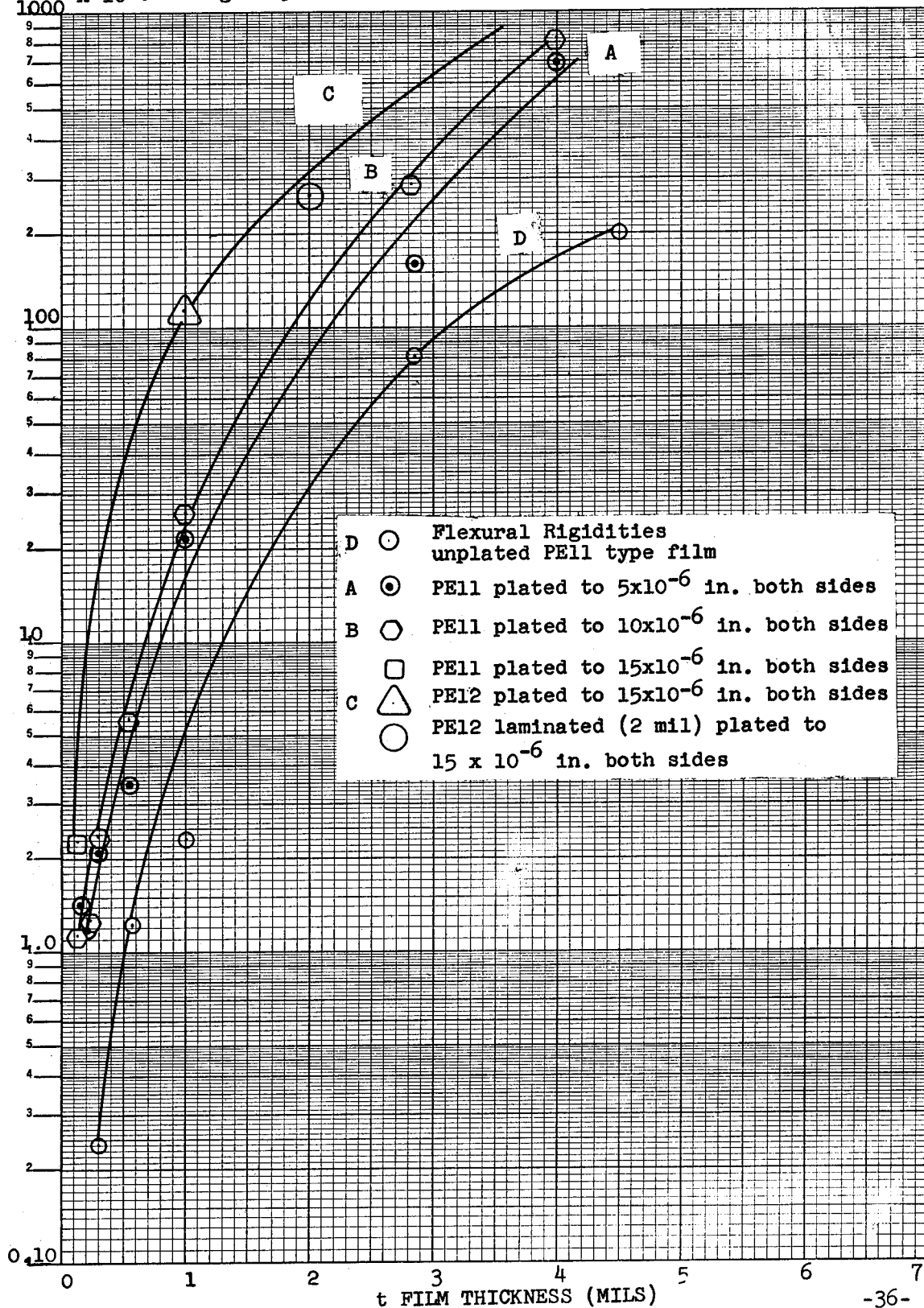
Figure 5 EXPERIMENTAL FLEXURAL RIGIDITIES
