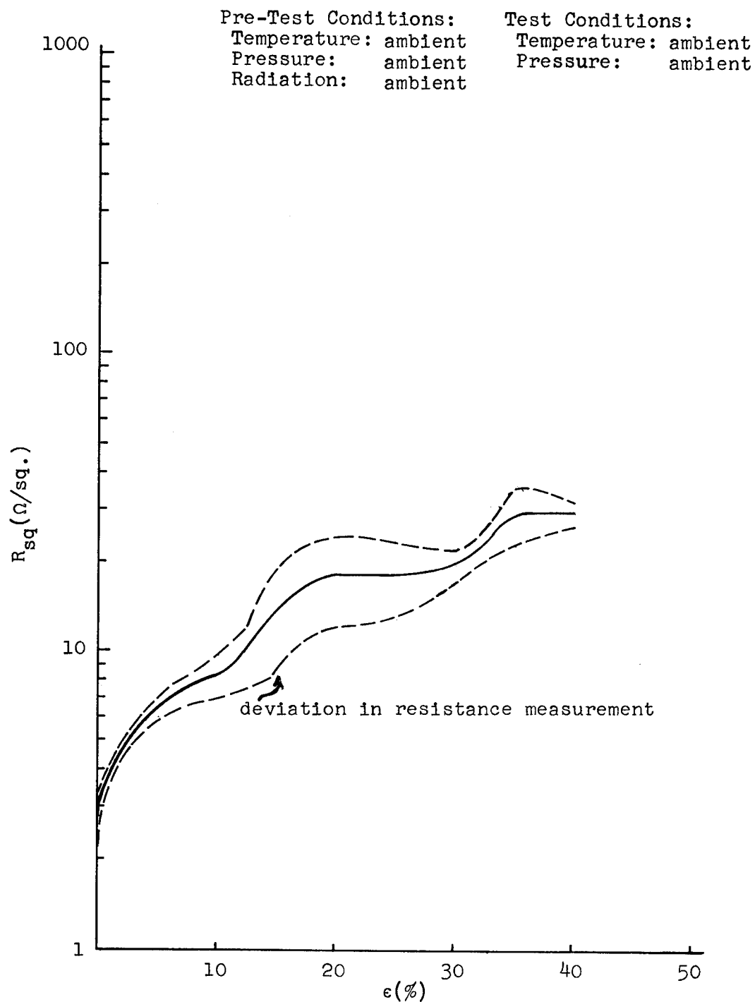
Figure 55 SURFACE RESISTANCE VS. STRAIN FOR COMPLETED MATERIAL (in 90° Direction)
