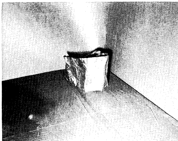
Cylinder # 2 After Test Height 6" Diameter 7.5"
