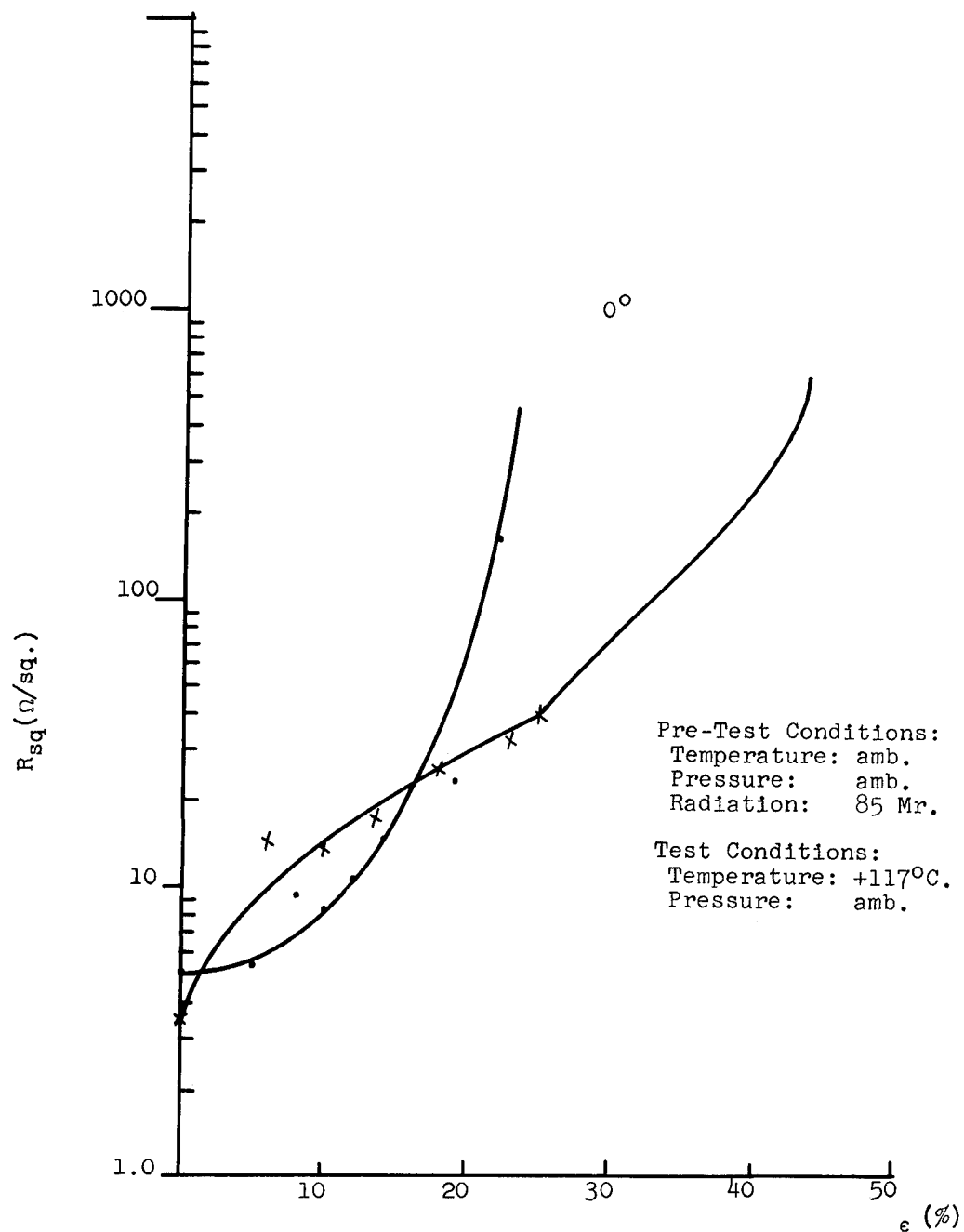
Figure 62 SURFACE RESISTANCE VS. STRAIN FOR COMPLETED MATERIAL (in 0° Direction)
