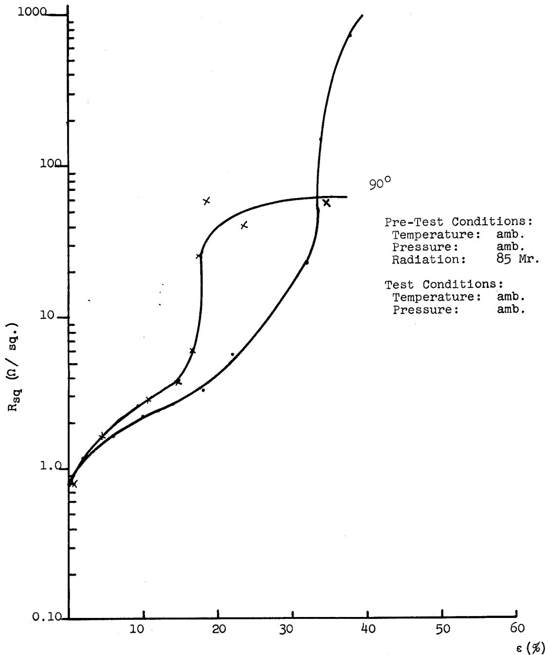
Figure 59 SURFACE RESISTANCE VS. STRAIN FOR COMPLETED MATERIAL (in 90° Direction)
