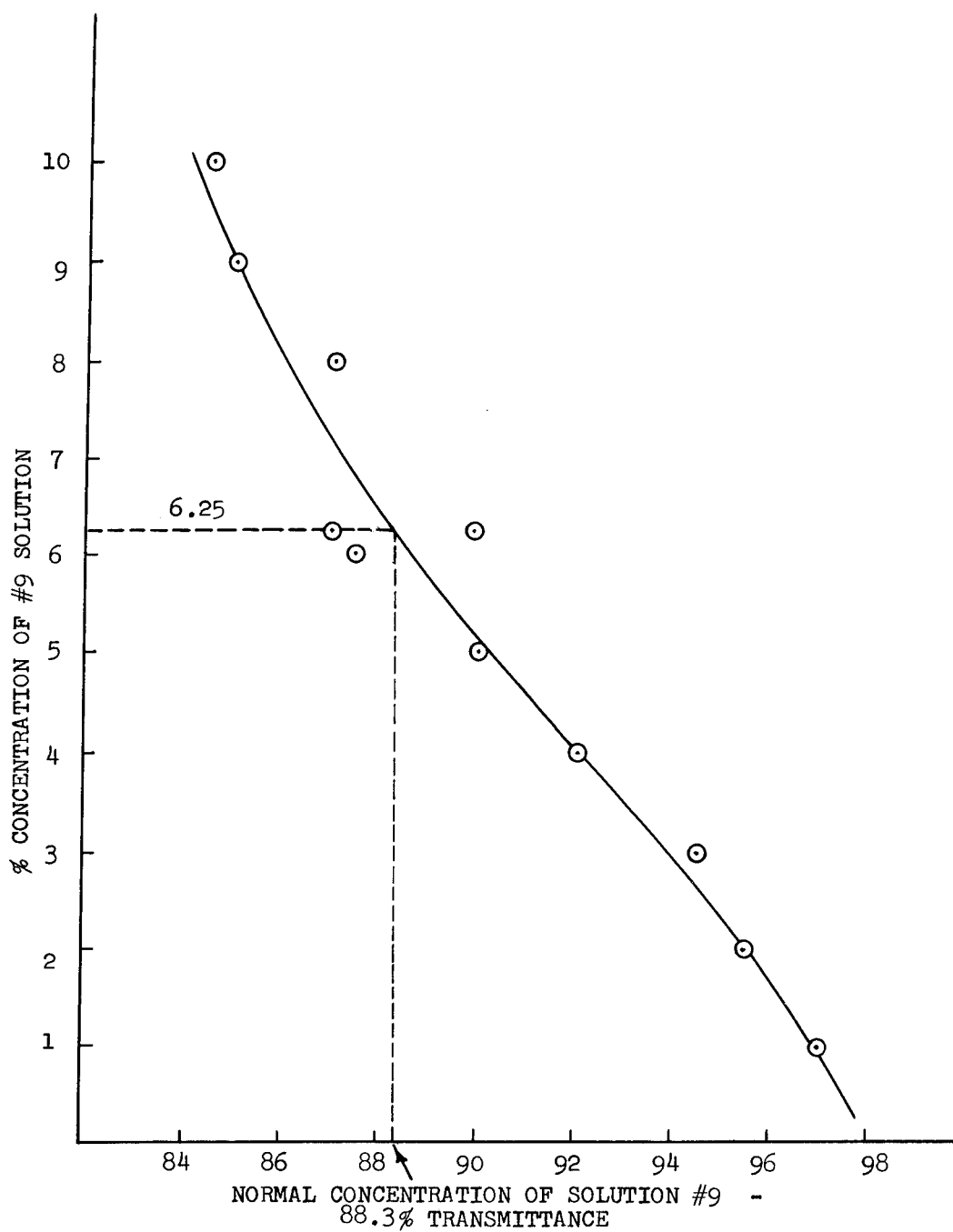
Figure 1 ACTIVATOR CONCENTRATION VS. TRANSMITTANCE at 535 \times 10^{-9} cm. and 24^{\circ}\text{C} . wavelength
