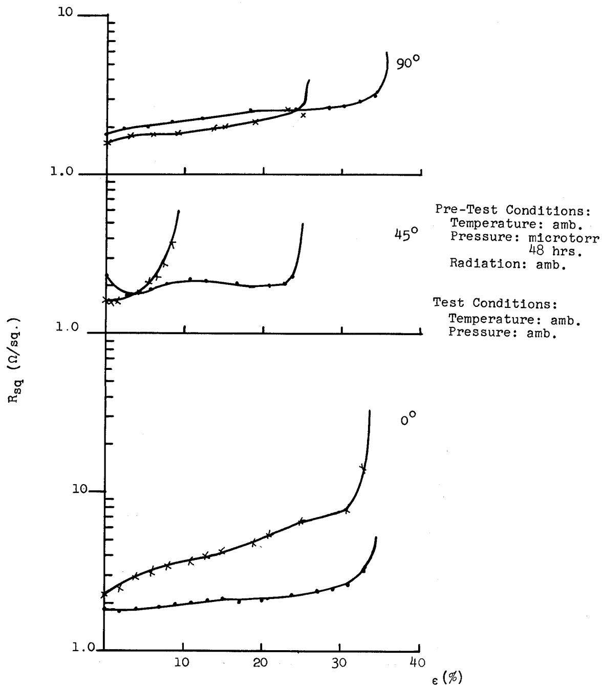
Figure 57 SURFACE RESISTANCE VS. STRAIN FOR COMPLETED MATERIAL (in 0°, 45° and 90° Directions)
