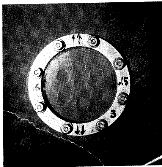
Figure 2 PERFORATED 0.15 MIL SEA SPACE FILM AFTER ANNEALING
