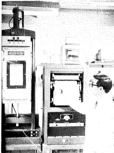
Figure 2 INSTRON TABLE MODEL TENSILE TESTER Left: Cross-head and jaw assembly enclosed in Missimers Constant Temperature Oven Right: Recorder for measurement of stress strain relationship
