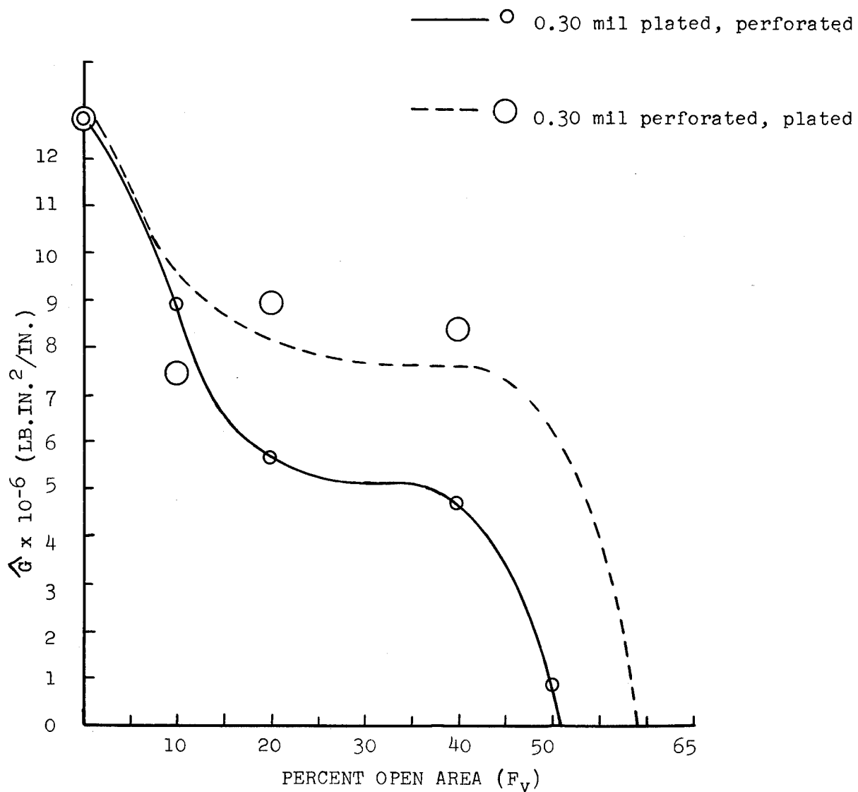
Figure 8 FLEXURAL RIGIDITY OF PERFORATED 0.30 MIL STANDARD DENSITY POLYETHYLENE FILM VS. PERCENT OPEN AREA (Plated to 15 \times 10^{-6} inches on both sides)
