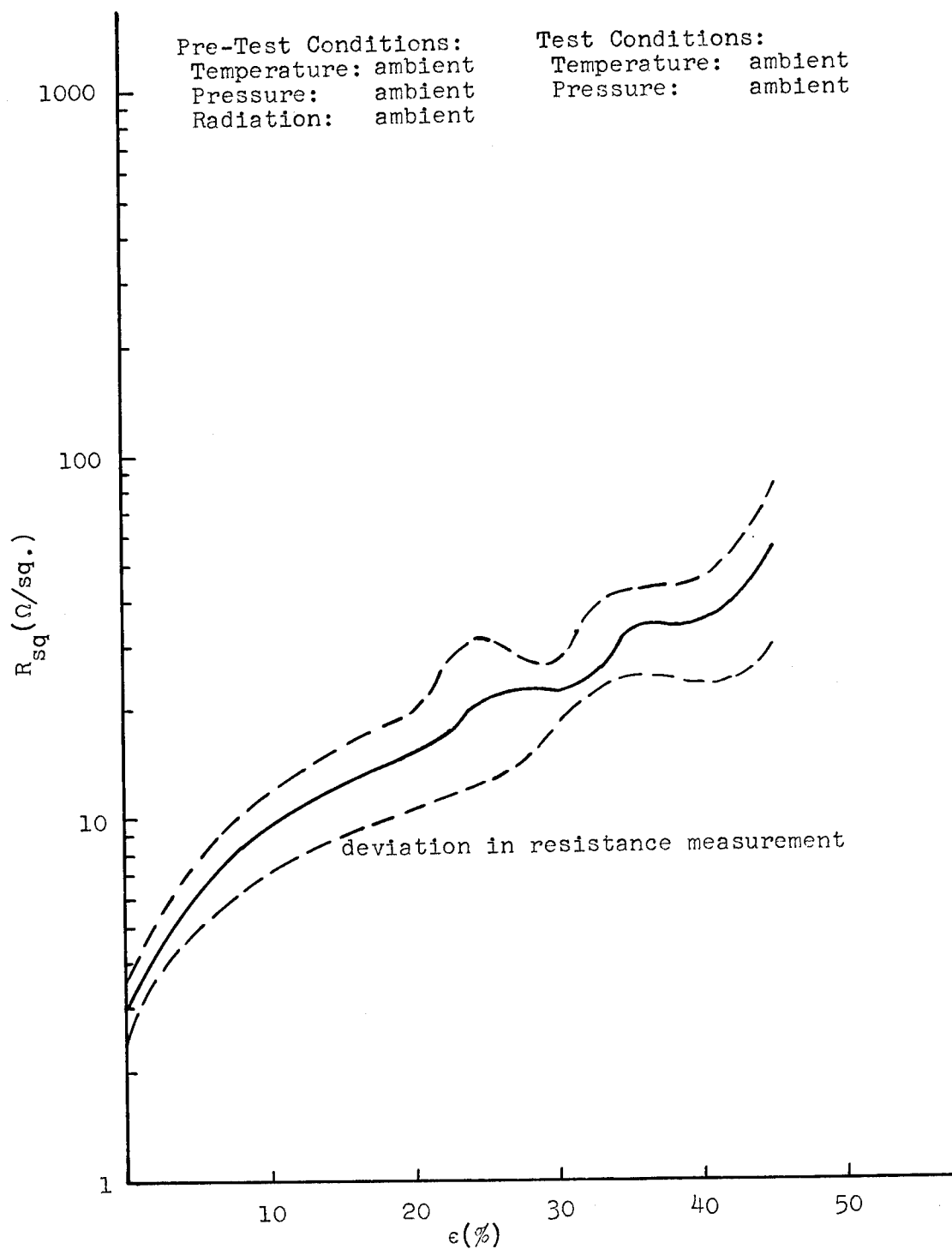
Figure 53 SURFACE RESISTANCE VS. STRAIN FOR COMPLETED MATERIAL (in 0°Direction)
