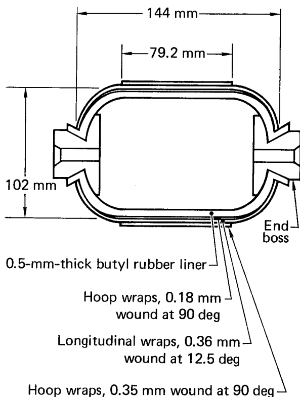
Fig. 24. Dimensions of the 10.2-cm-diameter pressure vessel (volume = 950 \pm 8 \text{ cm}^3 ): thicknesses of coating are not shown.
