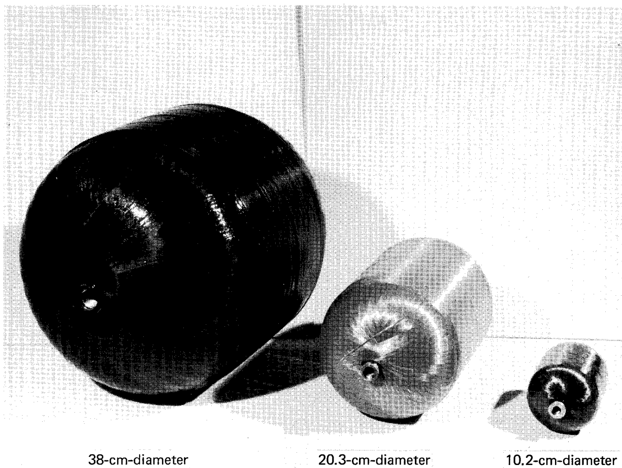
Fig. 36. Photograph of the 10-cm-diameter, 20-cm-diameter, and 38-cm-diameter pressure vessels tested in this study.
