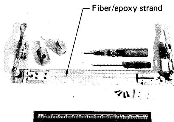
Fig. 21. Clamping arrangement for testing the fiber strengths of epoxy-impregnated strands.
