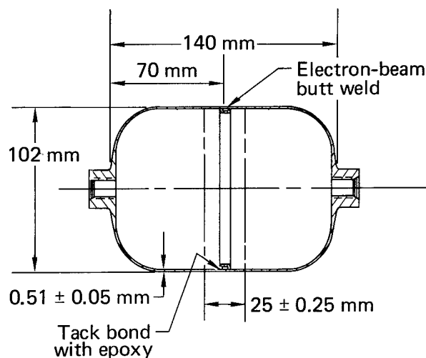
Fig. 9. Design of the metal mandrel used to wind the 10.2-cm-diameter pressure vessels.
