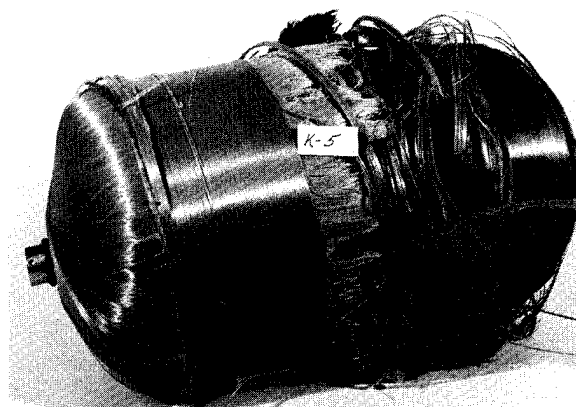
Fig. 38. Photograph of the hoop failure of the K-5, 20.3-cm-diameter pressure vessel.
