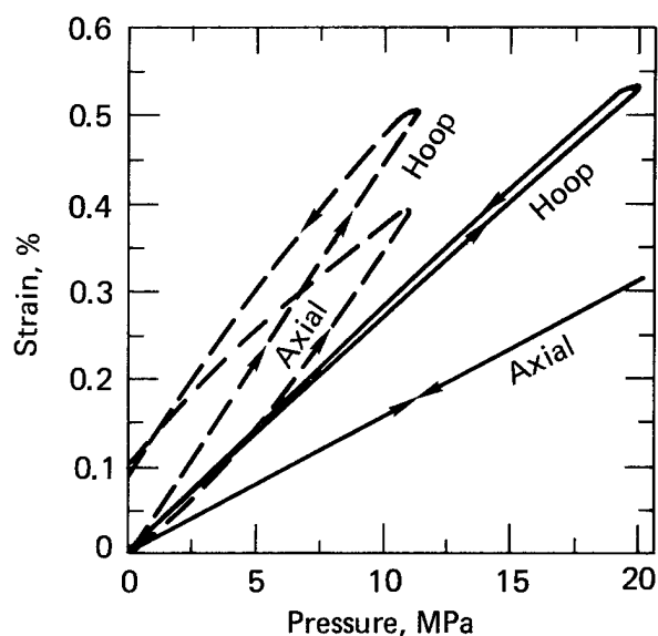
Fig. 11. Typical pressure vs strain curves during the first load cycle to 50% of the expected failure pressure of titanium-lined and aluminum-lined pressure vessels: solid curves denote titanium-lined vessel results, dashed curves denote aluminum-lined vessel results.
