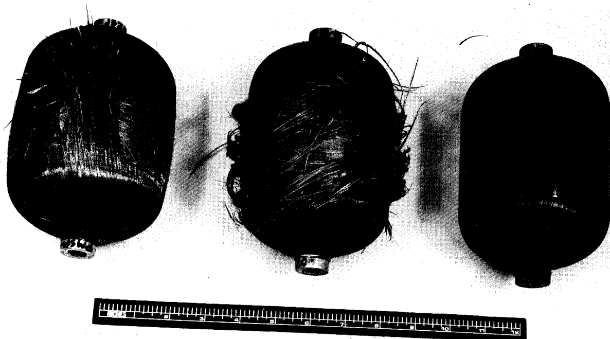
Fig. 32. Photograph of two typical hoop failed vessels (a, b) and a typical unfailed pressure vessel (c).
