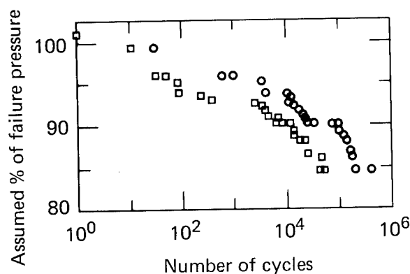
Fig. 34. Fatigue life at assumed peak cyclic stress levels for 10.2-cm-diameter pressure vessels: \circ denotes failure of vessels under sinusoidal cycling, \square denotes failure of vessels under rectangular cycling. Vessels that failed at less than one cycle are plotted at one cycle.
