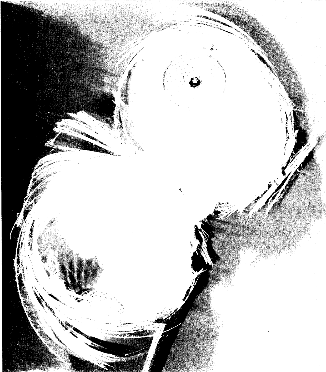
Fig. 44. Photograph of an ABS-lined pressure vessel wound with the double pattern overwind showing the hoop mode of failure (vessel failed at 36.8 MPa).
