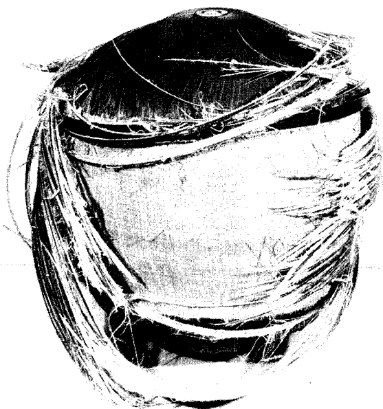
Fig. 39. Photograph of the hoop failure of a 38-cm-diameter, Kevlar 49/epoxy pressure vessel.
