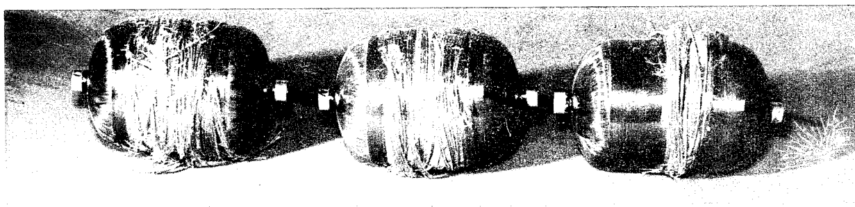
Fig. 23. Typical pressure vessel failures: from left to right, vessels made with epoxy systems 1, 4, and 7.
