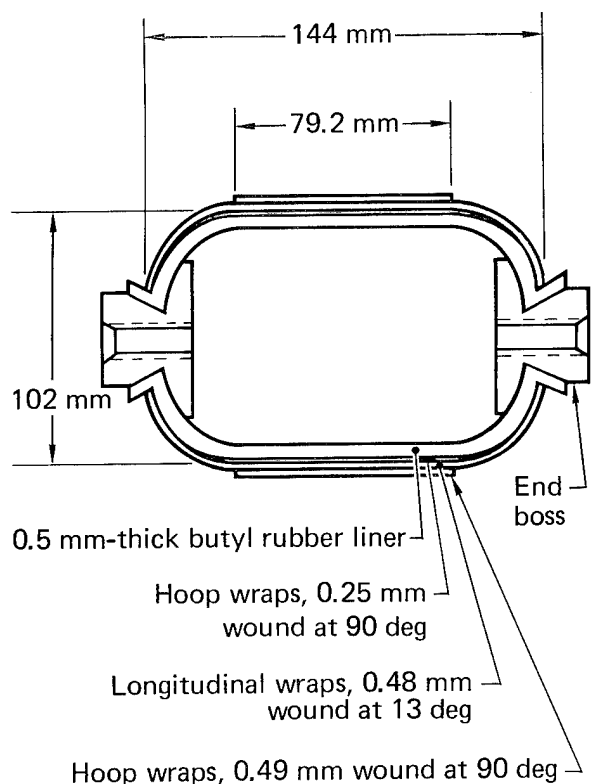
Fig. 7. Typical dimensions of a 10.2-cm-diameter, filament wound pressure vessel (volume = 950 \pm 8 \text{ cm}^3 ).
