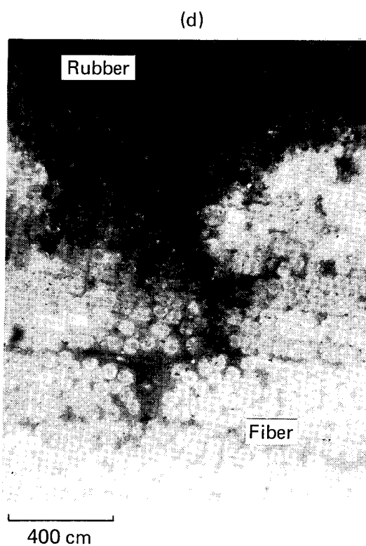
Fig. 43. Photomicrographs of four wall sections illustrating some of the problems with the liners: (a, b) 20.3-cm 3 -diameter vessels with voids, (c, d) 10.2-cm-diameter vessels with rubber migration.
