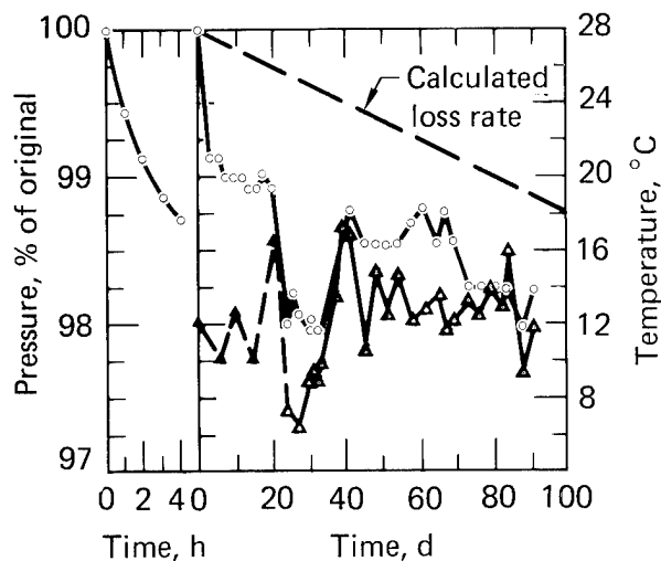
Fig. 26. Percentage of original nitrogen pressure vs time and ambient air temperature vs time for vessel 1: ○ = gage pressure, ▽ = temperature as read at thermometer near Heise gage, ▲ = temperature as estimated from outside air temperature 2 mi away.
