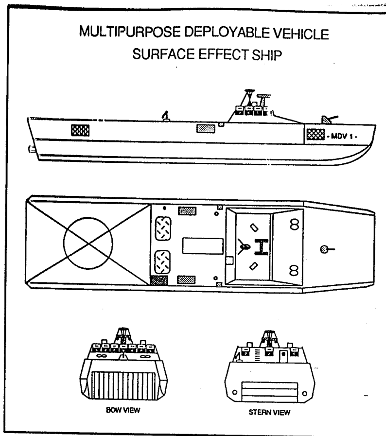
Figure 5. Multi-Mission Deployable Vehicle, Surface Effect Ship (MDV-SES)
