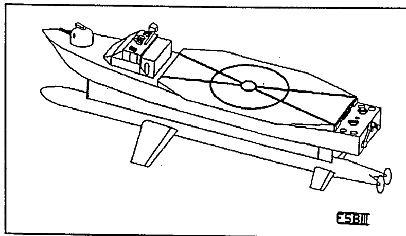
Figure 6. Multi-Mission Deployable Vehicle, Hybrid Hydrofoil (MDV-HH)
