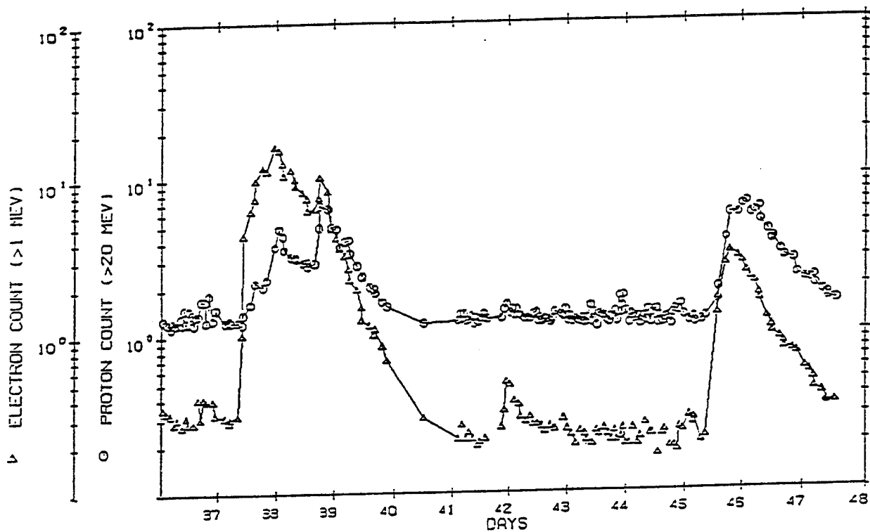
Figure 3a. Proton and electron count rates in DMSP/F7 SSJ* instrument during solar particle events SOLAR GEOPHYSICAL DATA: FEB 05-17, 86
