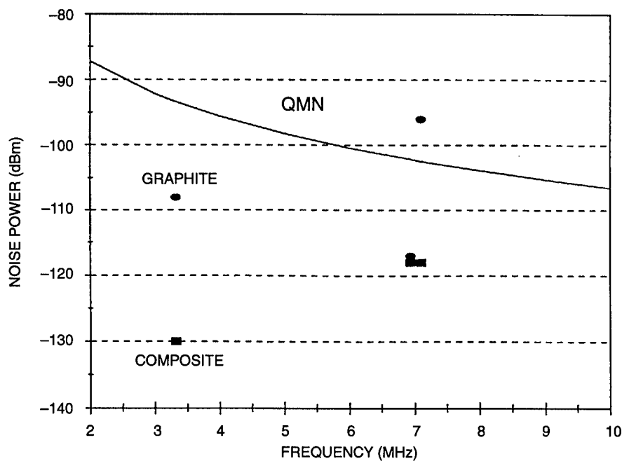
Figure 6. Noise power results for measurement run #2.
