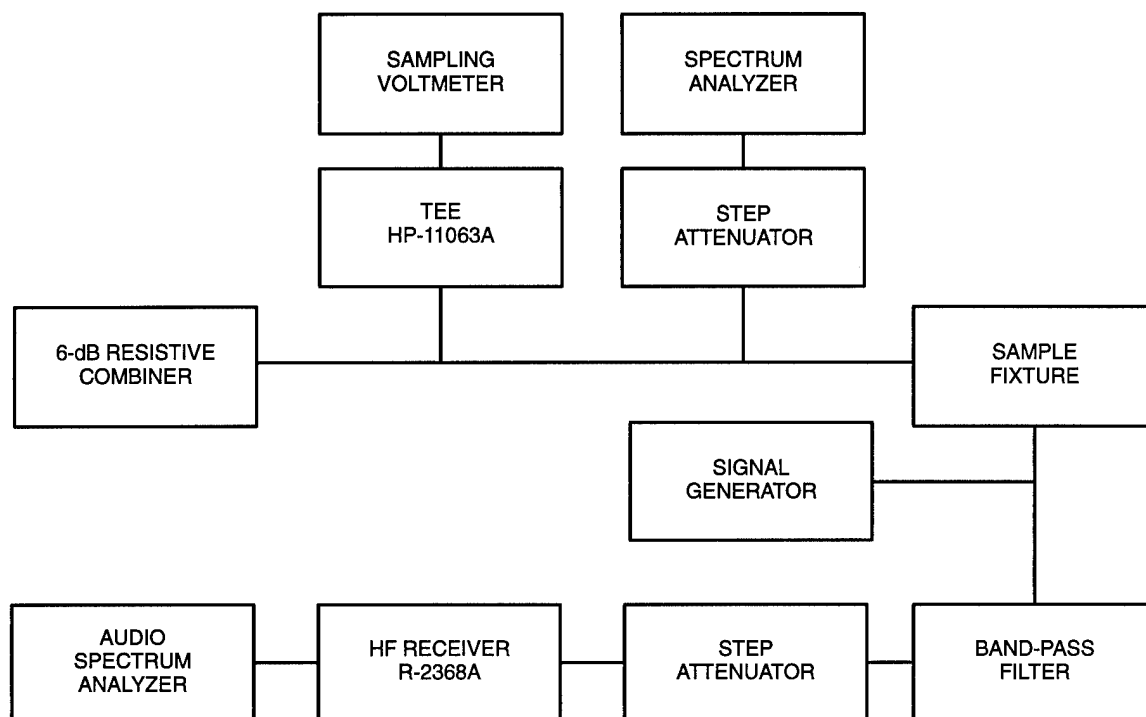
Figure 3. Test setup for measurement of IMI amplitude, continued.
