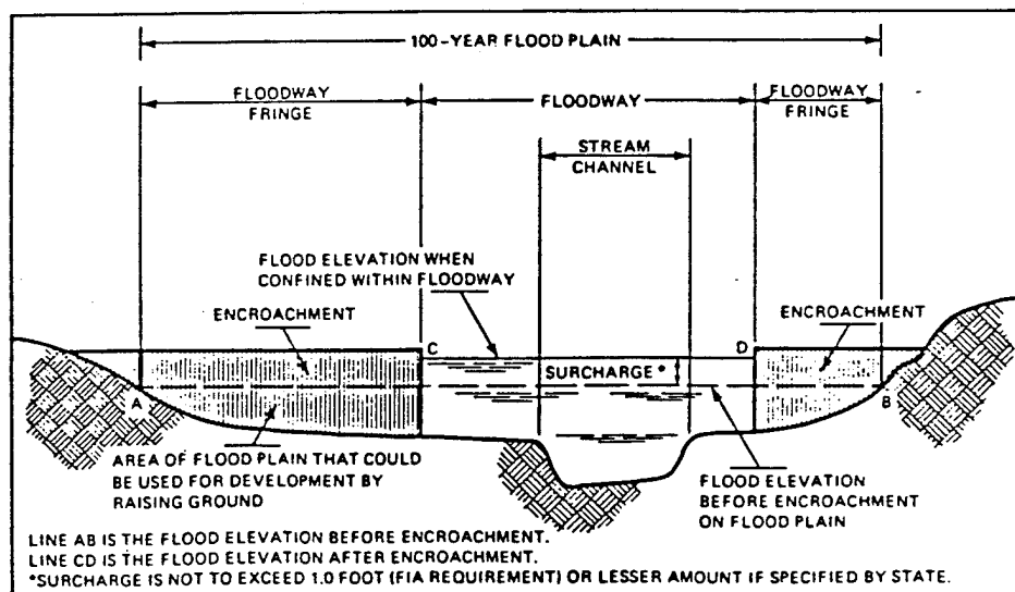
Figure 2 - Floodway Schematic
