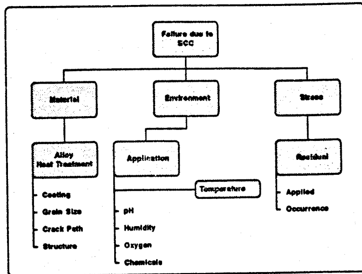
Fig. 4 Inference tree of SCC factors considered by Failure Analyst.
