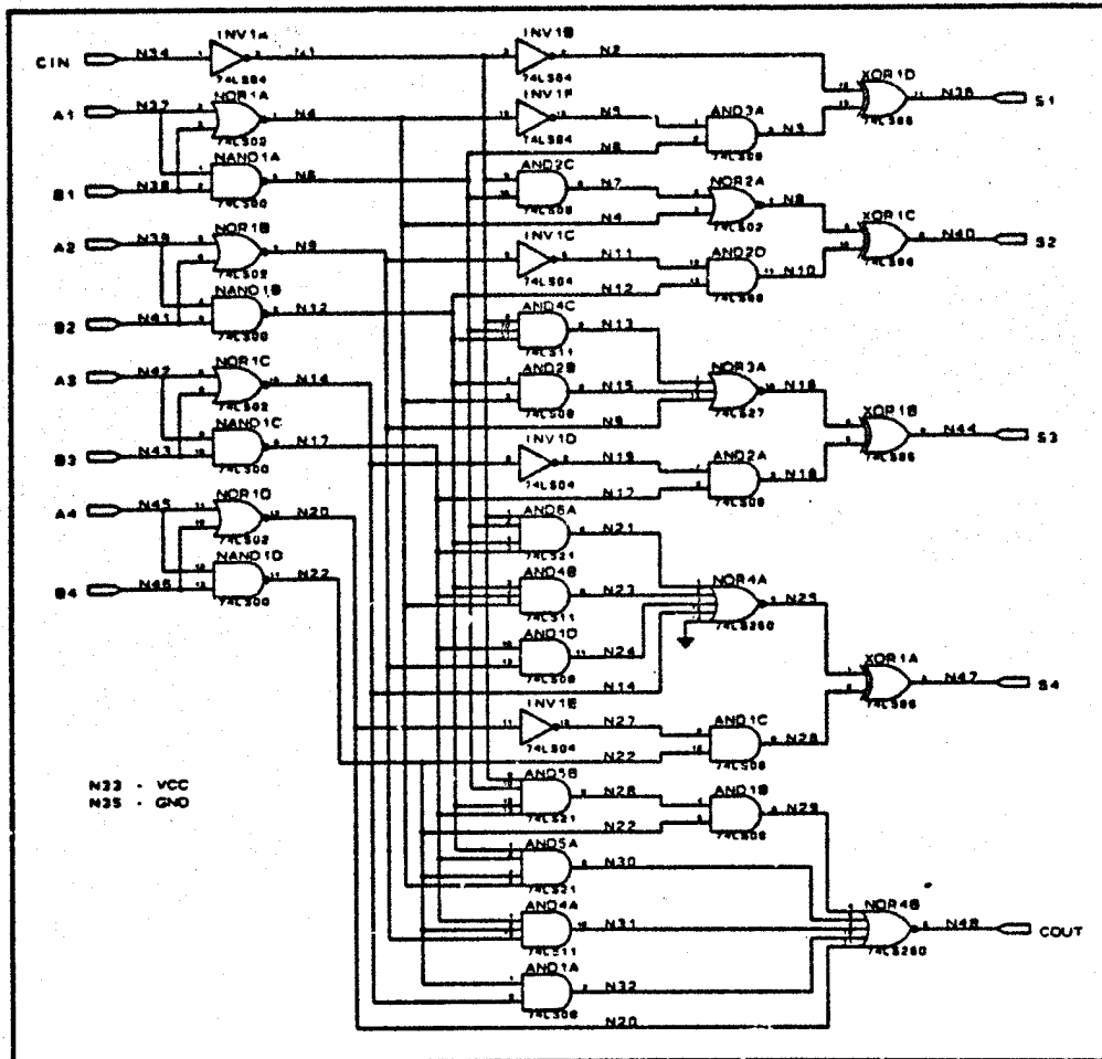
Figure 5: 4-Bit Full Adder test circuit
