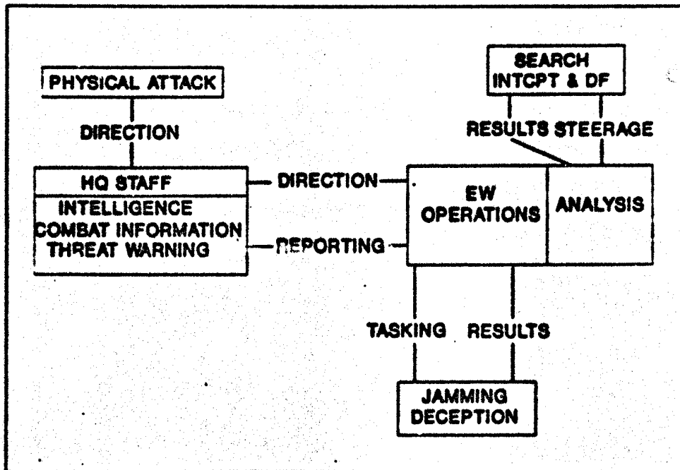
Figure 2 - EW process
