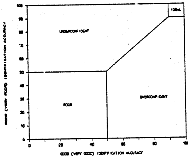
Figure 3: A Method of Evaluating Confidence Factor Models
