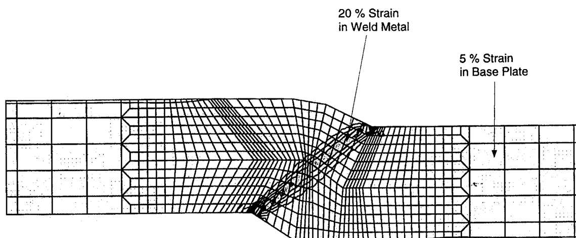
Misaligned Welded Joint HSLA-100, 100S-1 Weld 3 mm Offset
