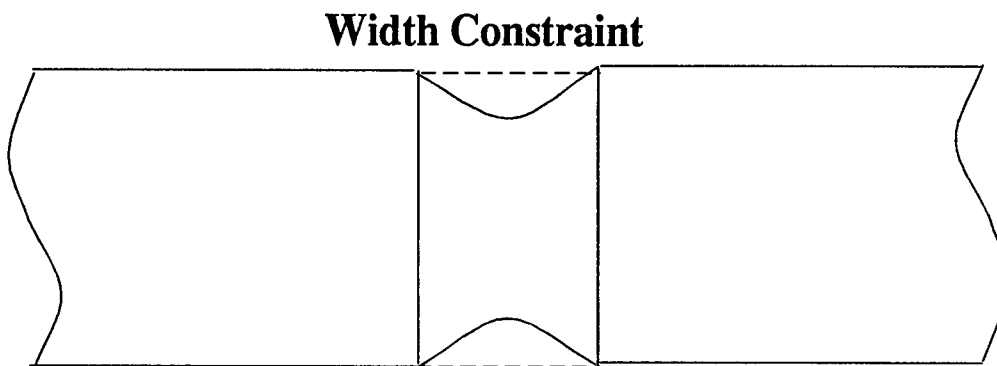
Figure 2-2 Weld Deformations that Lead to the Development of Constraint.
