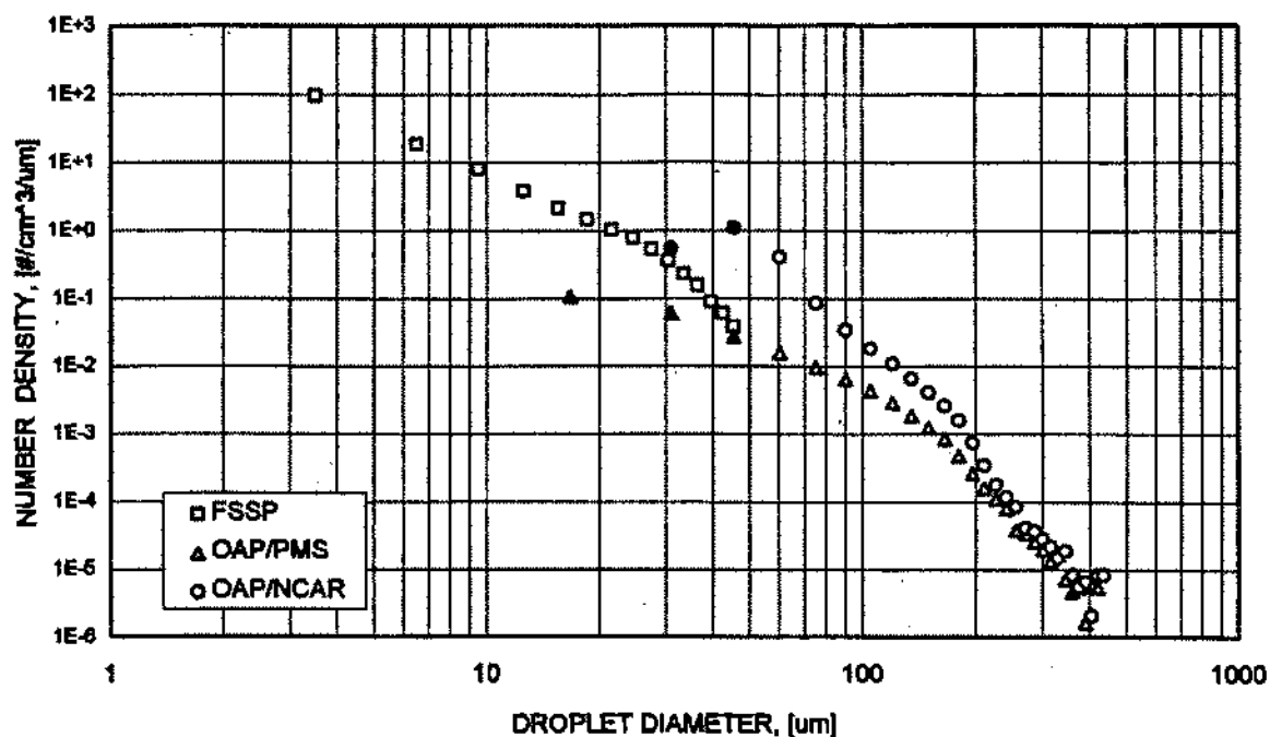
a). Number density distribution (air pressure = 6 psig, water pressure = 36 psig)
