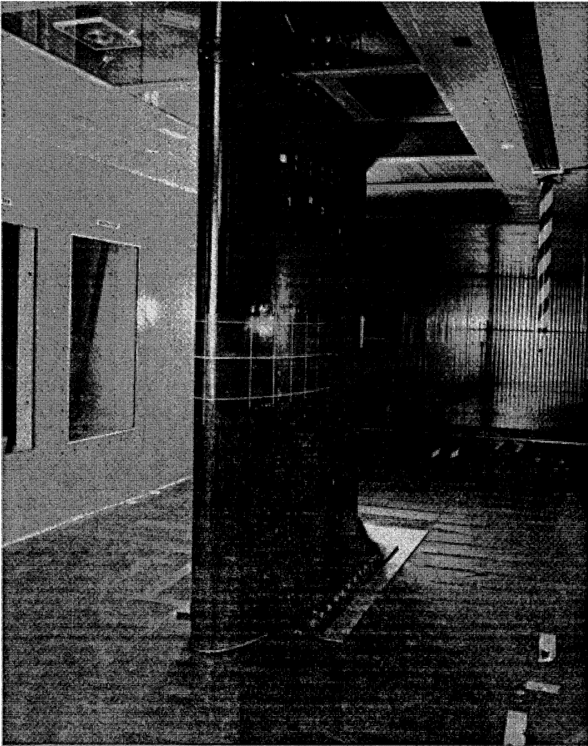
Figure 3 – Twin Otter wing section installed in Icing Research Tunnel.
