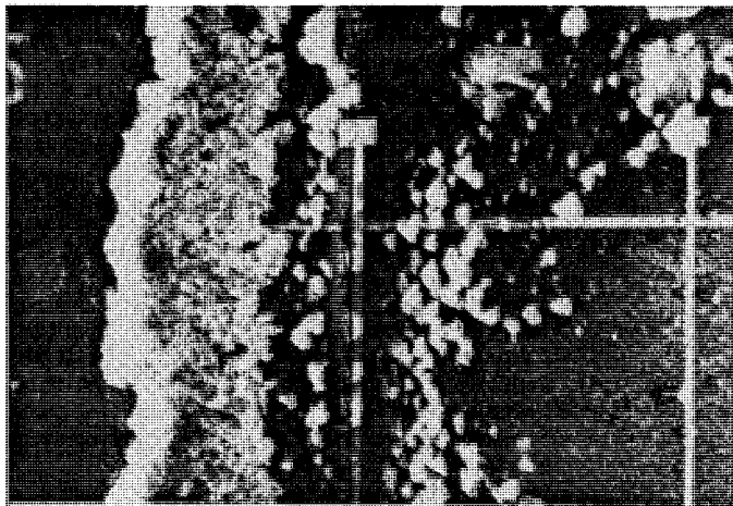
c). Run 5, T_t = 28^\circ\text{F} , V = 125 mph
