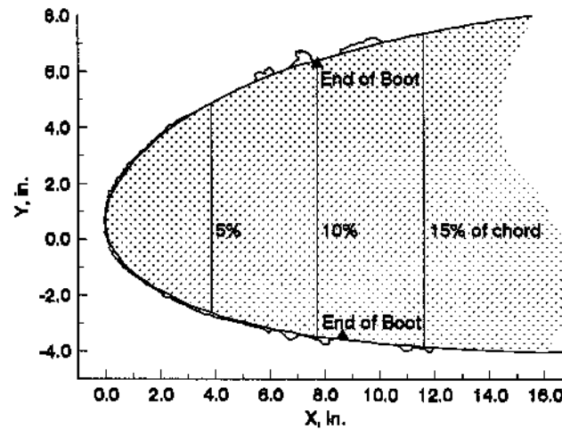
c). Run 43a-r2, STA 36 tracing
