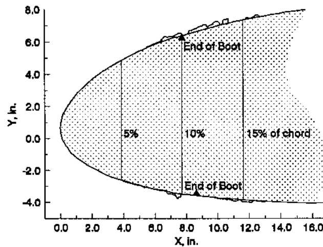
c). MVD = 180\mu m , LWC = 1.36 g/m^3
