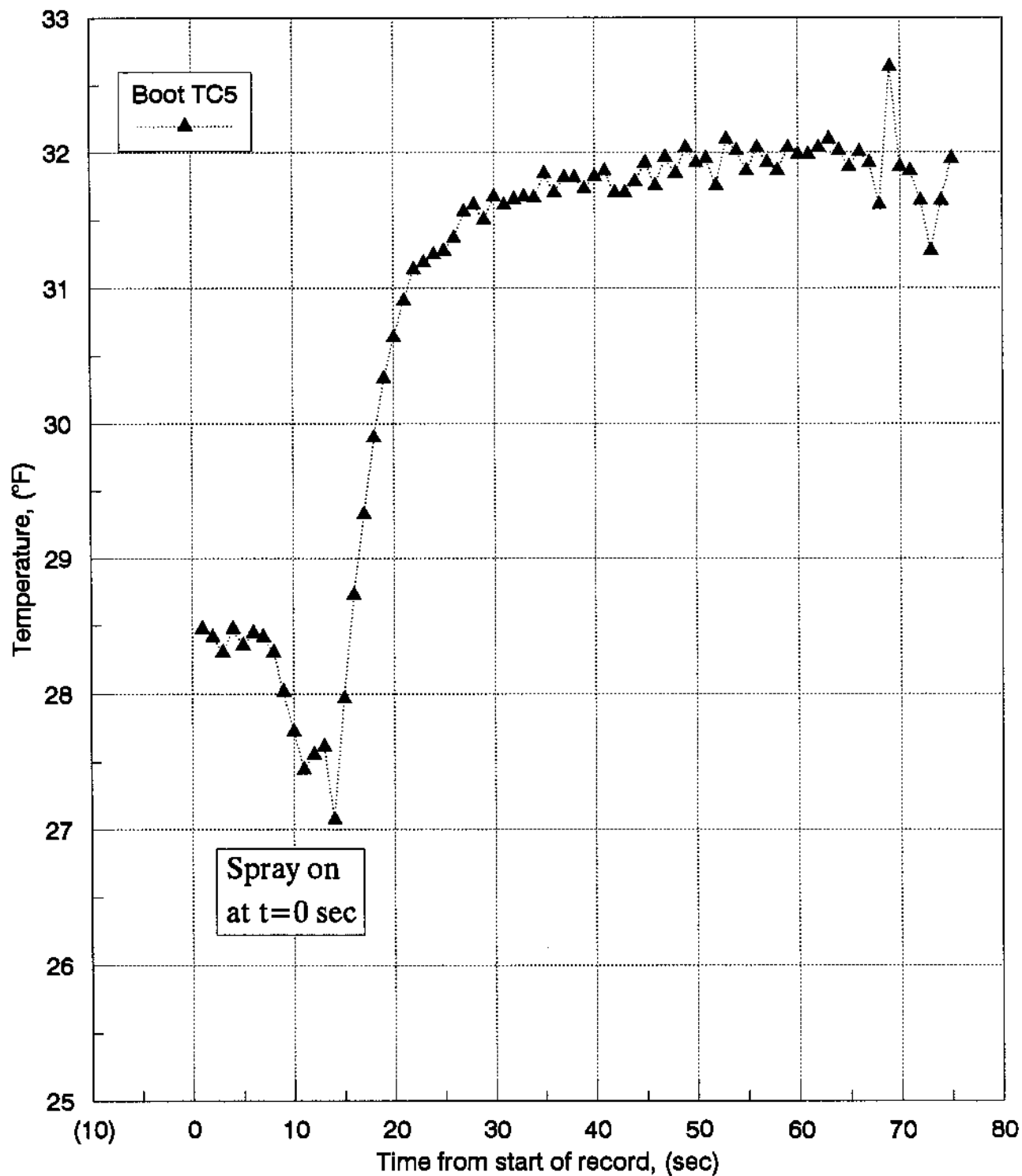
Figure 7 - Leading-Edge temperature after initiation of large droplet icing spray. ( T_t=28^\circ\text{F} , V=195 mph, MVD=160\mu\text{m} , LWC=0.82\text{ g/m}^3 , AOA=0^\circ , Flap=0^\circ )
