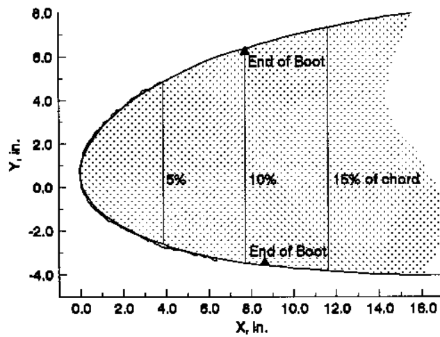
a). MVD = 40\mu m , LWC = 0.76 g/m^3
