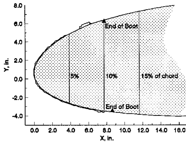
b). MVD = 88\mu m , LWC = 0.85 g/m^3
