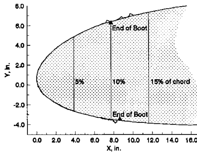
c). Run 43-r3, STA 36 tracing
