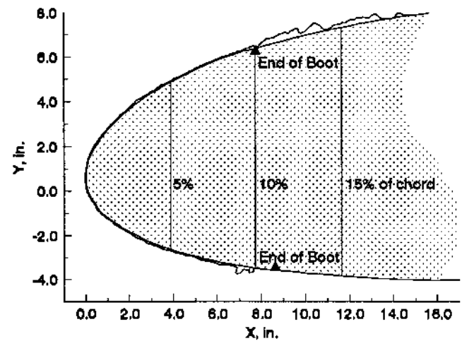
Figure 13 - AOA effect.
