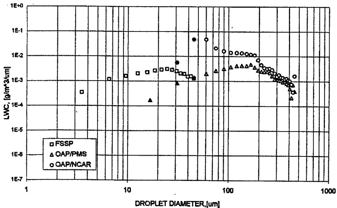
d). LWC distribution (air pressure = 5 psig, water pressure = 55 psig)
