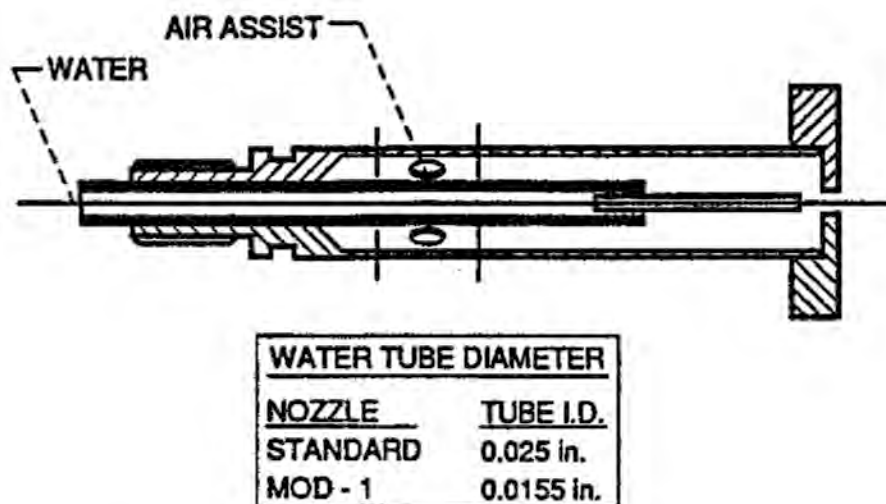
Figure 2 – Icing Research Tunnel spray bar nozzle.
