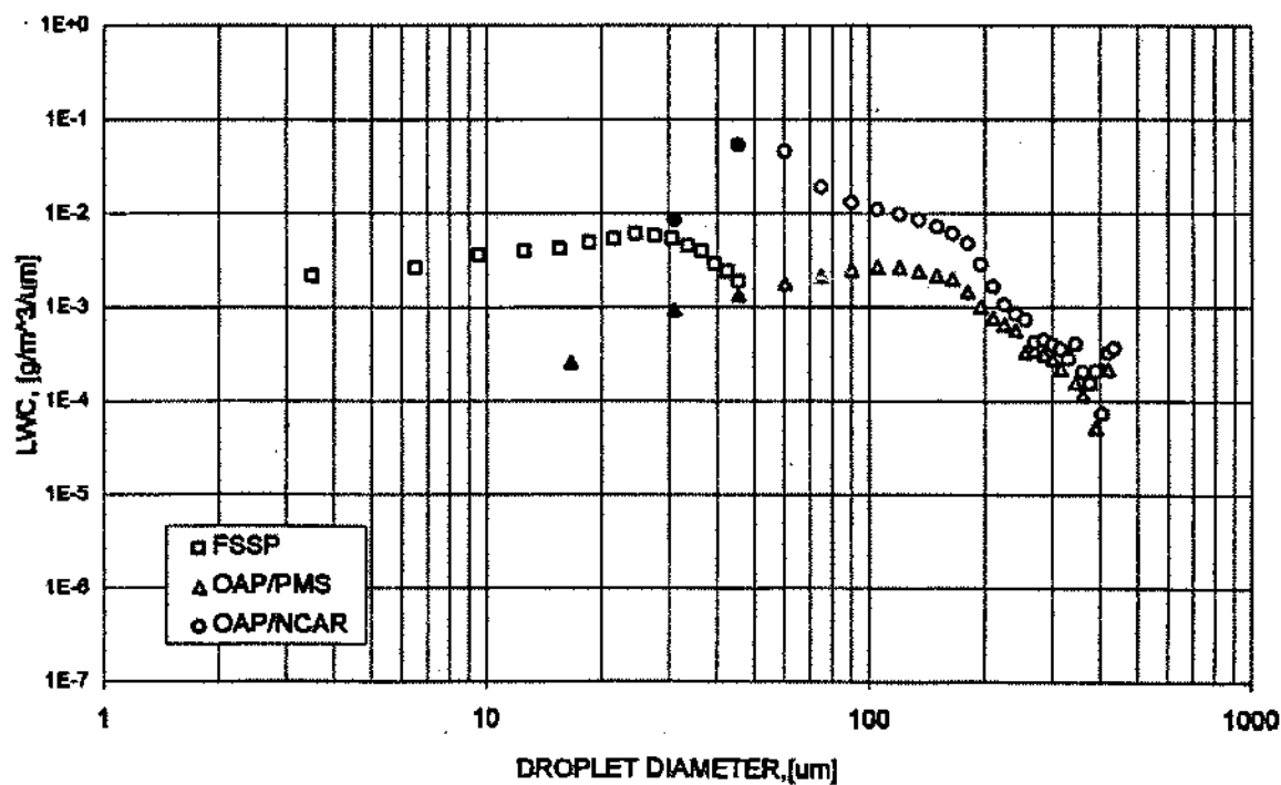
b). LWC distribution (air pressure = 6 psig, water pressure = 36 psig)
