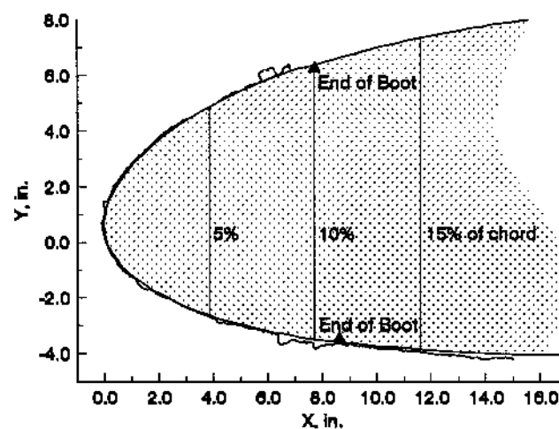
c). Flap = 20°
