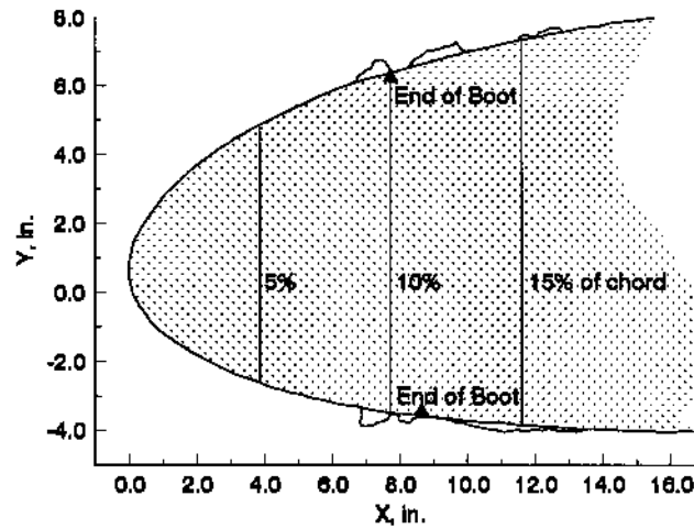
b). Run 43a-r, STA 36 tracing
