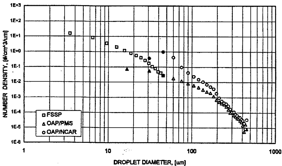
c). Number density distribution (air pressure = 5 psig, water pressure = 55 psig)
