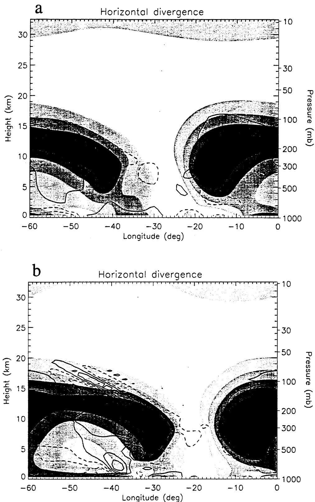
FIG. 6. Longitude–height cross section of horizontal velocity divergence at 55° latitude on consecutive days: (a) day 9; (b) day 10; (c) day 11; (d) day 12. Contour interval is 10^{-5} \text{ s}^{-1} . Windspeed superposed as in Fig. 5 with contour interval 10 \text{ m s}^{-1} .
