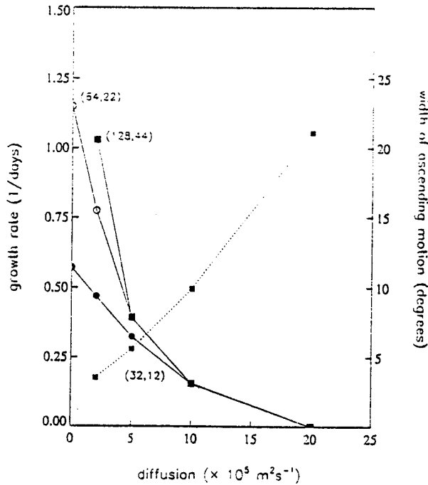
Fig. 1. CISK growth rates in the five-level model as a function of diffusion for q = 8 \text{ g kg}^{-1} . Solid circles, open circles, and squares denote simulation with (M, N) = (32, 12) , (64, 22) , and (128, 44) respectively. The e -folding width of ascending motion is shown by the dashed line for (M, N) = (128, 44) .
