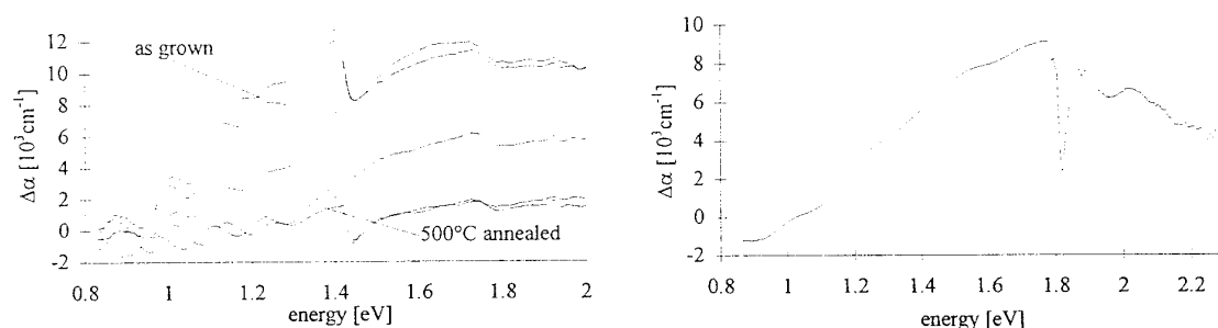
Fig.2 Absorption coefficient change \Delta\alpha due to annealing a) relative to the 600°C annealed LT-GaAs sample and b) relative to the 600°C annealed LT- \text{Al}_{0.3}\text{Ga}_{0.7}\text{As} sample.
