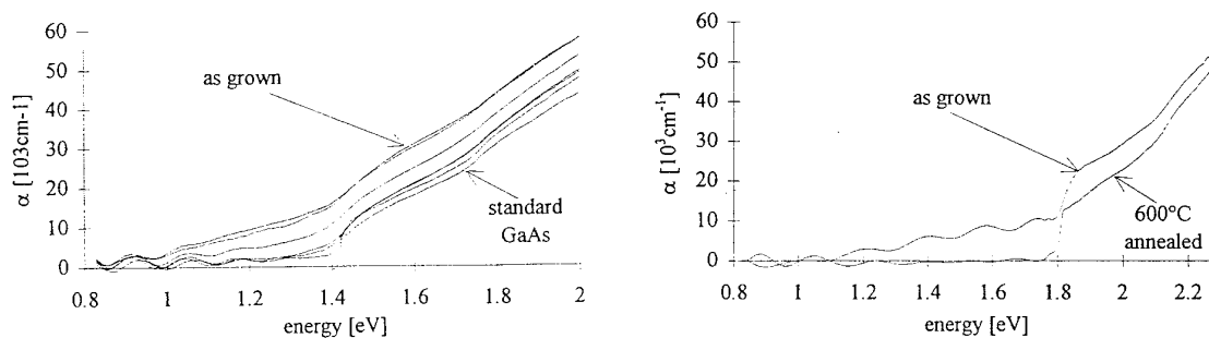
Fig.1 Absorption coefficient \alpha of a) as grown, 400°C, 430°C, 470, 500°C and 600°C annealed LT-GaAs samples and of b) as grown and 600°C annealed LT- \text{Al}_{0.3}\text{Ga}_{0.7}\text{As} .
