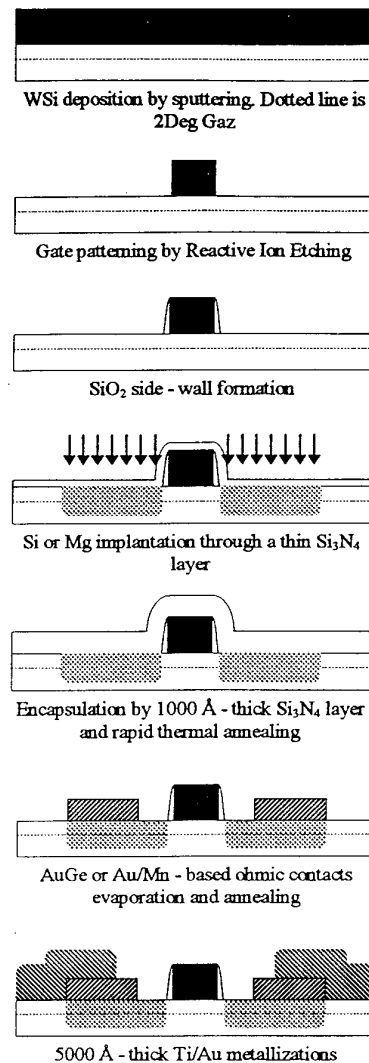
Figure 2 : Complementary process steps
