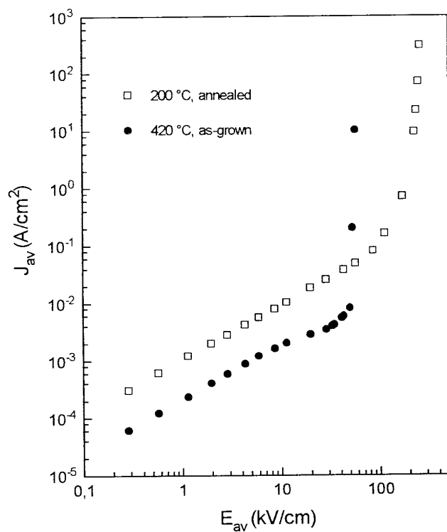
Fig. 2. Current density vs electric field for 420 °C grown GaAs layers and LT GaAs layers ( T_g = 200 °C).
