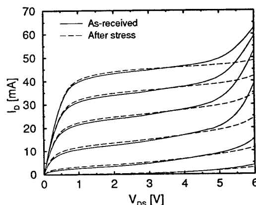
Figure 1: Output characteristics of one of the devices under test. Continuous line: I_D in an as-received device. Dashed lines: I_D after 30 minutes of stress at V_{DS} = 6\text{ V} , V_{GS} = 0 .
