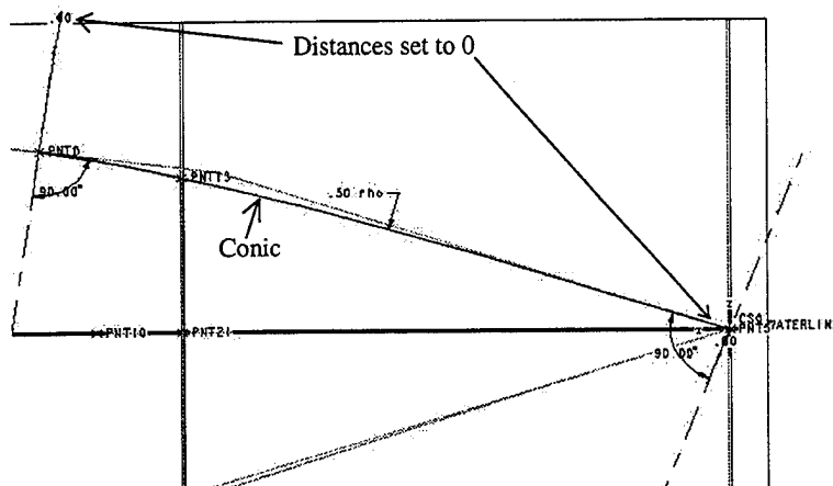
Figure(29) Dimensioned, regenerated conic sketch, values edited 1
