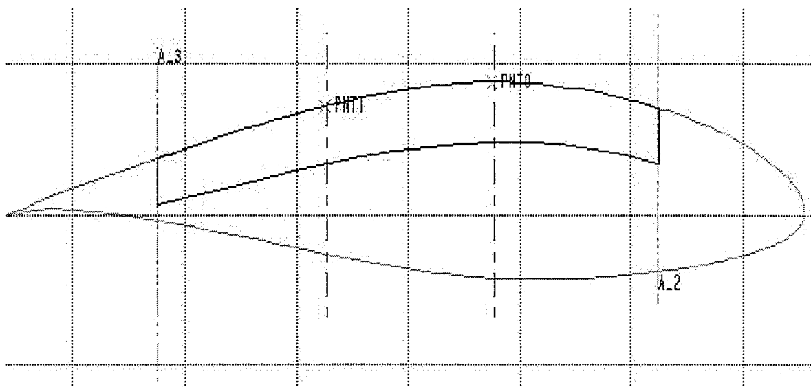
Figure(16) Completed Datum Curve sketch.
