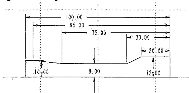
Figure(23) Completed engine sketch.
