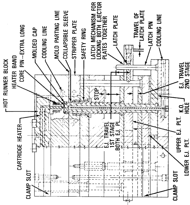
SCHEMATIC HOT RUNNER MOLD ASSEMBLY WITH CENTER GATED PART FIGURE 11 - COLLAPSIBLE CORE
