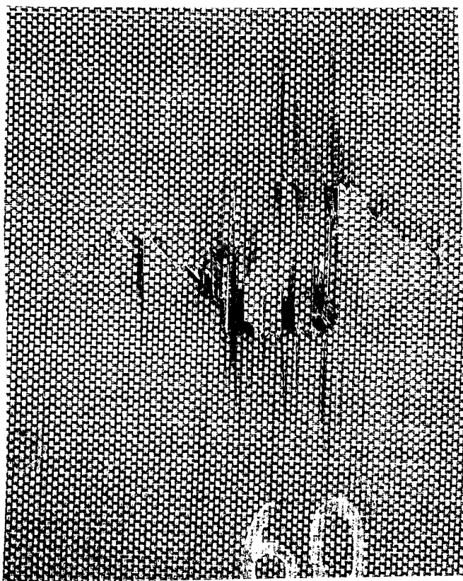
FIGURE 9. VISIBLE IMPACT DAMAGE ON BACK SIDE (0, \pm 45, 90) s 5208 REFERENCE LAMINATE
