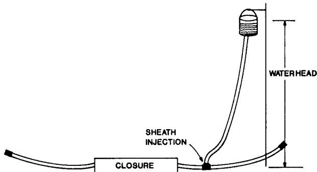
FIGURE 5d. SHEATH INJECTION WATERHEAD TEST
