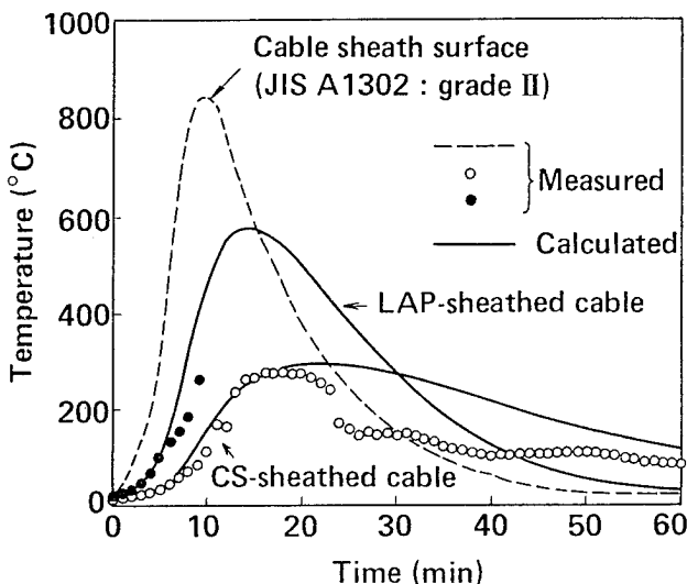
Fig.7 Temperature change at optical unit layer surface.
