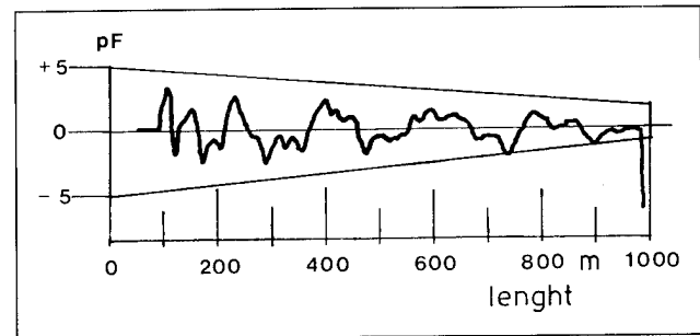
Fig. 10: Distribution of Capacitance Unbalance over a Tail Cable Length
