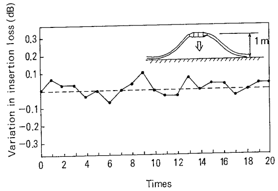
Figure 12. Impact test
