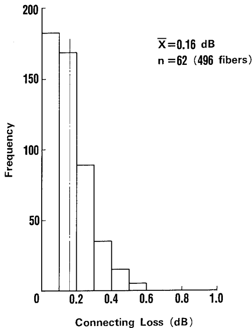
Fig.7 Connecting Loss
