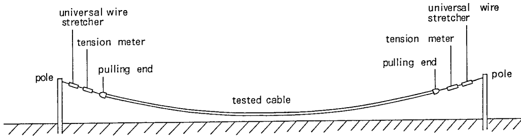
Figure 23 Tensile strength test system
