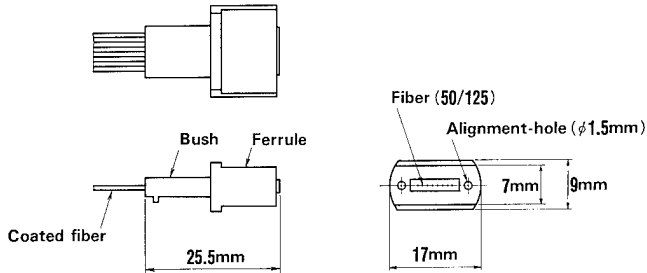
Fig.1 Construction of Multi Fiber Plastic Plug
