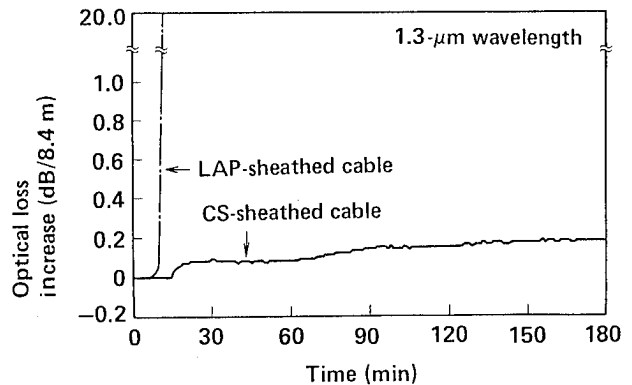
Fig.8 Measured optical loss increase.
