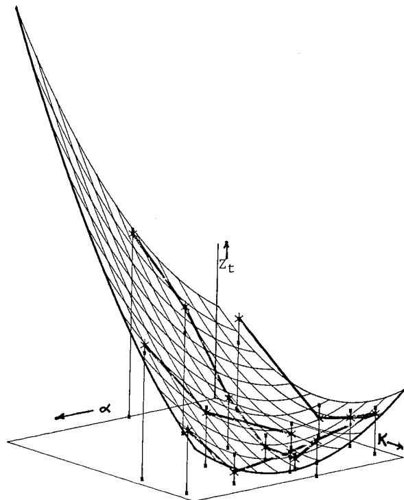
Fig. 2 - Surface fitted to transfer impedance data from Table 1 braid designs, at 10^8 Hz.
