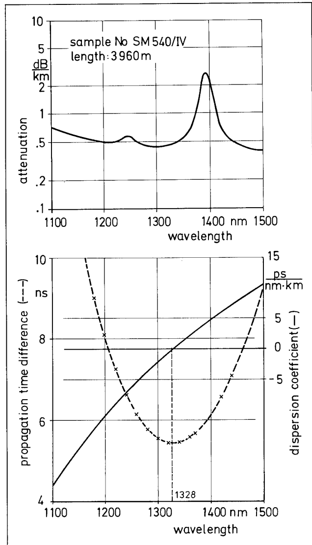
Fig. 5: Attenuation and dispersion of a typical matched cladding SM fibre for the local network
