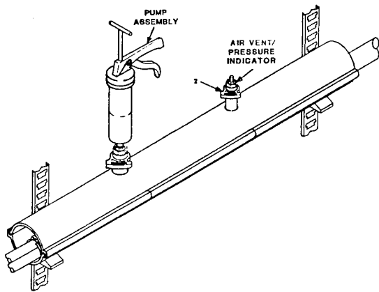
FIGURE 9. PUMPING ENCAPSULANT
