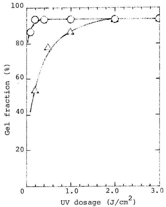
Fig. 2(B) UV dosage dependency of gel fraction of PBA ○; M-PBA, △; PBA
