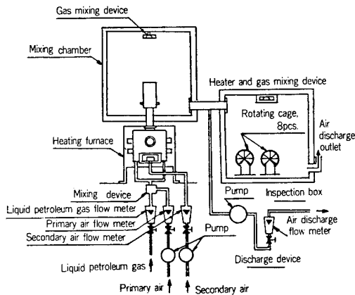
Figure 1 Typical equipment for testing toxicity of the gas, using mice (Notification No.1231 of the Ministry of Construction, Japan)
