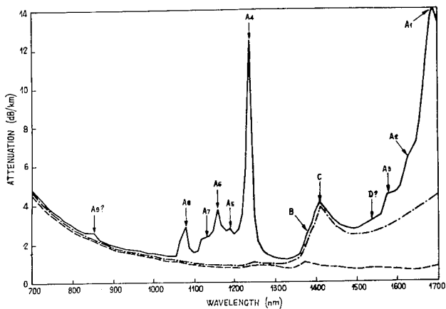
FIGURE 1 Spectral attenuation curve of a multimode fiber with 1% P_2O_5 before (---), after an absorption ( \frac{25}{} ) and a subsequent desorption (-·-·-·) period of 1260 hours at 20°C and 600 mmHg.
