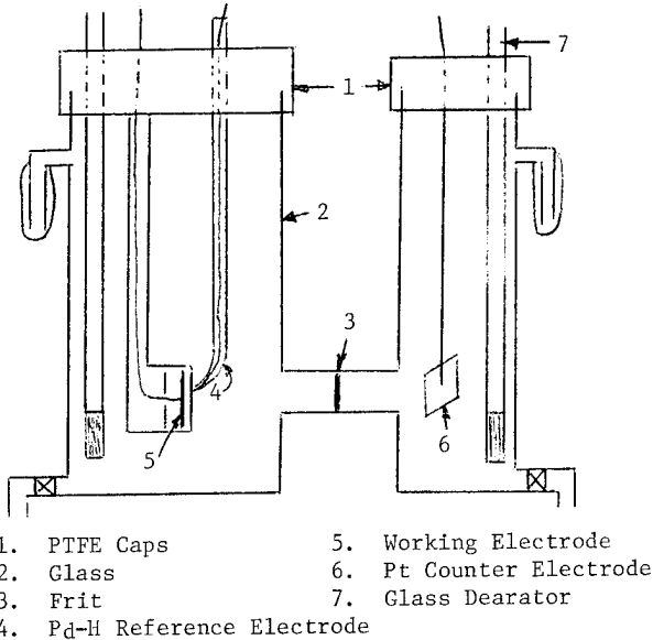
Figure 3. Electrochemical Cell
