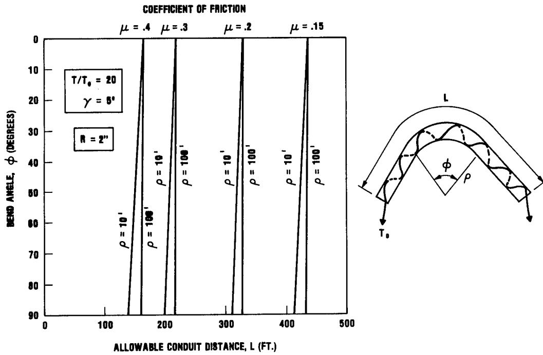
FIGURE 15 - ALLOWABLE CONDUIT LENGTH FOR CENTRAL BEND, T/T_0 = 20 , \gamma = 5^\circ
