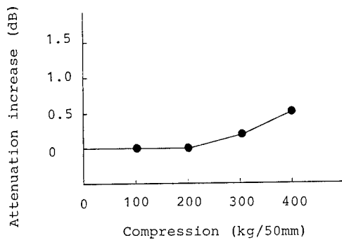
Fig. 8 Compression test
