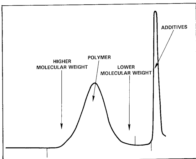
Figure 10 Sample Chromatogram of PVC Insulation (Columns — 10 6 , 10 4 , 500 A° Ultrastyrigel ® )
