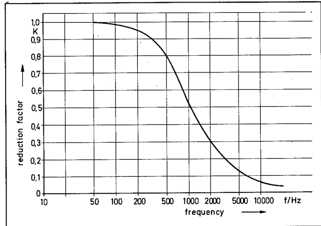
Fig. 19: Reduction Factor of LAN Unit
