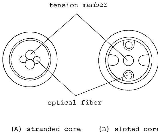
Fig. 1 Existing cables
