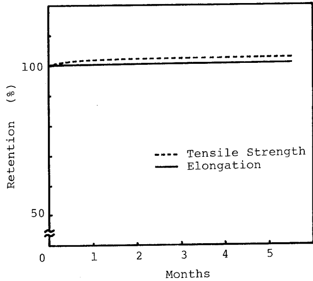
Figure 3 Immersion in Water at 50°C
