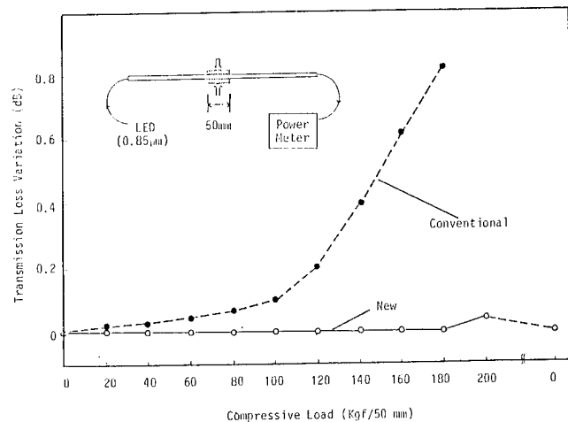
Figure 3 Compression Property
