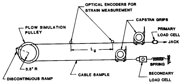
FIGURE 7. PLOW SIMULATION TEST
