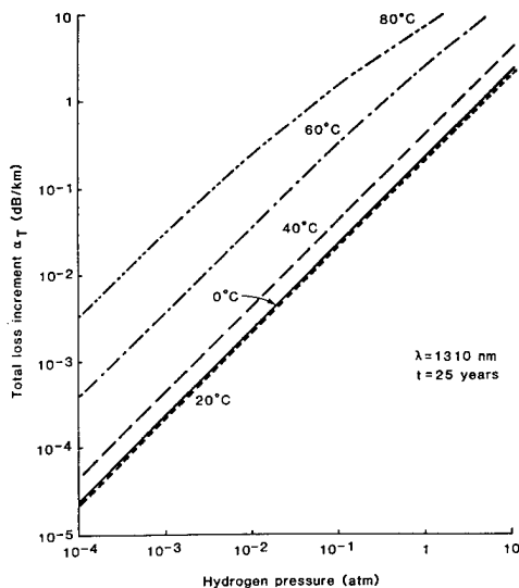
Fig. 1 Total Loss Increment as a Function of Hydrogen Pressure
