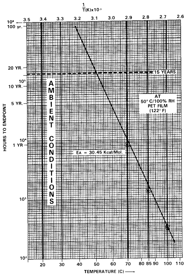
Figure 54 Arrhenius Model of PET Film in 98 + 2% RH Environment Using 14,000 PSI Tensile Strength as End-of-life Criteria.
