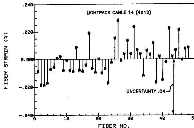
FIGURE 6. FIBER STRAIN AFTER MANDREL WRAP (4" DIA.)
