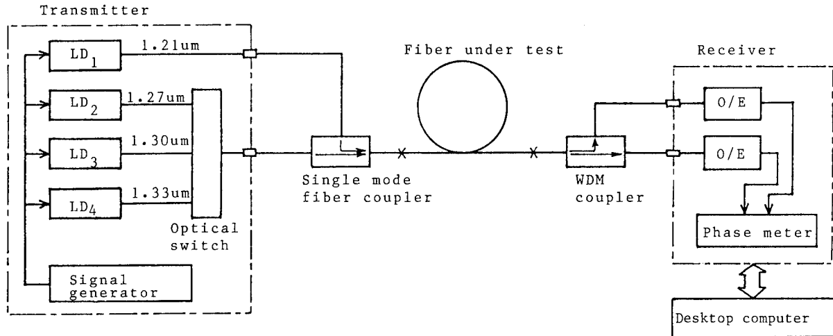
Fig. 1 Measuring system
