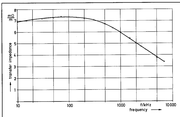
Fig. 18: Transfer Impedance of LAN Unit
