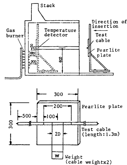
Figure 3 Equipment of fire resisting test
