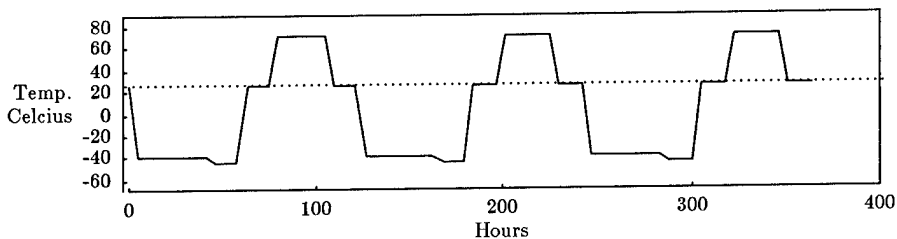
Figure 4.1a. Temperature Cycle
