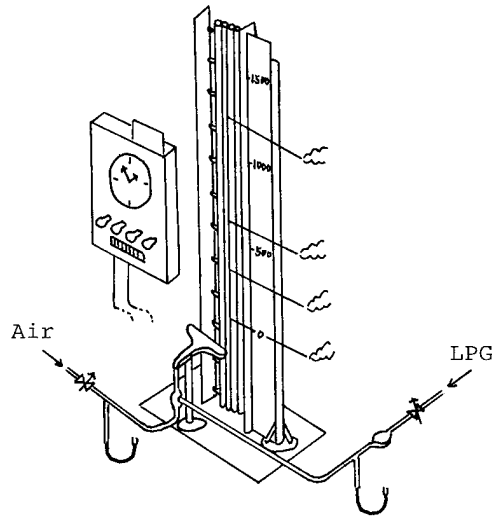
Figure 9 Arrangement of Vertical Tray Flame Test
