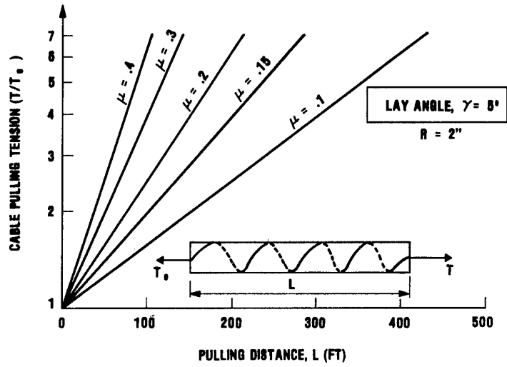
FIGURE 11 - CABLE PULLING TENSION FOR STRAIGHT HELIX SECTION, LAY ANGLE, \gamma = 5^\circ
