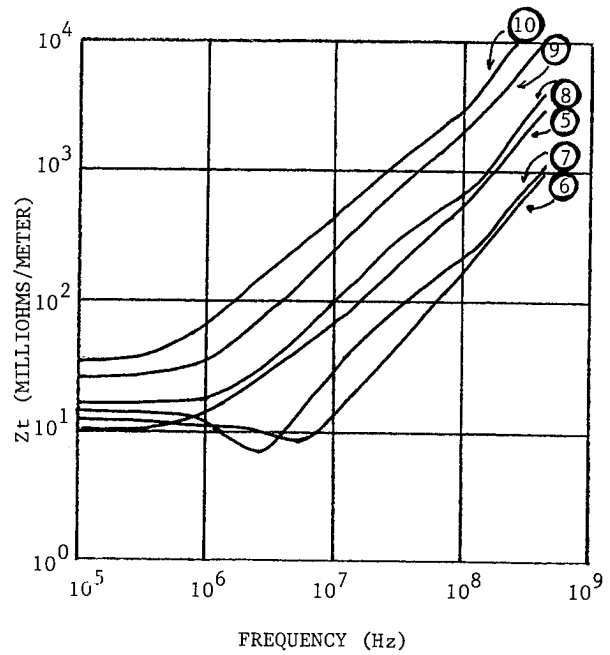
Fig. 7 - Variation in transfer impedance vs. braid coverage for \alpha = 32^\circ . (Re: Table 1)
