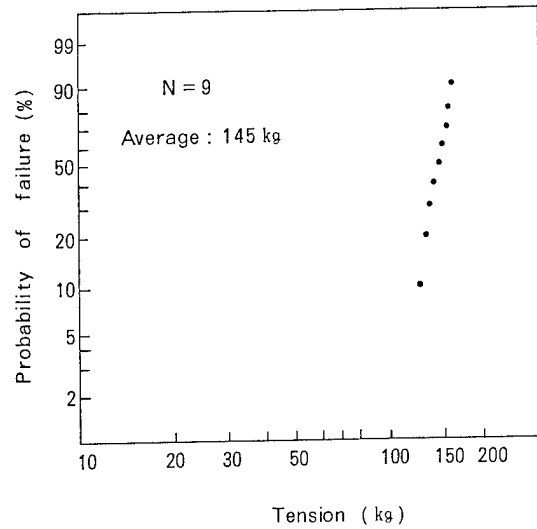
Figure 13. Tensile strength
