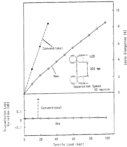
Figure 2 Tension Property
