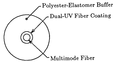
Figure 3.2. Buffered Fiber
