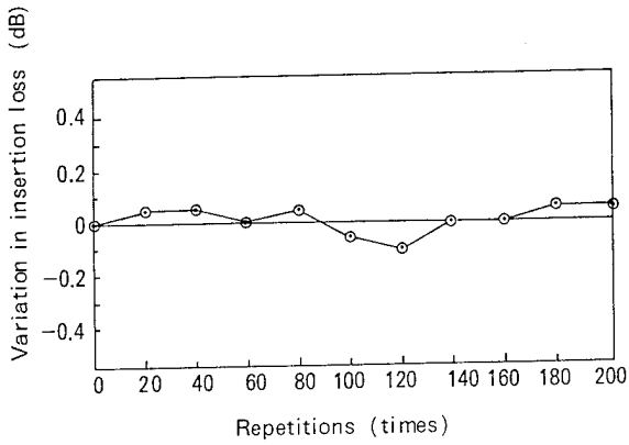
Figure 9. Repeatability test
