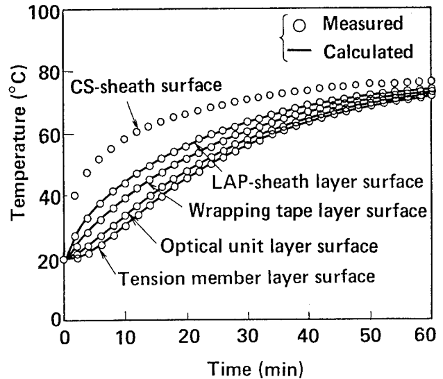
FIG.4 Temperature rise characteristics of each layer.
