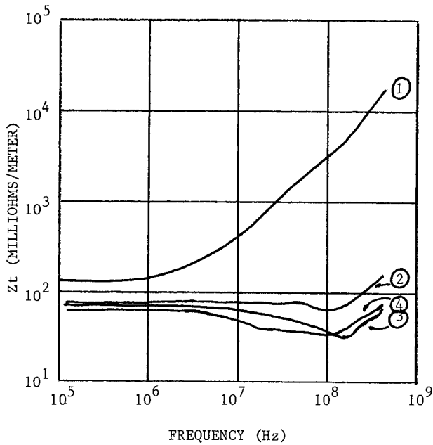
Fig. 10 - Transfer impedance vs. amount of tape overlap "s". (Re: Table 2)
