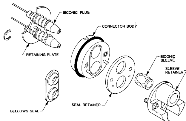
Figure 4. Connector-Insert Assembly
