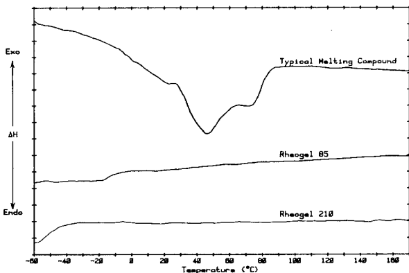
Fig. 2 DSC Thermograms
