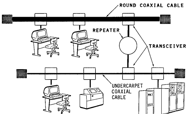
FIGURE 11 UNDERCARPET ETHERNET INTERFACE WITH STANDARD ETHERNET NETWORK
