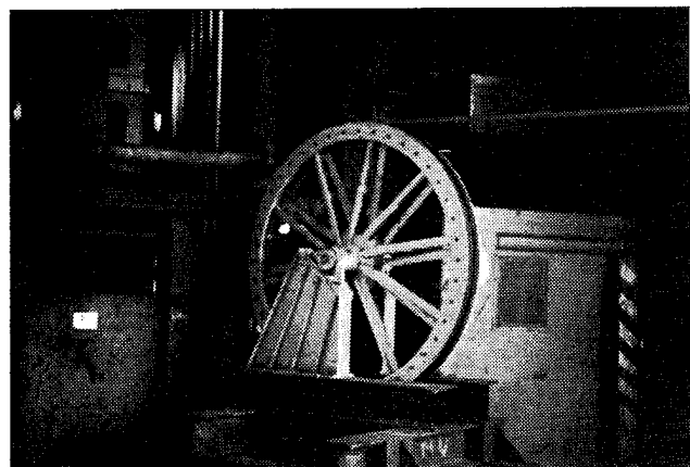
Fig 20: Shifting Wheel for Shaft Cable Installation
