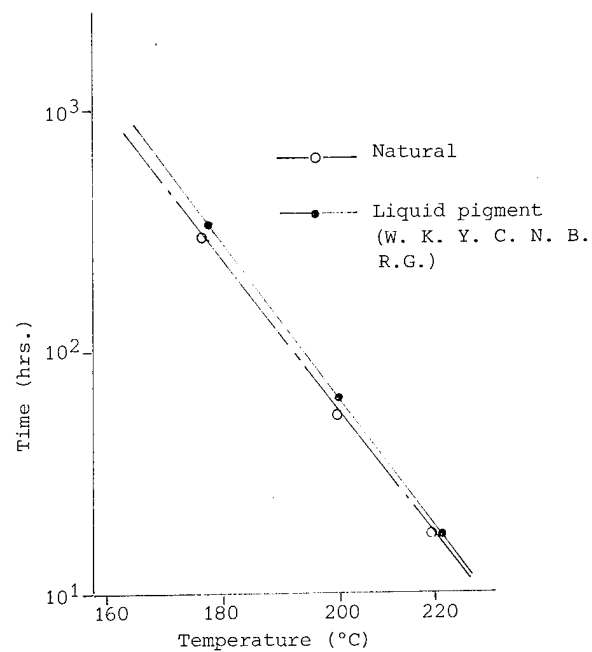
Fig. 2 Thermal Aging Property of Beamex ER* (Method: Wire wrapped around a same diameter mandrel after aging)
