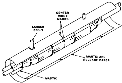
FIGURE 5. BLADDER
