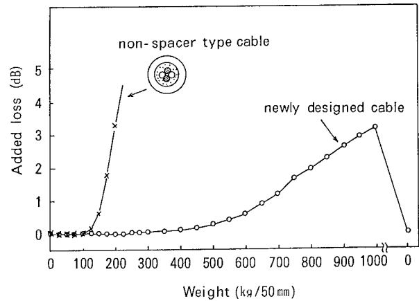
Figure 2. Compression property
