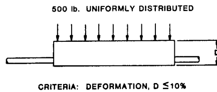
FIGURE 1d. COMPRESSION TEST
