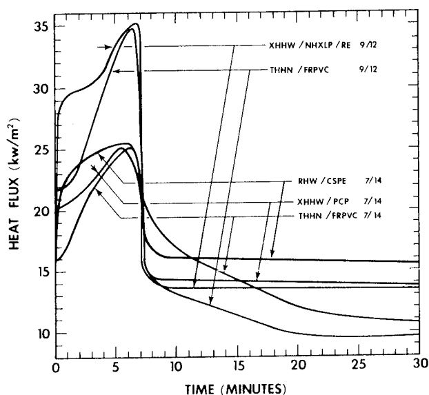
TOTAL RADIANT HEAT FLUX FROM BURNER AND CABLES
