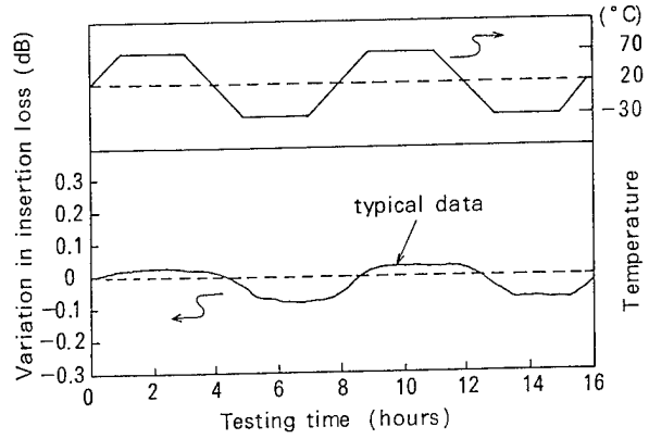
Figure 11. Thermal dependence
