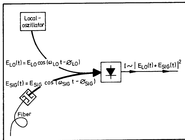
Fig. 3 Opto-electric conversion of coherent signals with photodiodes
