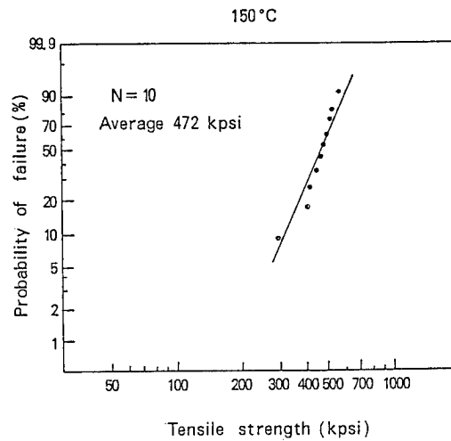
Figure 10 Tensile strength after high temperature test
