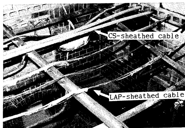
Fig.6 Photographic view of cables after heating.
