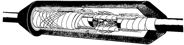
figure 7 Cross Section Of Buried Non-pressurized Splice
