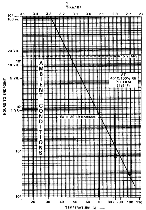
Figure 53 Arrhenius Model of PET film in 98 + 2% RH Environment Using 20% Elongation as End-of-life Criteria.
