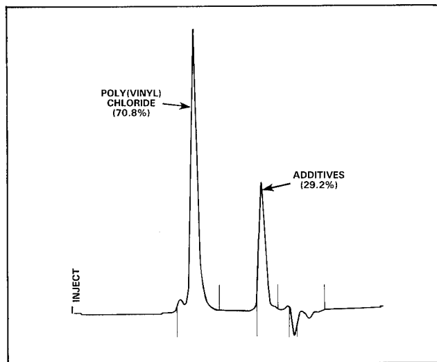
Figure 35 Sample Chromatogram for 105 C Rated PVC Insulations Exposed to 85 C/98% RH Environment
