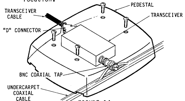
FIGURE 14 BNC MALE TAP CONNECTION METHOD
