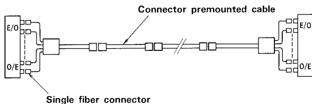
Fig.3 Application of Connector Premounted Cable
