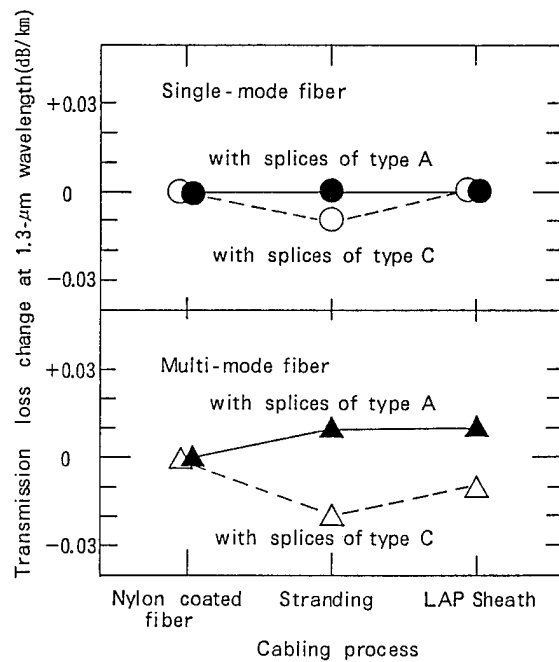
Figure 20 Transmission loss changes during cabling process for 14-fiber cable
