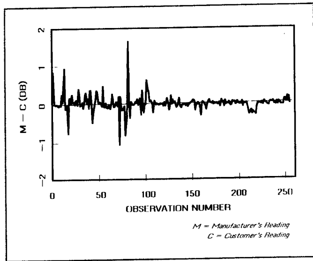
Figure 4. Differences in fiber attenuation measurements.
