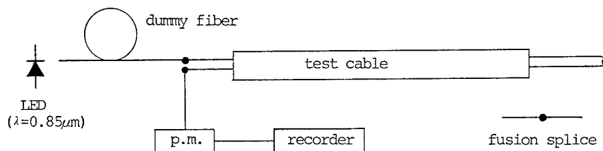
Fig. 5 Setup for measuring attenuation
