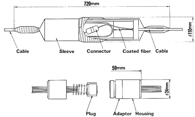
Fig.5 Construction of Sleeve Type
