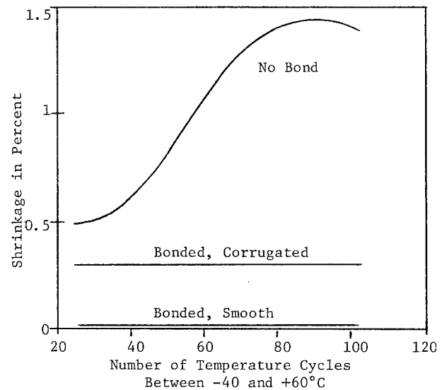
Figure 3. Effects of Thermal Cycling on Jacket Shrinkback
