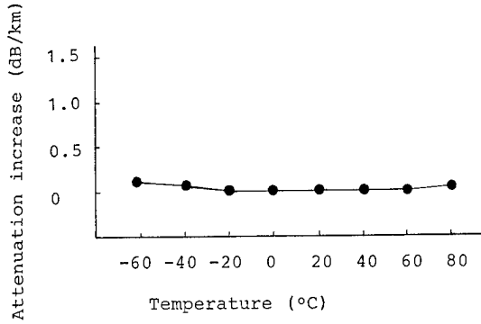
Fig. 6 Temperature characteristics
