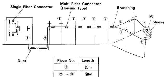
Fig.13 Installed Cables
