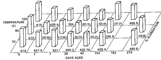
Figure 25 Change in Elongation for Solid Tubular Cross-Linked PE (22 AWG) VGM Insulation - Blue with a White Helical Stripe
