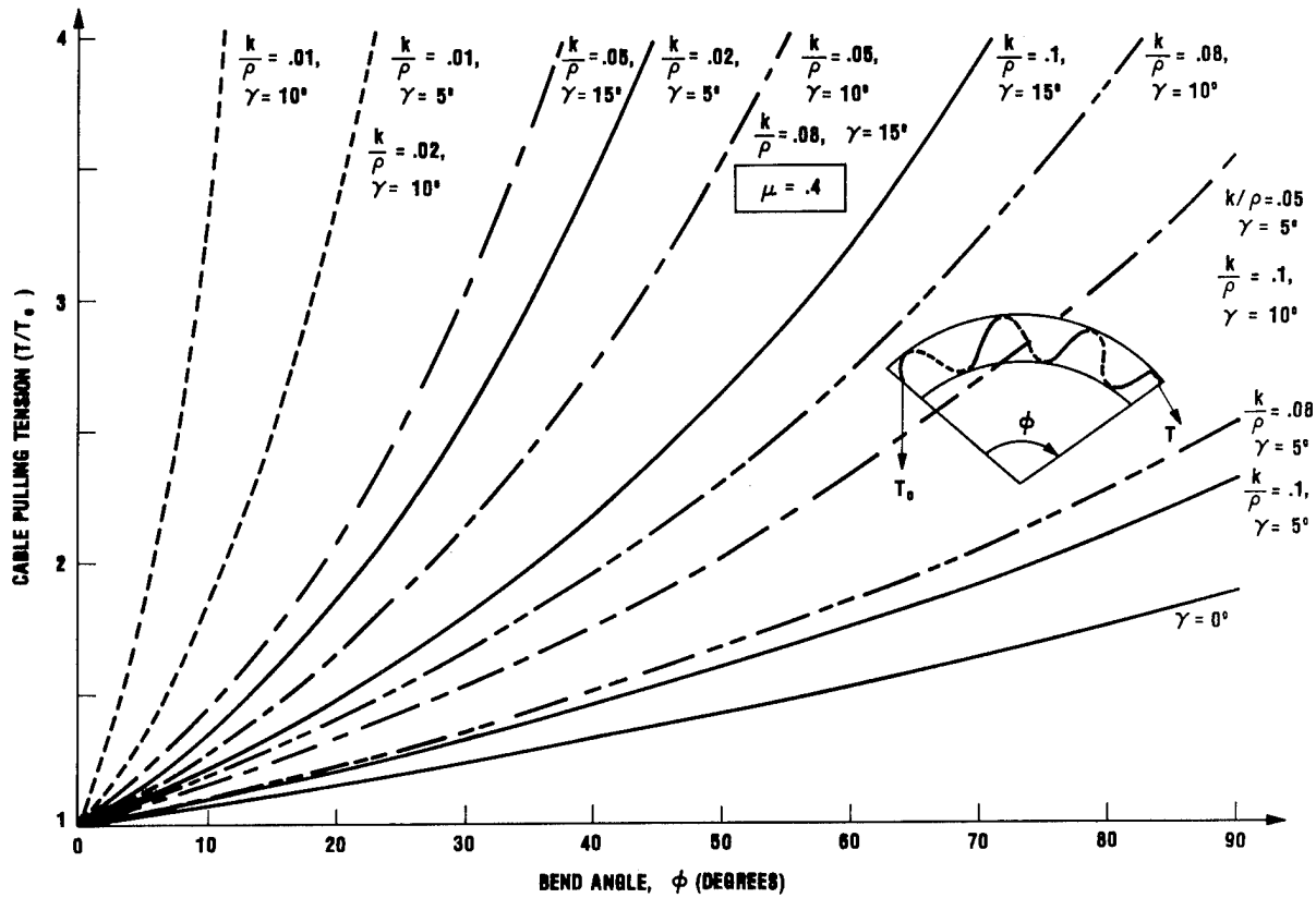
FIGURE 9 - CABLE PULLING TENSION THROUGH CURVED HELIX
