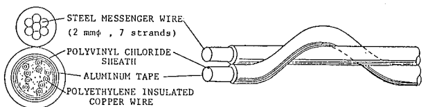
Fig. 2 Structure of copper communication cable 0.9 mm 10 pairs CPEV-SSS (Polyethylene insulated polyvinyl chloride sheathed self-supporting cable)
