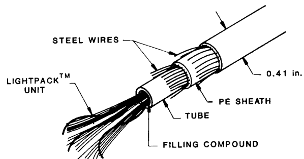
FIGURE 2. LIGHTPACK™ CABLE
