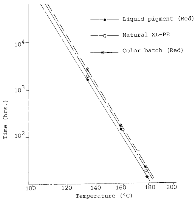
Fig. 1 Thermal Aging Property of Std. XL-PE vs. Liquid (Elongation, 50% retention)
