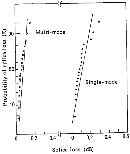
Figure 6 Splice loss of high strength splicing
