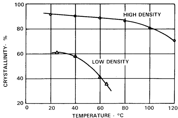
Figure 56 (43) The Effect of Heat Treatment on the Crystallinity of Polyethylene
