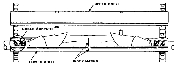
FIGURE 8. OUTER SHELL
