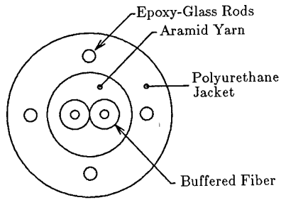
Figure 3.1. Tactical Fiber Optic Cable
