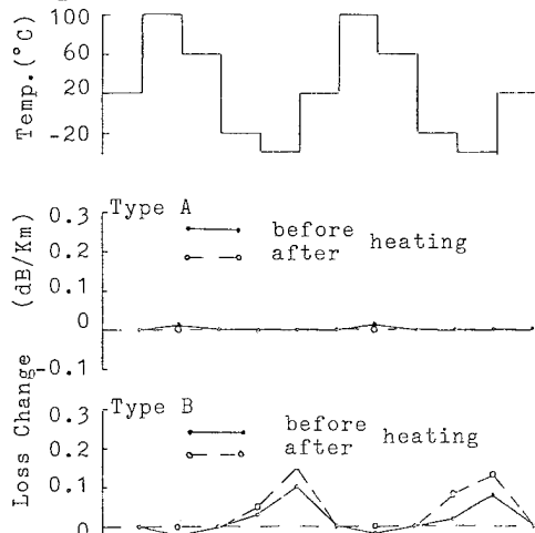
Fig. 6 Heat Cycle Test of before and after heating test
