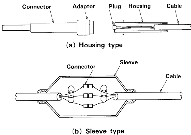
Fig.2 Fiber Connector Premounted Cable
