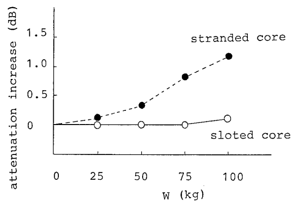
Fig. 3 Result of squeezing test
