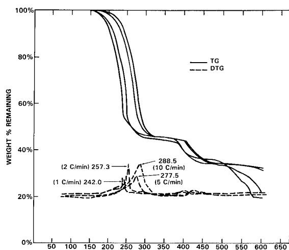
Figure 27 Thermogravimetric Analysis (TGA) of 80 C Rated PVC Jacket Insulation Aged 154 Days in 70 C/98%+ Environment
