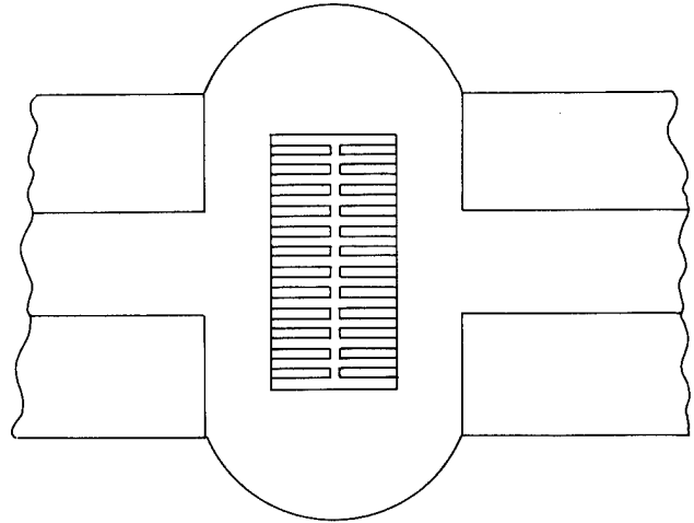
FIGURE 7. MAGNIFIED VIEW OF INDEX MATCH SLOT
