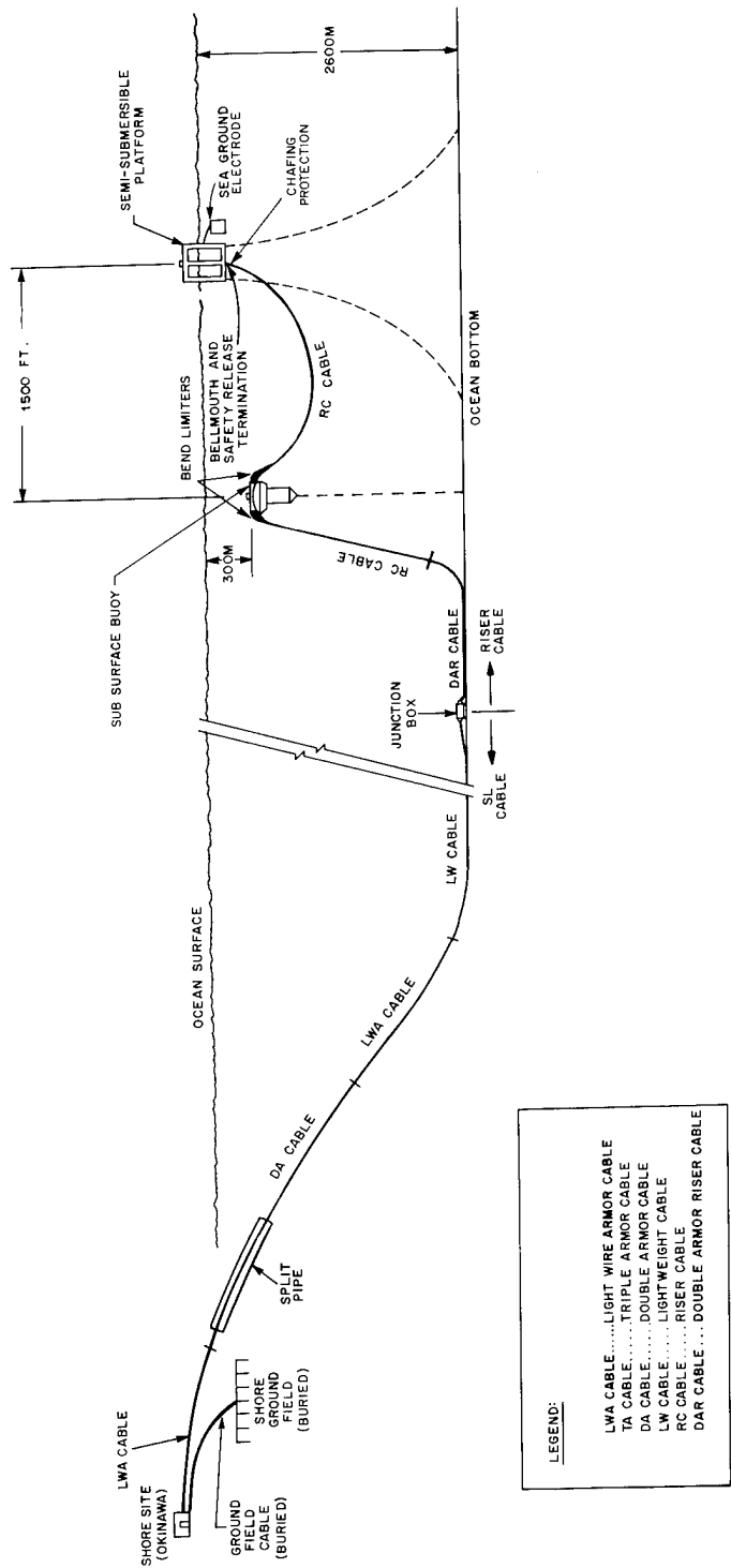
Figure 1 SYSTEM DESIGN
