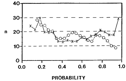
Fig. 5. Distribution of Static (o) and Dynamic (x) Fatigue Constant "n" for Spliced Fiber.
