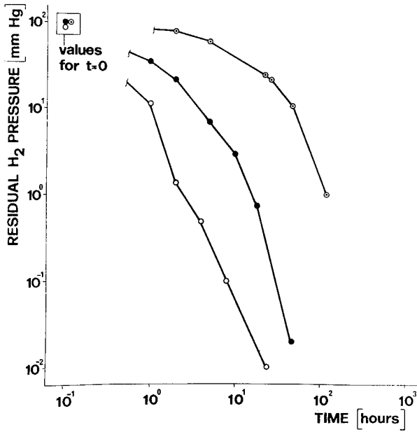
FIGURE 7 Absorption test results in shortage of hydrogen atmosphere at 0 ( ⊙ ), 25 ( ● ) and 70 ( ◐ )°C. Initial pressure 100 mmHg. An activation energy of 11 Kcal/mole can be estimated for the absorption process.
