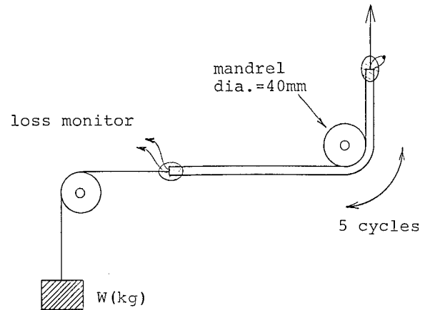
Fig. 2 Method of squeezing test
