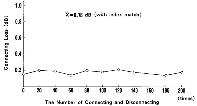
Fig.12 Result of Connecting and Disconnecting Test
