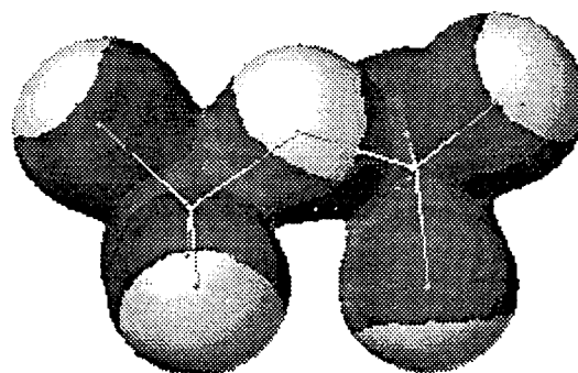
Al 2 Cl 7 - HF/6-31G* Ab Initio Density @ 0.01 e - /Å 3
