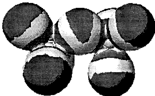
Al 2 Cl 7 - Valence Shell Density 0.01 e - /Å 3
