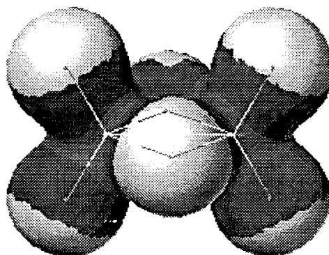
Al 2 Cl 6 HF/6-31G* Ab Initio Density @ 0.01 e - /Å 3
