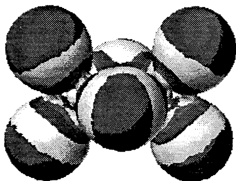
Al 2 Cl 6 Valence Shell Density 0.01 e - /Å 3
