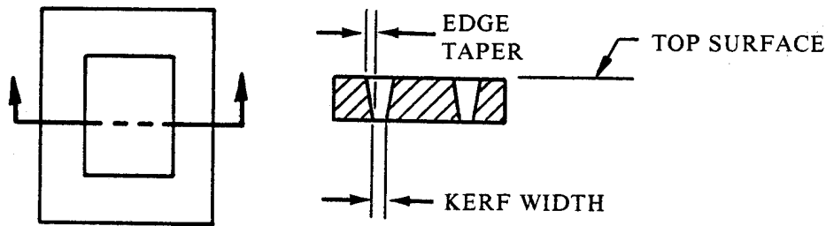
Figure 3. Kerf Width and Edge Taper Definition
