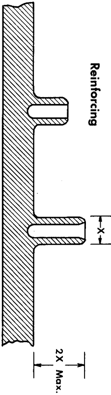
Screw Holding
