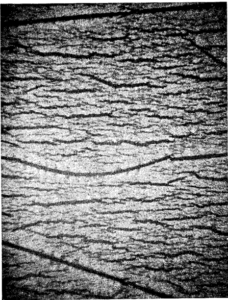
FIGURE 1: Cracks and fissures in polypropylene after 15-min. etch in hot chromic-sulfuric acid solution. (75X, dark field)
