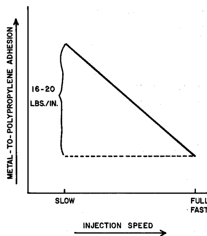
FIGURE 4: Effect of injection speed on the metal-to-plastic adhesion of electroplating grade polypropylene.
