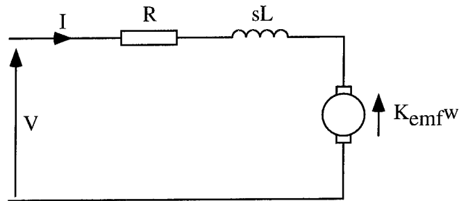
Figure 5-18: Motor model
