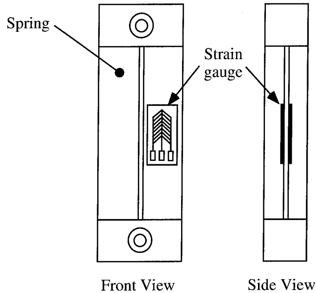
Figure 5-12: Showing position of gauges on the spring
