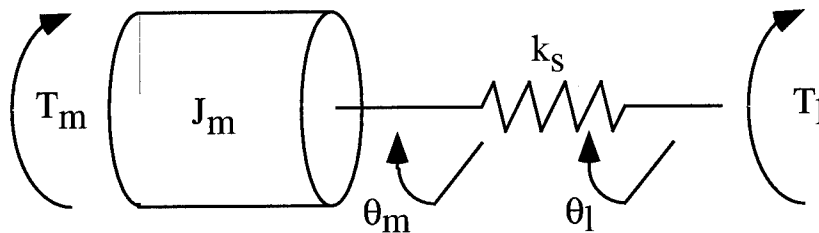
Figure 3-1: Model of actuator
