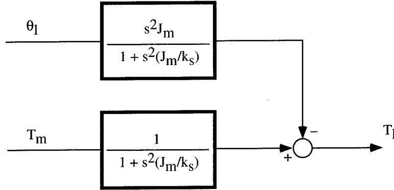
Figure 3-2: Plant model
