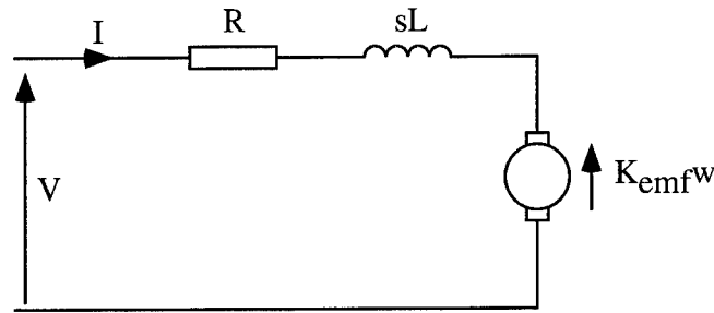
Figure 4-8: Motor model
