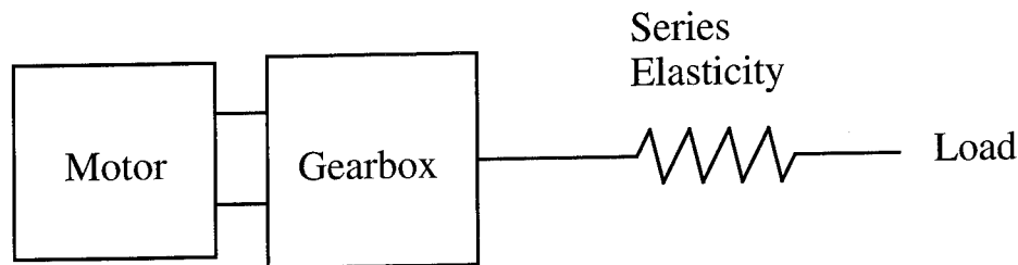
Figure 1-1: Schematic of Series-Elastic Actuator
