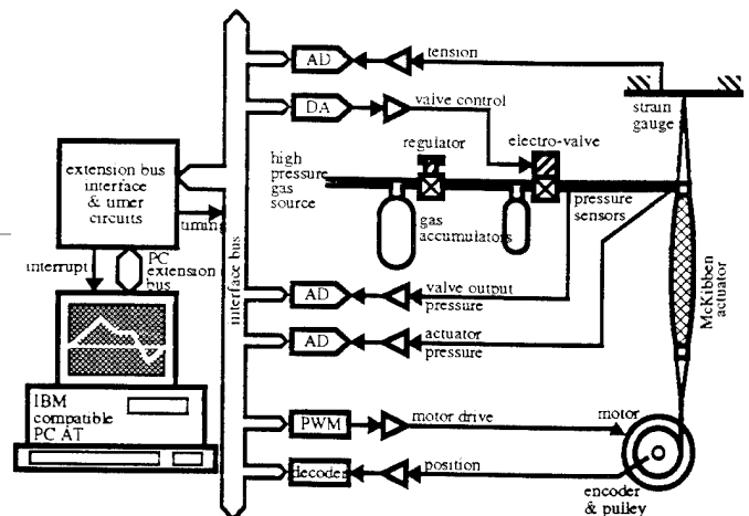
Fig. 2 Block diagram of the dynamic testing machine.
