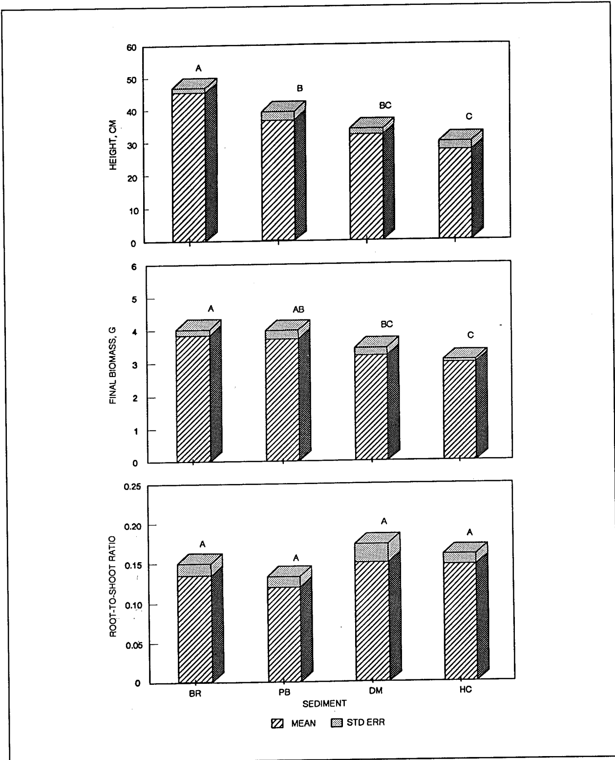
Figure 6. Plant height (uppermost frame), total biomass (middle frame), and root-to-shoot ratios (lowermost frame) in Hydrilla grown on sediments from Browns's Lake (BR), and on sediments from three unvegetated sites, Pohick Bay (PB), DM-4R (DM), and Hunting Creek (HC), in the Potomac River. Values are means and standard errors based on six replicate determinations. Within each frame, bars sharing the same letter do not differ significantly from each other. Duncan's Multiple Range Test was used to determine statistical significance at p < 0.05
