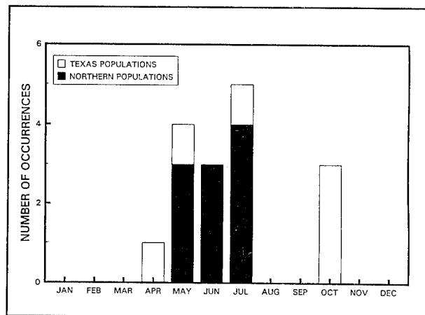
Figure 1. Frequency distribution of weak point timing by month of the year for Eurasian watermilfoil populations in northern areas and in Texas. Data from Table 1
