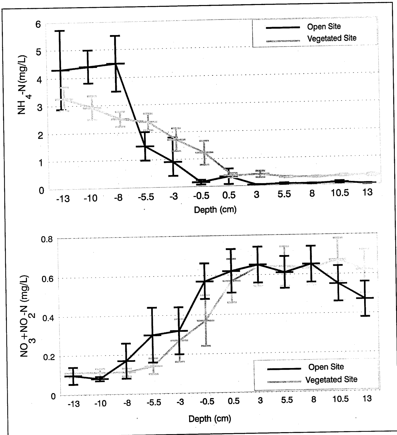
Figure 2. Seasonal means of \text{NH}_4\text{-N} and \text{NO}_3\text{+NO}_2\text{-N} concentrations in pore water, collected from peeper chambers in Lake Onalaska, 1994. Depths relate to location of the chambers in centimeters above or below the sediment-water interface. Means and standard errors are based on six to nine determinations at each depth
