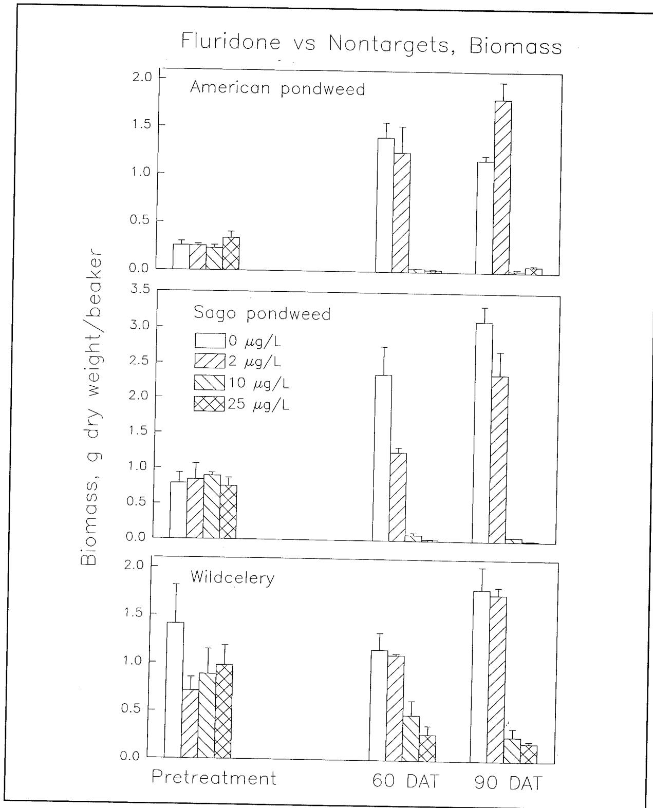
Figure 2. Pretreatment, 60, and 90 DAT biomass (one planting beaker) for three nontarget species treated with fluridone at 2, 10, and 25 µg ai/L for 90 days, or untreated. Bars represent the standard errors of means of three replicates
