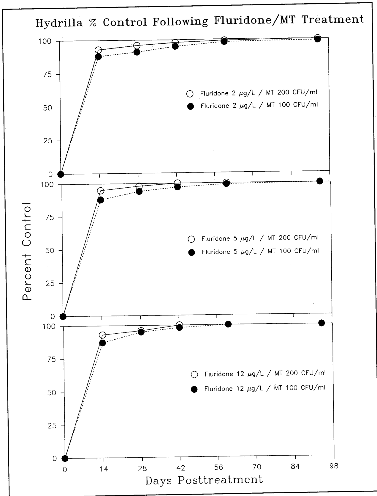
Figure 2. Percent control of hydrilla following treatment with various combinations of fluridone or Mycoleptidiscus terrestris (MT). Points at each sampling date represent the average of three replicate samples
