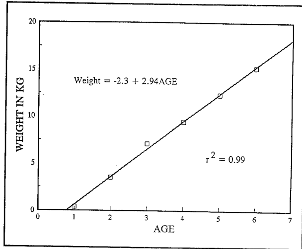
Figure 1. Growth of triploid grass carp stocked in the Santee Cooper reservoirs, South Carolina
