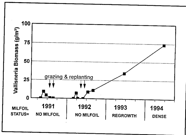
Figure 1. Mass of vallisneria within small plots at the Chisenhall Embayment on Gunter'sville Reservoir during the experiment period. Also noted is the status of Eurasian watermilfoil over the same time period
