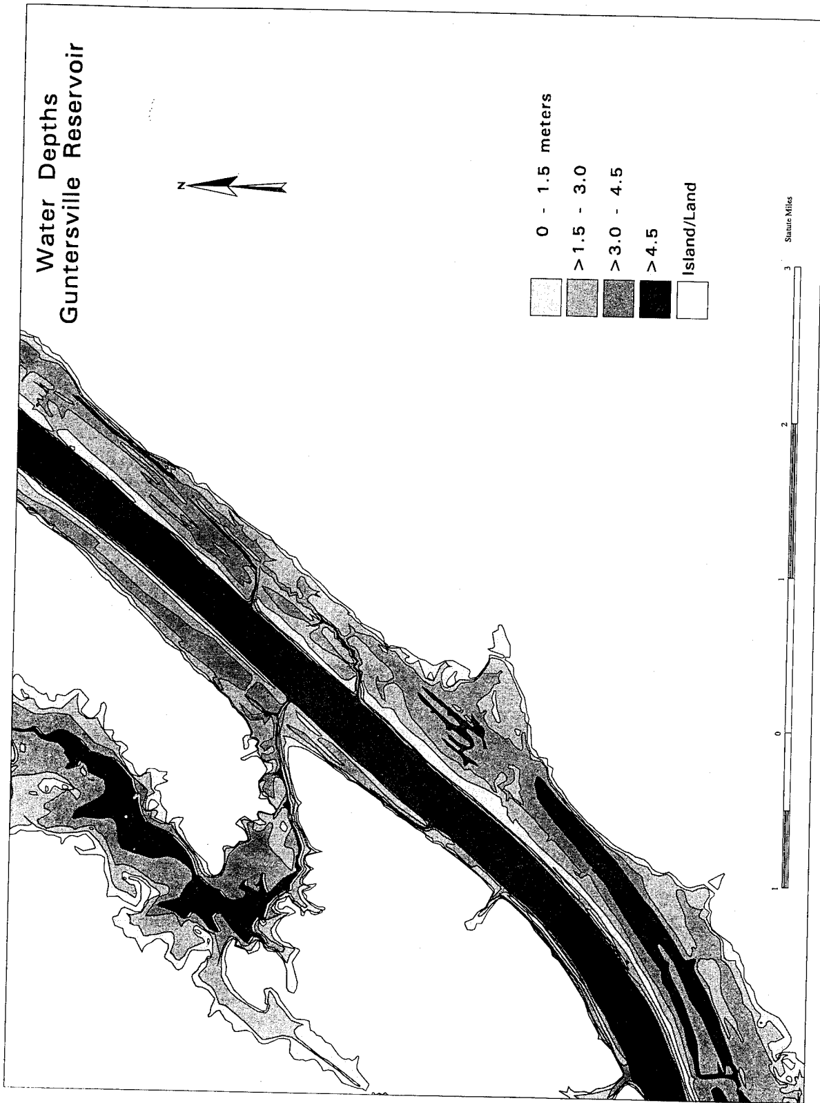
Figure 3. Lake Gunterville water depths for same area as plant distribution shown in Figure 2
