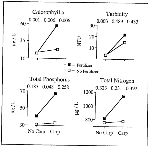
Figure 1. Mean responses of water quality variables to carp and fertilizer. ANOVA probability values are given for the main effects of carp (left), fertilizer (center), and carp x fertilizer interaction effect (right)
