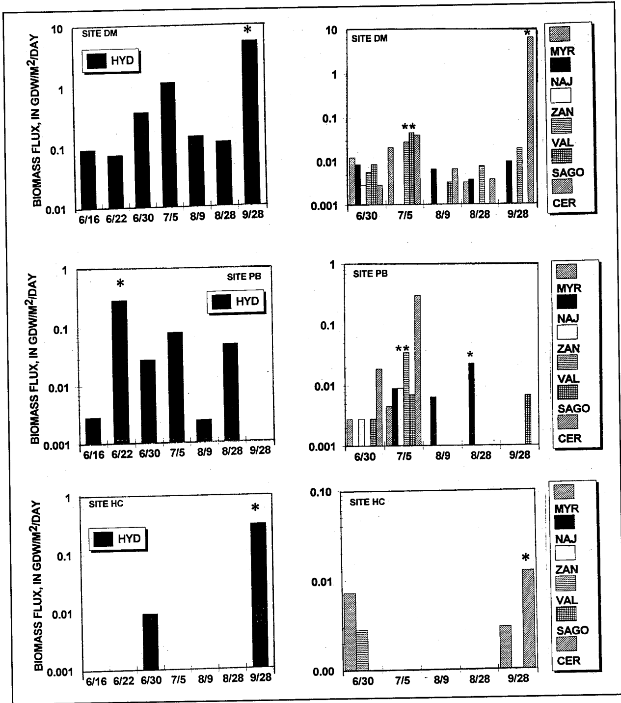
Figure 5. Species biomass flux (gdw m -2 d -1 ) by date, at unvegetated sites in the tidal Potomac River. * indicates biomass flux significantly different from that on other dates. (HYD = Hydrilla verticillata, MYR = Myriophyllum spicatum, CER = Ceratophyllum demersum, SAGO = Potamogeton pectinatus, ZAN = Zannichellia palustris, NAJ = Najas minor, VAL = Vallisneria americana)
