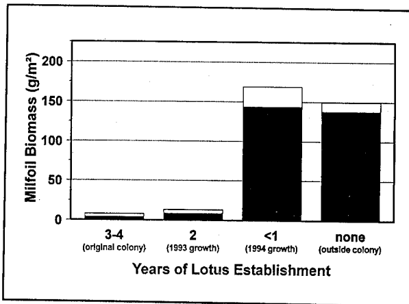
Figure 4. Eurasian watermilfoil mass in August 1994 within the various growth zones of the American lotus colony at Osa-Win-Tha cove
