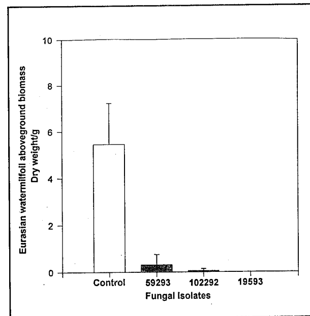
Figure 4. Mean dry weight in grams of aboveground biomass of Eurasian watermilfoil plots harvested 2 weeks post application with isolates 59293, 102292, and 19593
