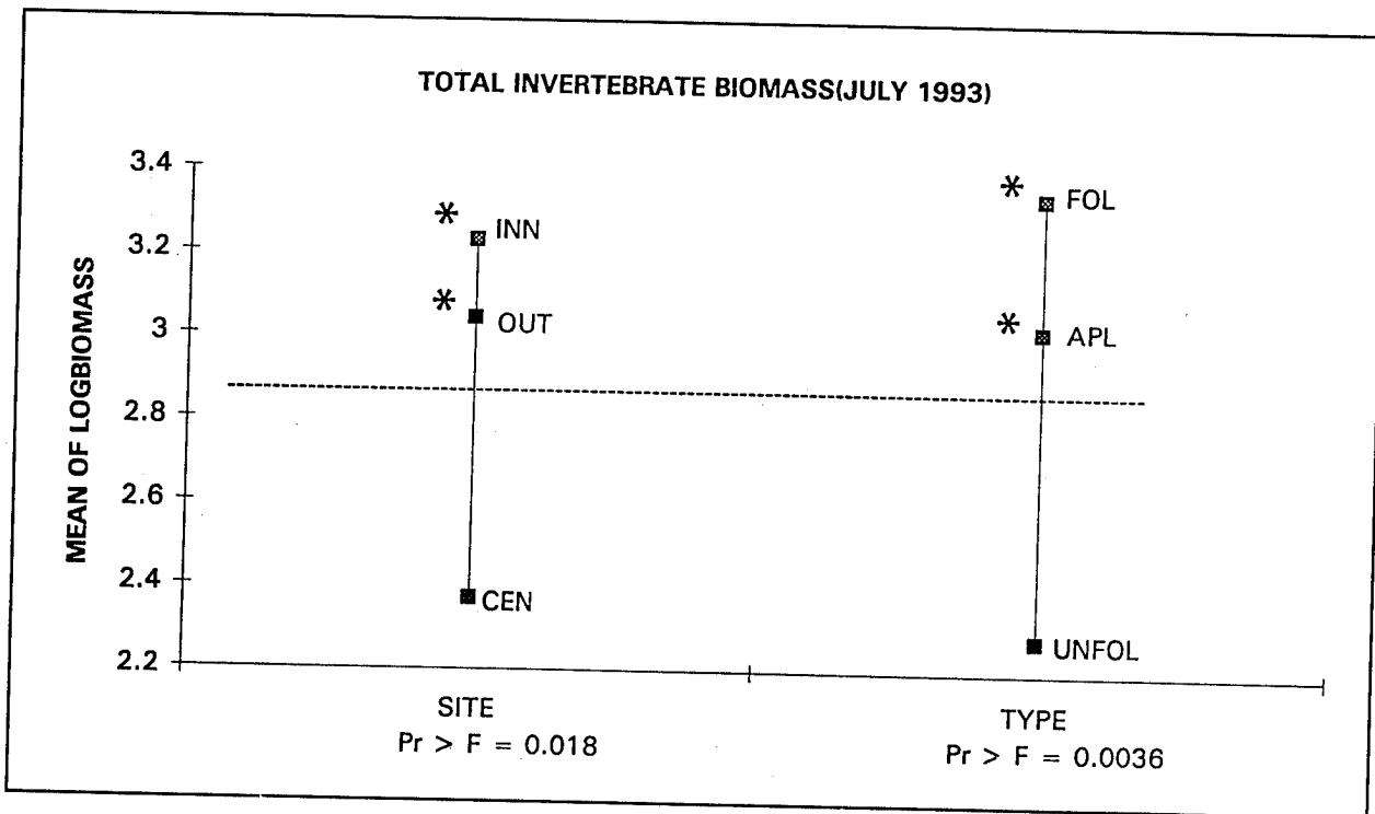
Figure 5. 1993 Fish Lake invertebrate distribution in the Eurasian watermilfoil beds by biomass, where the asterisk indicates that the mean log of the biomass is significantly higher at that site than at the lower site
