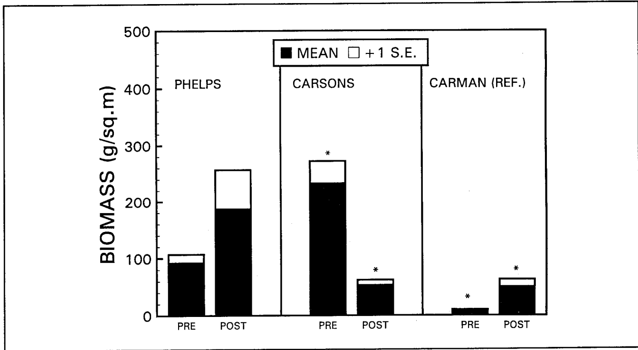
Figure 2. Biomass (g DW m -2 ) of native plants pre- (PRE) and posttreatment (POST) at the two treatment sites (PHELPS, CARSONS) and the untreated reference (CARMAN(REF)) site. Asterisks (*) indicate a significant difference between pre- and posttreatment at the p = 0.05 level using a T-test
