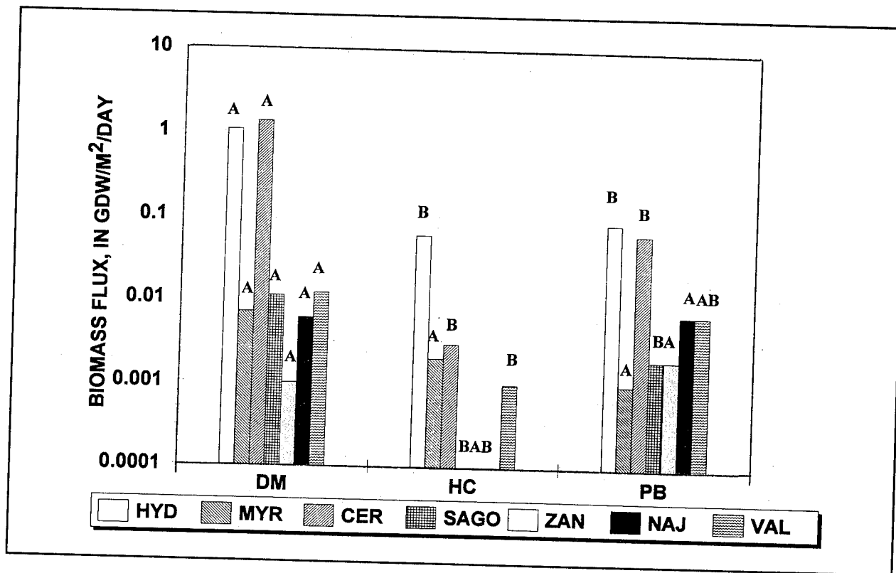
Figure 4. Mean biomass flux ( gdw\ m^{-2}\ d^{-1} ) of H. verticillata between June 16 and September 28, 1994, and mean biomass flux of all other species between June 30 and September 28, 1994, at unvegetated sites in the tidal Potomac River. (HYD = Hydrilla verticillata , MYR = Myriophyllum spicatum , CER = Ceratophyllum demersum , SAGO = Potamogeton pectinatus , ZAN = Zannichellia palustris , NAJ = Najas minor , VAL = Vallisneria americana )
