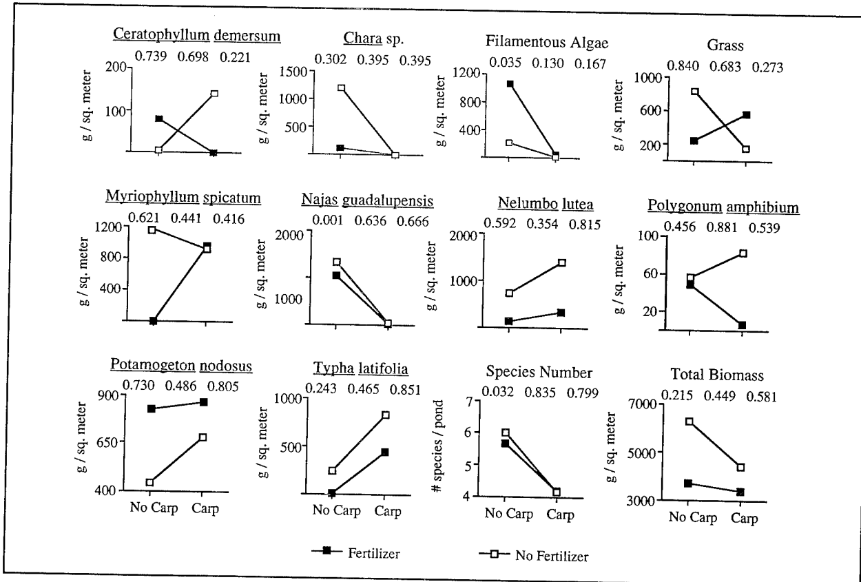
Figure 3. Mean responses of macrophytes to carp and fertilizer. ANOVA probability values are given for the main effects of carp (left), fertilizer (center), and carp x fertilizer interaction effect (right)
