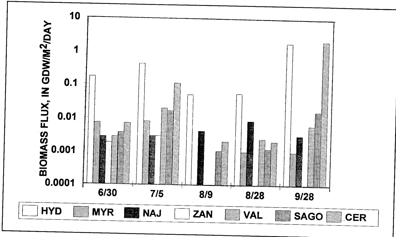
Figure 6. Species biomass flux ( gdw\ m^{-2}\ d^{-1} ) by date, for all unvegetated sites combined, in the tidal Potomac River. (HYD = Hydrilla verticillata , MYR = Myriophyllum spicatum , CER = Ceratophyllum demersum , SAGO = Potamogeton pectinatus , ZAN = Zannichellia palustris , NAJ = Najas minor , VAL = Vallisneria americana )
