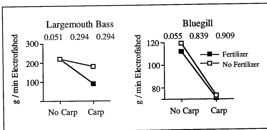
Figure 5. Mean responses of bluegill and largemouth bass to carp and fertilizer. ANOVA probability values are given for the main effects of carp (left), fertilizer (center), and carp × fertilizer interaction effect (right)
