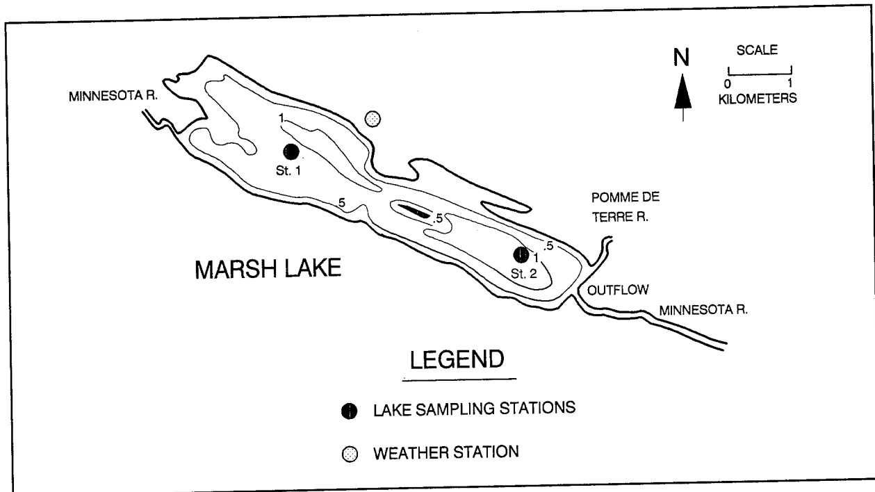
Figure 1. Morphometric map and station locations in Marsh Lake. Depth contours are in meters
