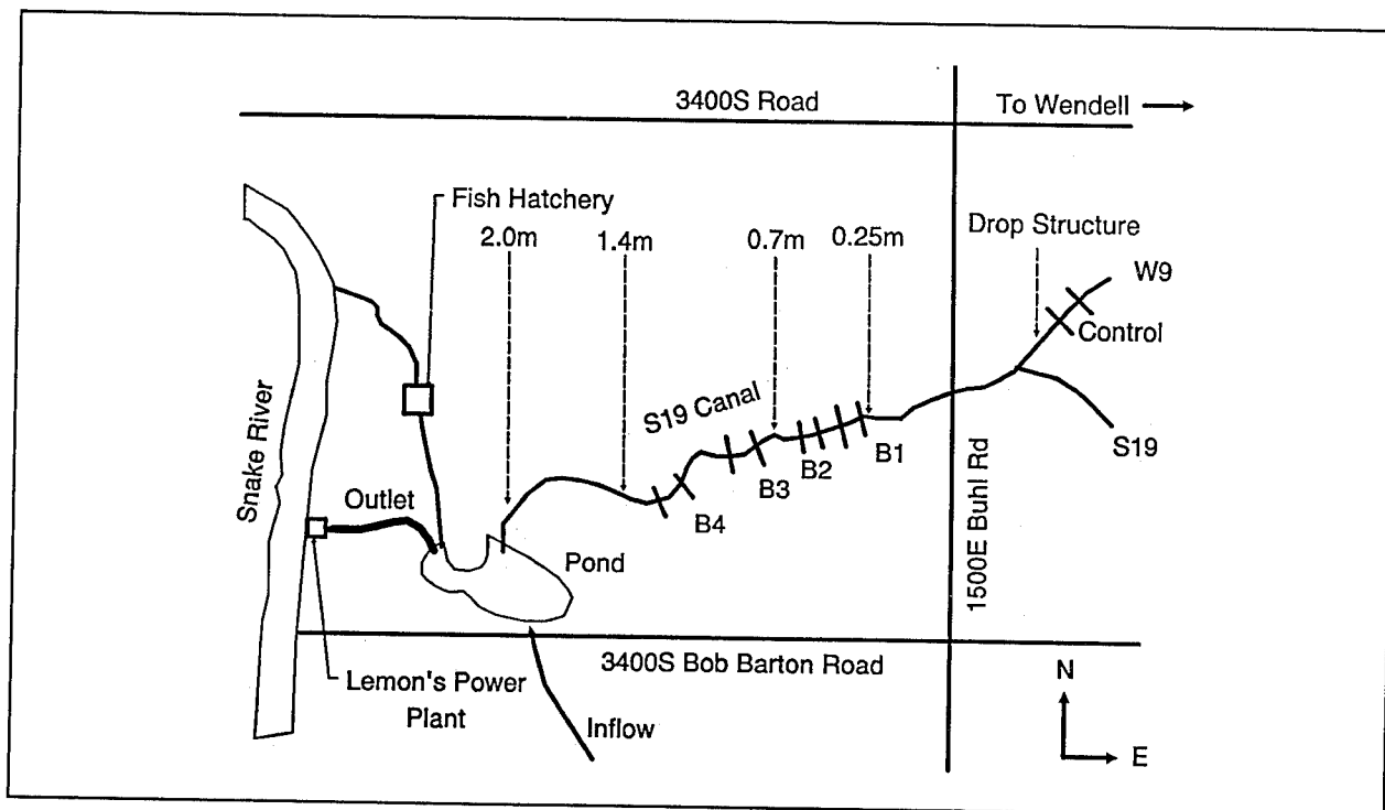
Figure 2. Location of the S19 canal showing the location of sampling stations at 0.25, 0.7, 1.4, and 2.0 miles from the drop structure where endotshall was metered in. Additional sampling stations included the fish hatchery and the outlet at Lemon's Power Plant
