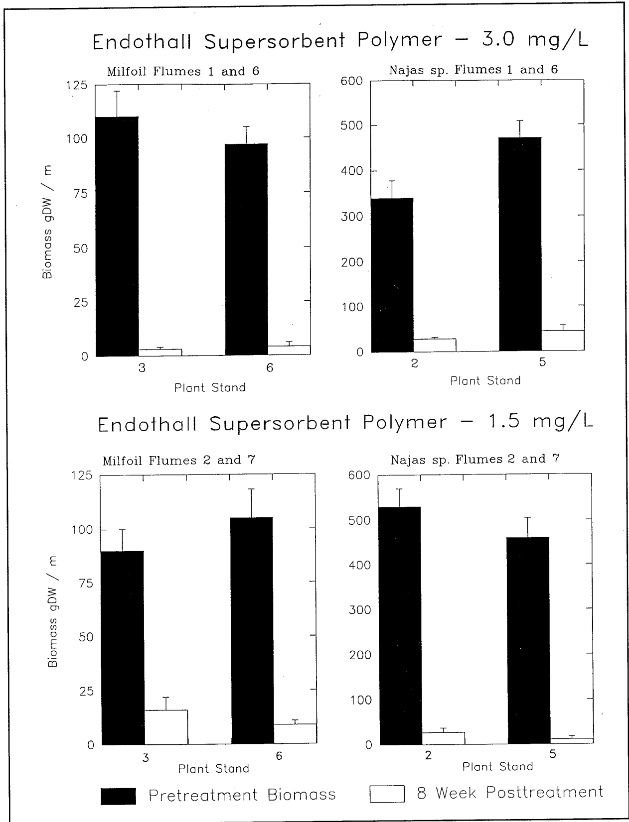
Figure 2. Endothall efficacy on Eurasian watermilfoil and Najas sp. following a 1.5- or 3.0-mg/L treatment to flowing water flumes with a supersorbent polymer formulation. Each bar represents the average of four biomass samples taken from each plant stand
