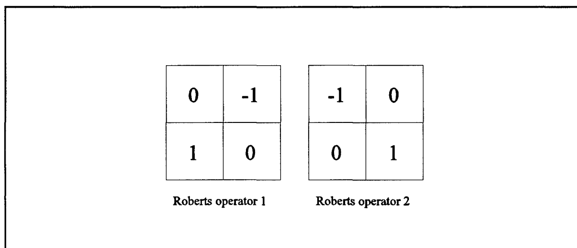
Figure 17 Roberts operators.
