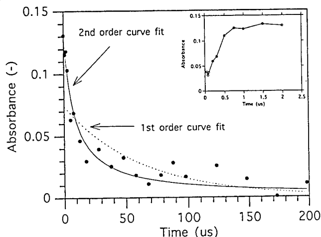
Fig. 8. Decay of the CH 3 (B ← X) absorbance in time. The dotted line is an attempt at a simple first order decay, whereas the solid curve represents a second order decay fit to the data.
