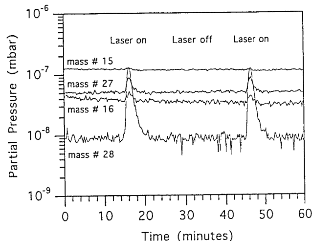
Fig. 9. Mass spectra of the by-products of the photodissociation process. Mass 15 (CH 3 ), 16 (CH 4 ), 27 (C 2 H 3 ), and 28 (C 2 H 4 ) were recorded with the ArF laser on and off. The change in concentration is greatest for mass 28, and while there is little change for mass 16, and no change for mass 15. This is a good indication that ethane (C 2 H 6 ) is the primary product rather than ethane (CH 4 ). The background concentration of the hydrocarbons is due to the dissociation of the DMZn molecule by the ionizer head of the quadrupole.
