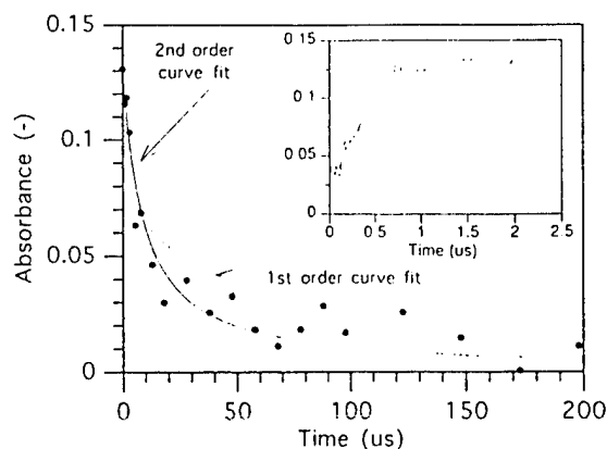
FIG. 8. Decay of the \text{CH}_3 absorbance ( B \leftarrow X transition at 2160 Å). The initial point was taken at the peak absorption, which corresponded to a time of t=2 \mu\text{s} . The inset shows the buildup of methyl radicals prior to t=2 \mu\text{s} .
