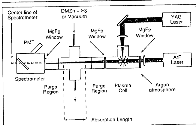
Fig. 3. Top view of the experimental layout. The experiment consists of a photodissociation laser (ArF), a laser (Nd:YAG) to create the plasma probe source, a 0.25 m spectrometer, a solar-blind PMT, a gated boxcar integrator, a timing control generator, an oscilloscope, and a microcomputer. The source gases flow through the center region and hydrogen purges are used to limit unwanted metal deposition on the windows. The absorption cell and plasma cell are separated by a \text{MgF}_2 window which allows wavelengths longer than \lambda \sim 1150\text{\AA} to be transmitted. The absorption cell is operated at a typical pressure of 25 Torr of DMZn + \text{H}_2 ; the plasma cell operates at several hundred Torr of argon, and the spectrometer is kept at vacuum. The ArF laser beam is directed slightly off axis so as to prevent 193 nm radiation from entering into the spectrometer.
