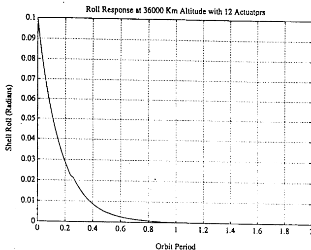
Fig. 16. Shell Roll Response
