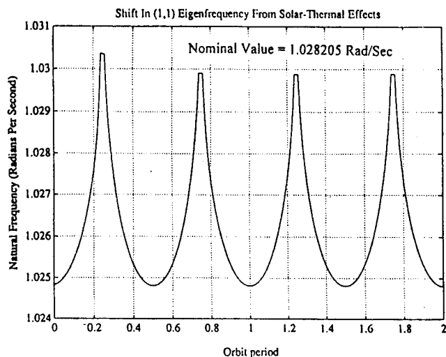
Fig. 19. Shell (1,1) Modal Frequency Vs. Orbital Time
