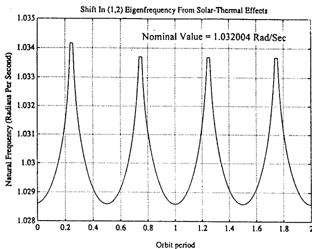
Fig. 21. Shell (1,2) Modal Frequency Vs. Orbital Time
