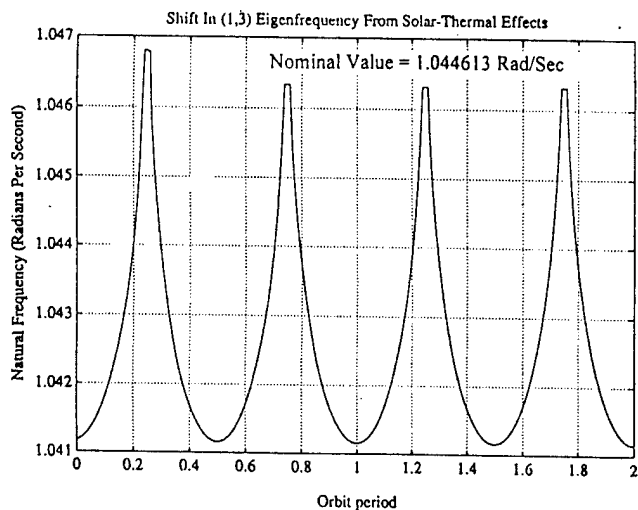
Fig. 23. Shell (1,3) Modal Frequency Vs. Orbital Time
