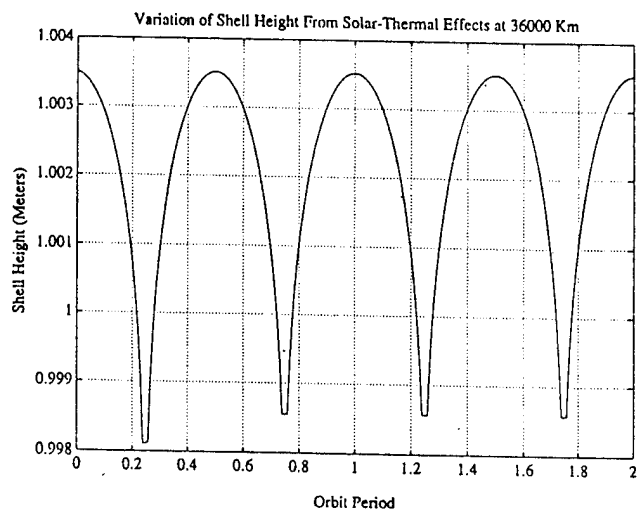
Fig. 10. Shell Height Vs. Orbital Time
