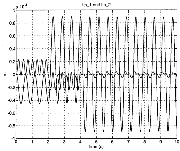
Figure 3.4: Time Histories of Tip Displacements
