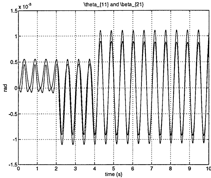
Figure 3.2: First-Order Displacements
