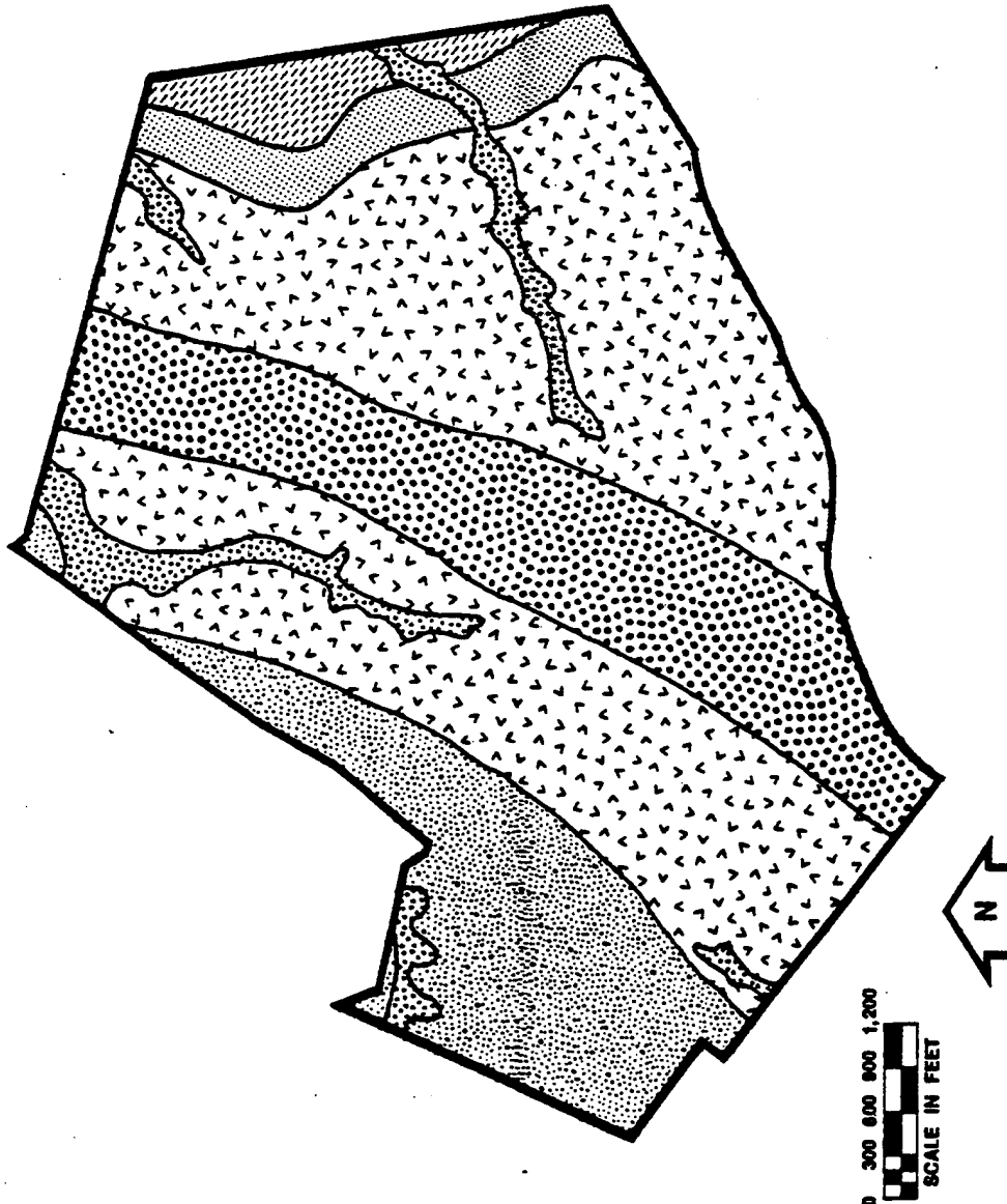
Figure 5.1-1 GEOLOGIC MAP OF VHFS BASED ON HISTORICAL DATA
