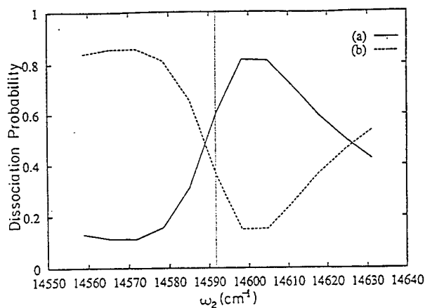
FIG. 11. As in (a) and (b) of Fig. 10, but here \omega_2 is tuned with \omega_1 = 15\,650\text{ cm}^{-1} fixed.
