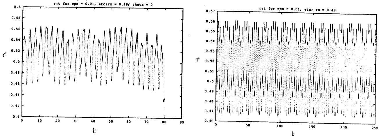
Figure 5: (a) r : t for r_o = 0.484, \theta_o = 0.0 ; (b) r : t for r_o = 0.49, \theta_o = 0.0 .
