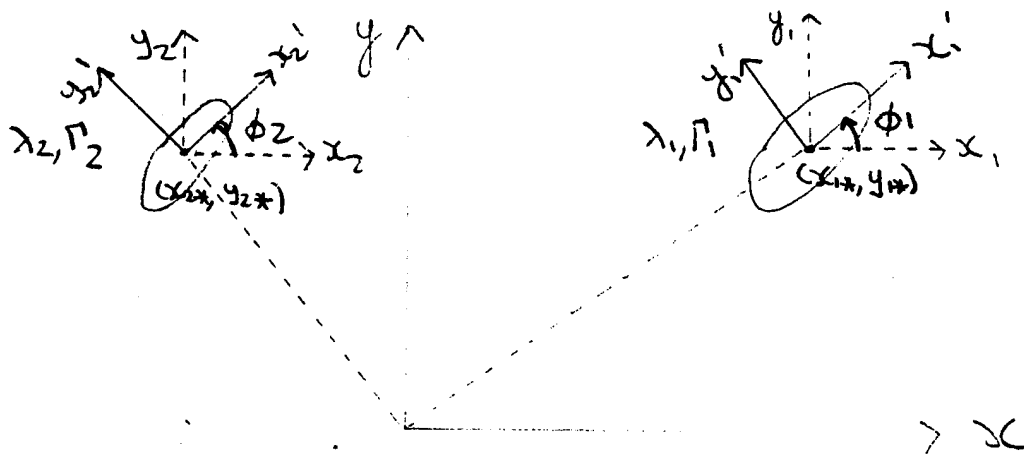
Figure 2: Configuration for the interacting Kida vortices
