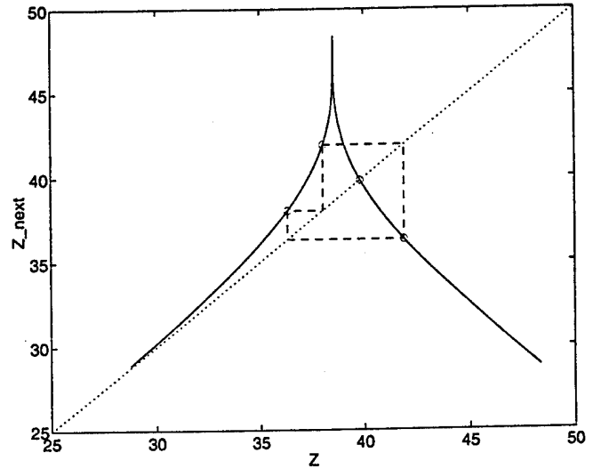
Figure 3. Map for predicting successive Z maxima at r = 28 . Two orbits are shown: the first order orbit, where the map intersects the diagonal line, and a third order orbit. These orbits are shown in figure 4.
