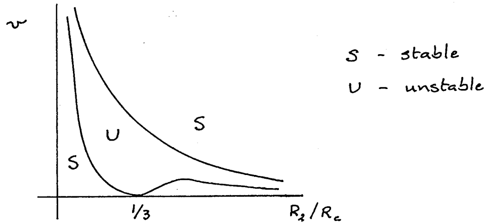
Figure 8. Stability diagram for the radial displacement.
