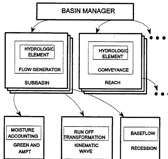
Figure 2 HEC-HMS Objects
