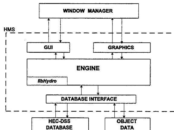
Figure 1 Software Architecture
