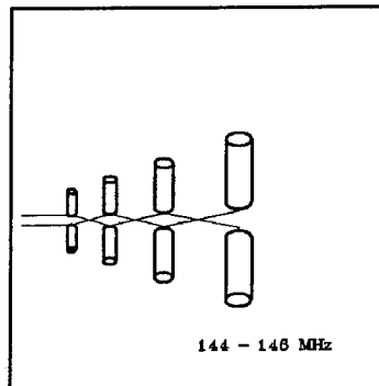
Figure 53 Choice of radio-amateurs band antenna
