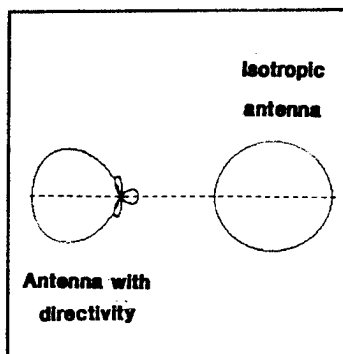
Figure 33 Antenna directivity
