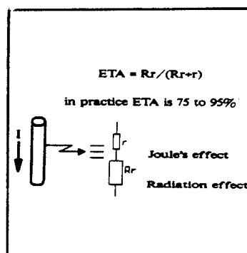
Figure 30 Efficiency of an antenna
