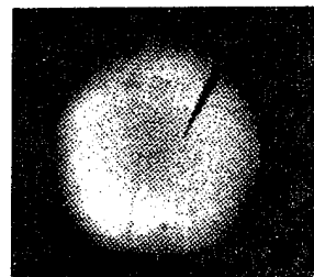
EL topography at a forward bias of 40 \text{ mA/cm}^2
