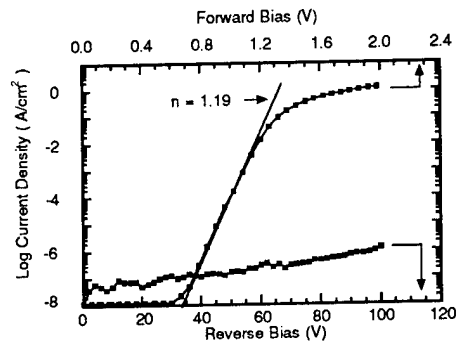
J-V characteristics of a Ni/6H-SiC diode
