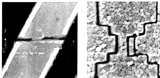
High-T c superconducting thin film microbridge
