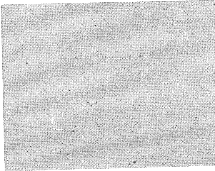
FIGURE 12. Micrograph of the as-polished transverse cross-section showing the extent of the inclusions. Mag. 100X.
