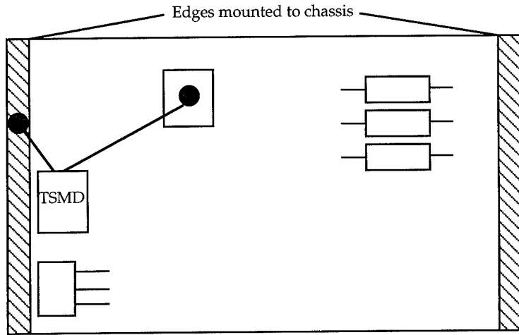
Figure 4: Micro TSMD Installation on Circuit Card
