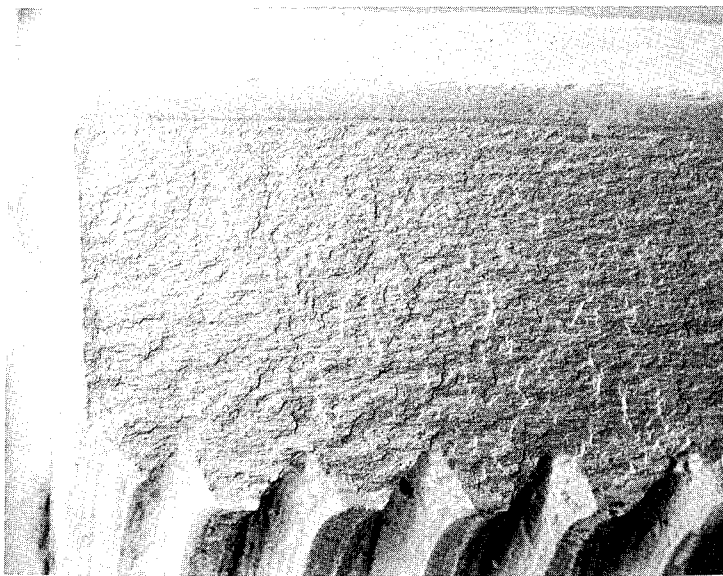
FIGURE 19. BEI fractograph showing the crack arrest marks radiating from the base of the forming seam. Mag. 12x.
