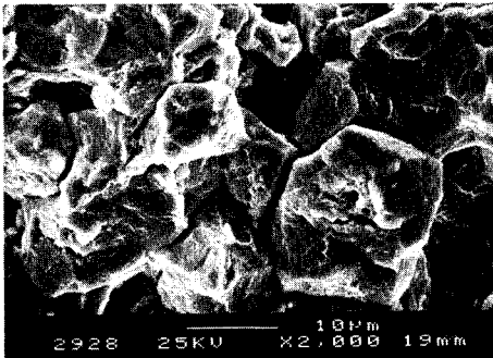
Figure 8 SEM micrograph showing part of non-corroded crack area with microcracks to be seen between grains, as well as pores, and hair lines on grain boundary surfaces
