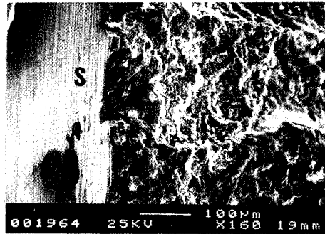
Figure 7 SEM micrograph showing preinduced crack area covered with corrosion products S = surface
