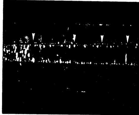
Figure 5 3:1 Dye penetrant indications in axle longitudinal direction around the preinduced crack; Cr-layer removed below the arrows
