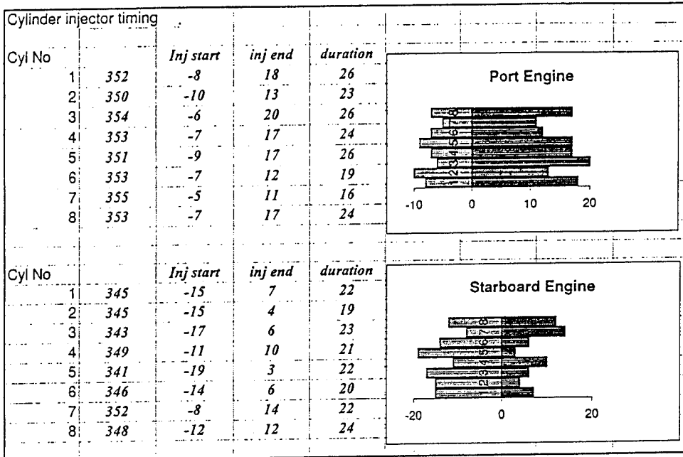
FIGURE 3 INJECTOR TIMING
