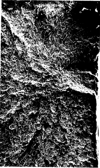
FIGURE 17 SEM fractograph showing the fracture origin and radial marks. Mag. 50x.
